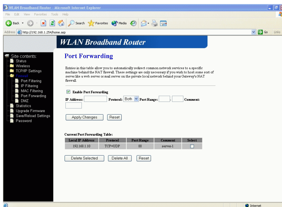
Screen snapshot – Firewall - Port Forwarding
