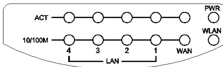
Figure 1 –WLAN Broadband Router Front Panel
