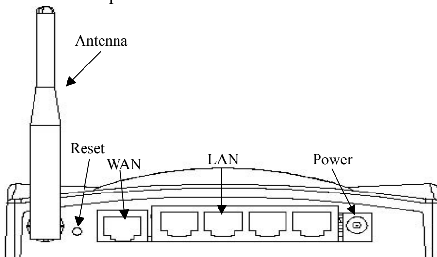
Figure 2 – WLAN Broadband Router Rear Panel
