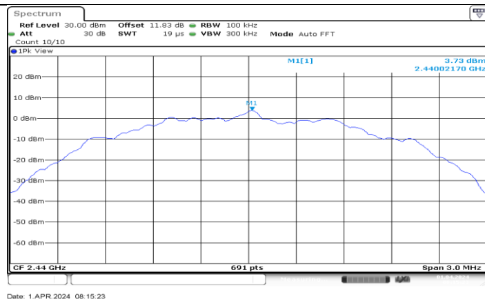
LE 2M_Ant1_2440_0~Reference
