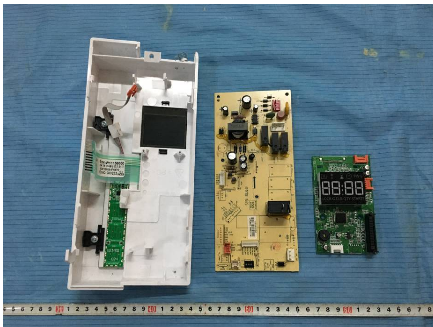
EUT – Touch Panel Cover off View
