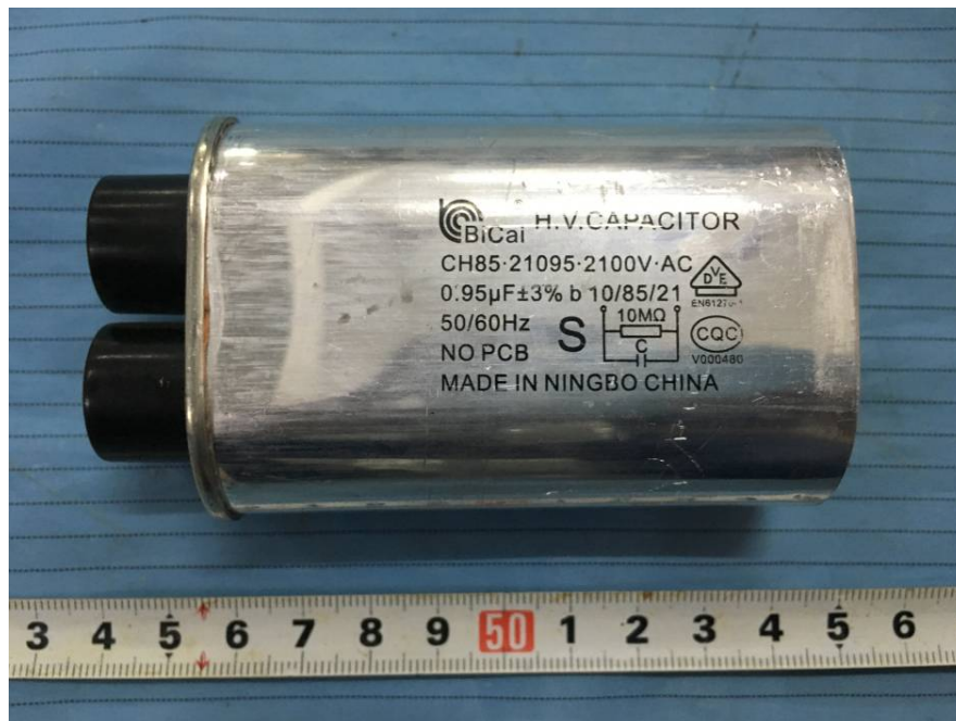
EUT – H.V. Capacitor Top View
