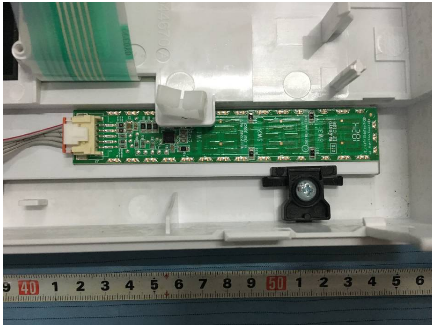
EUT – Key Board View
