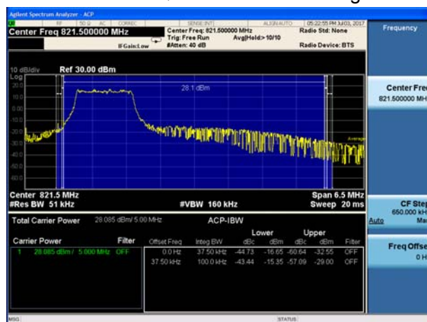
LTE Band 26 QPSK 100%RB CH High 5M
