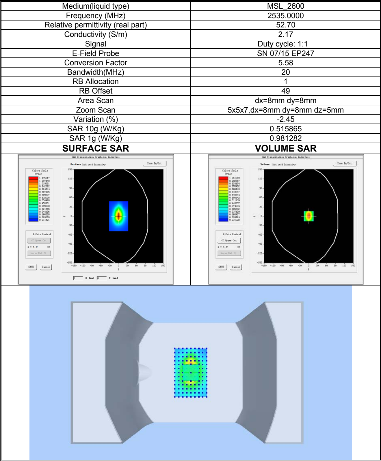
Plot 26:LTE BAND7, Middle channel (/Hotspot, Bottom edge) Product Description:Smart phone Test Date: 2019-05-13
