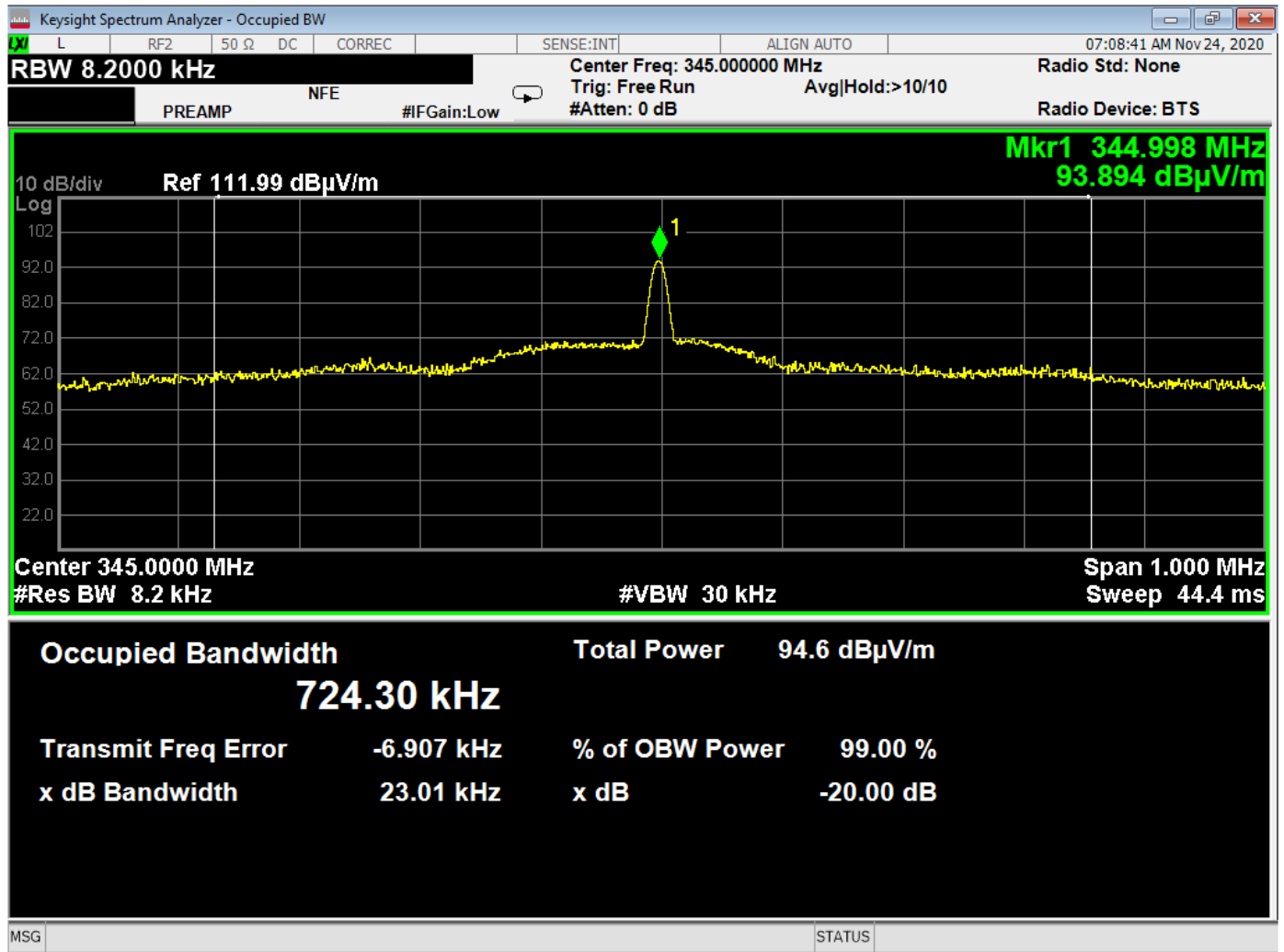
99 Percent Bandwidth Plot
