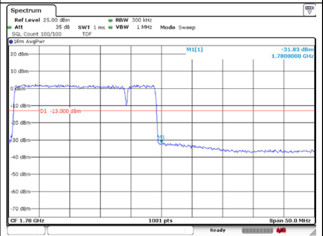
PCC 20 MHz + SCC 5 MHz_16QAM-High Channel
