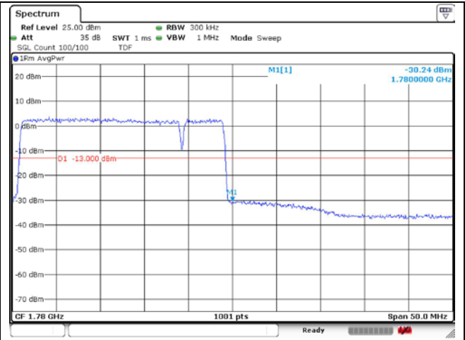
PCC 20 MHz + SCC 5 MHz_QPSK-High Channel
