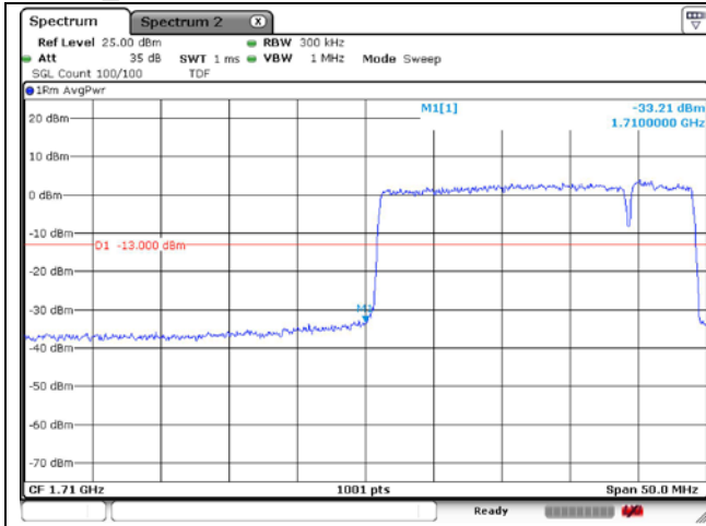
PCC 20 MHz + SCC 5 MHz_QPSK-Low Channel
