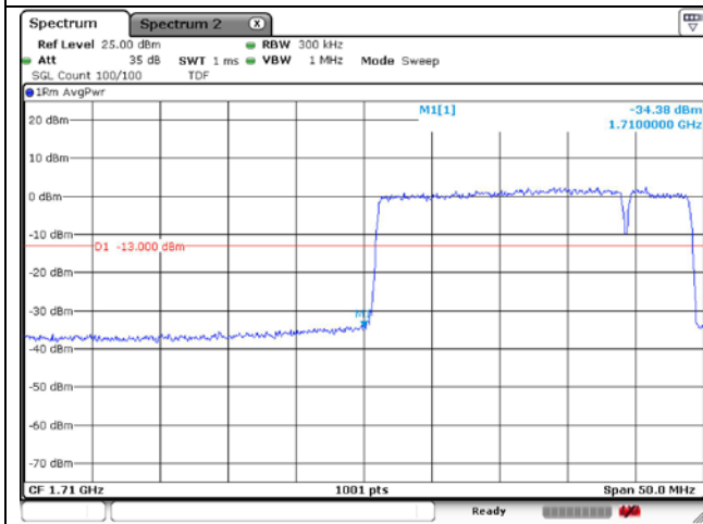
PCC 20 MHz + SCC 5 MHz_16QAM-Low Channel
