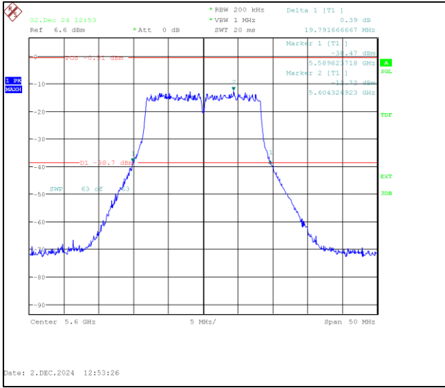
Channel Frequency:5600MHz
