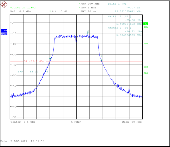
Channel Frequency:5500MHz
