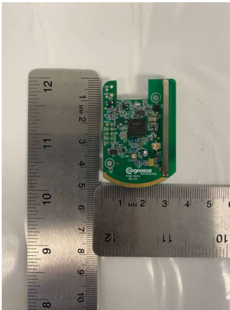
Figure 1. PCB Side 1 (see enlarged copy on page following)
