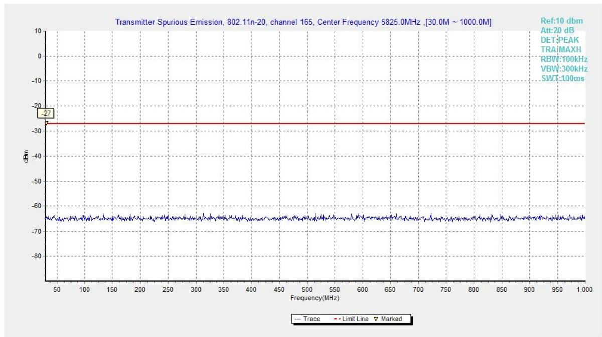
Fig. 29 Conducted Spurious Emission (802.11n20, Ch165 , 30 MHz ~ 1 GHz)
