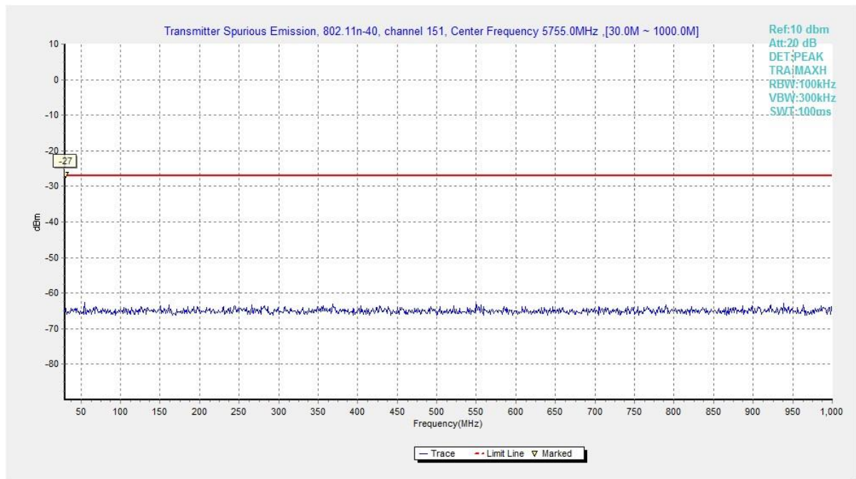
Fig. 33 Conducted Spurious Emission (802.11n40, Ch151 , 30 MHz ~ 1 GHz)
