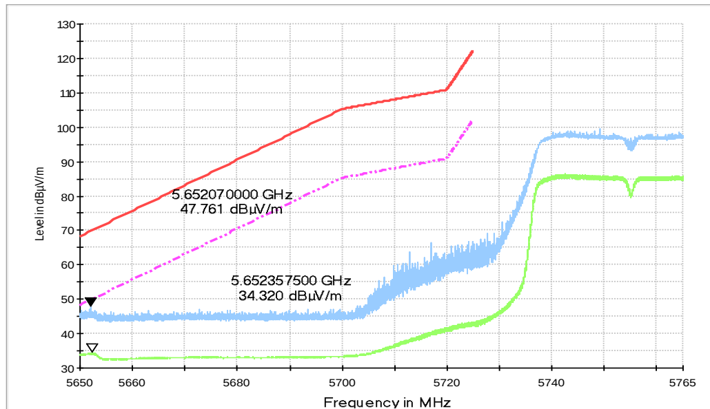
Fig. 51 Band Edges (802.11n-HT40, 5755MHz)
