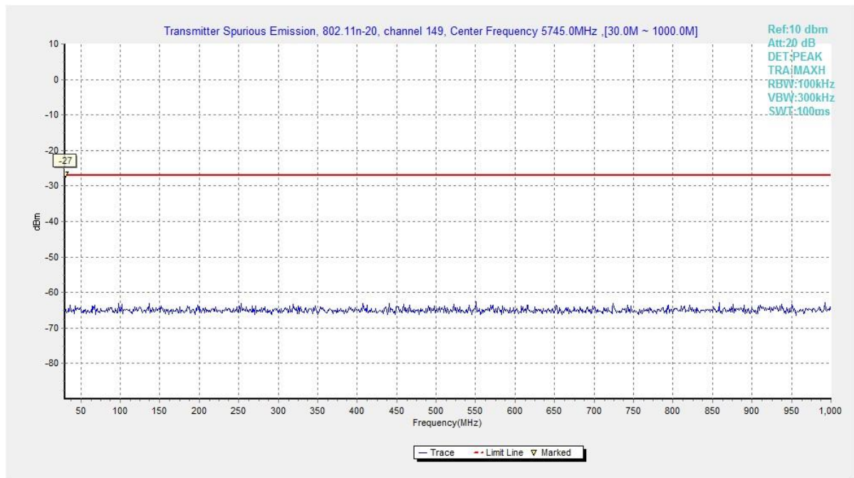
Fig. 21 Conducted Spurious Emission (802.11n20, Ch149 , 30 MHz ~ 1 GHz)
