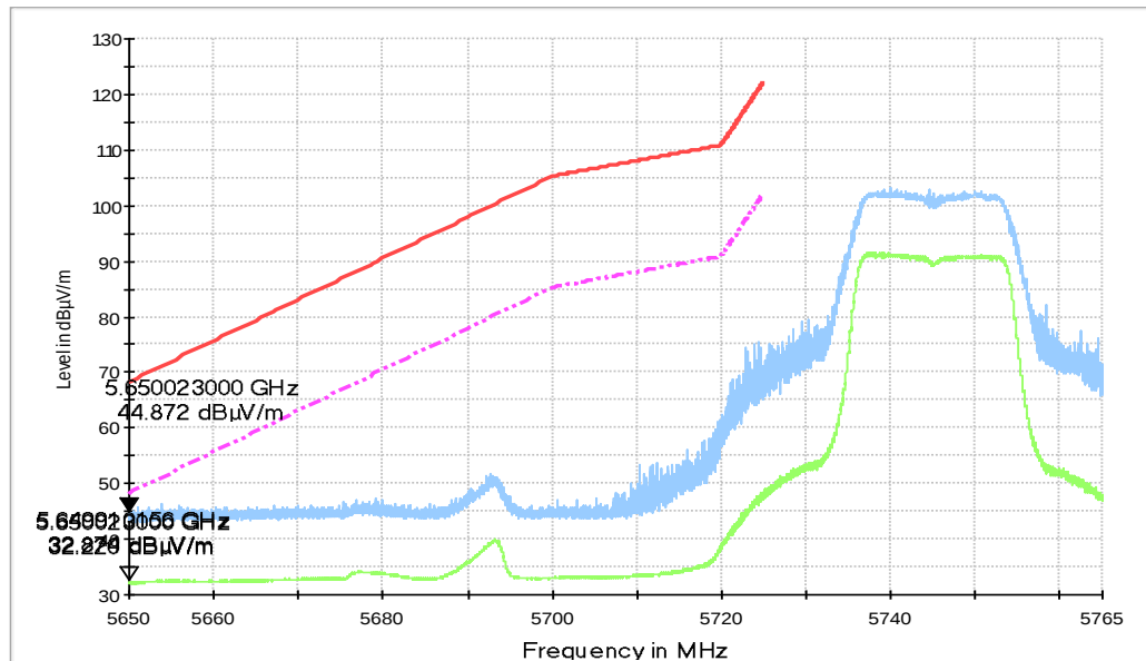
Fig. 49 Band Edges (802.11n-HT20, 5745MHz)
