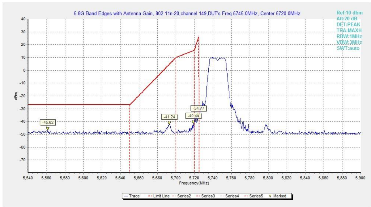
Fig. 43 Band Edges (802.11n20, 5745MHz)
