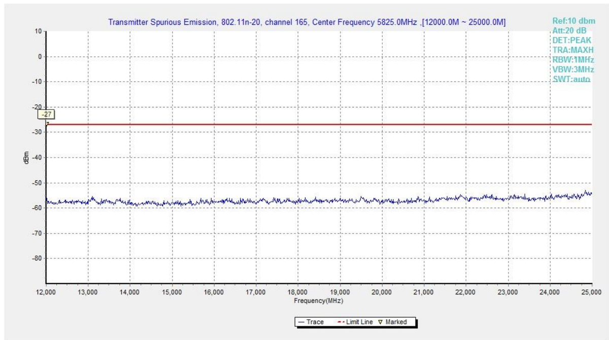
Fig. 31 Conducted Spurious Emission (802.11n20, Ch165 , 12 GHz ~ 25 GHz)
