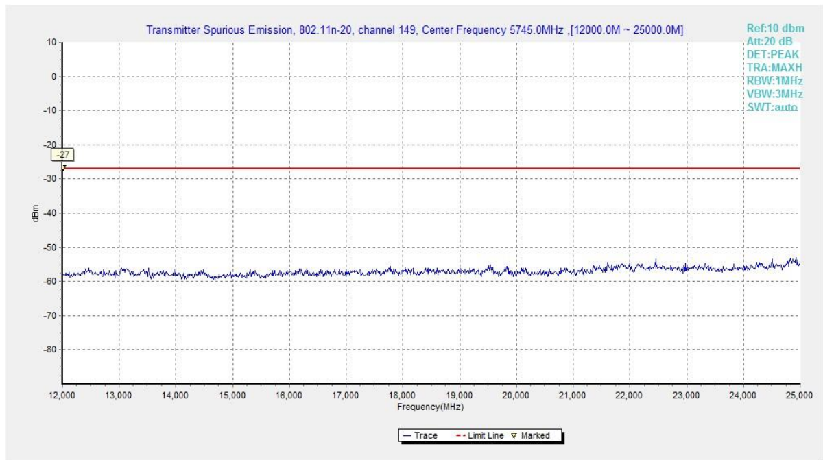
Fig. 23 Conducted Spurious Emission (802.11n20, Ch149, 12 GHz ~ 25 GHz)
