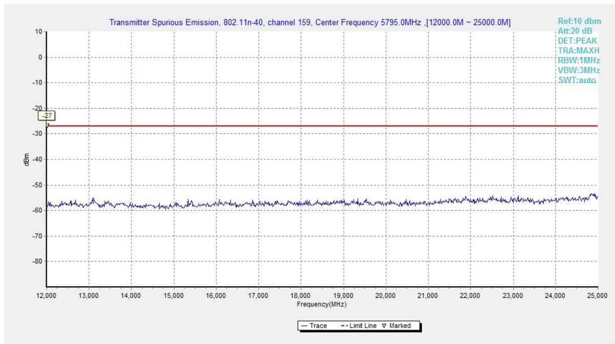
Fig. 39 Conducted Spurious Emission (802.11n40, Ch159 , 12 GHz ~ 25 GHz)
