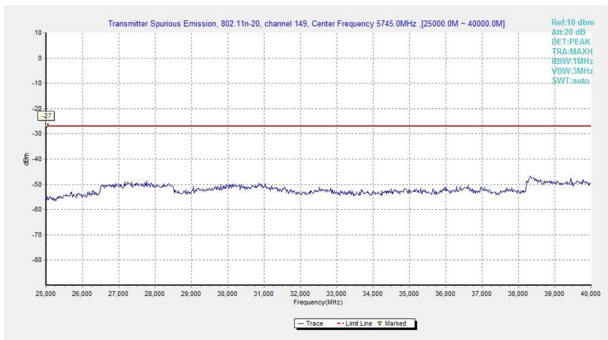
Fig. 24 Conducted Spurious Emission (802.11n20, Ch149, 25 GHz ~ 40 GHz)
