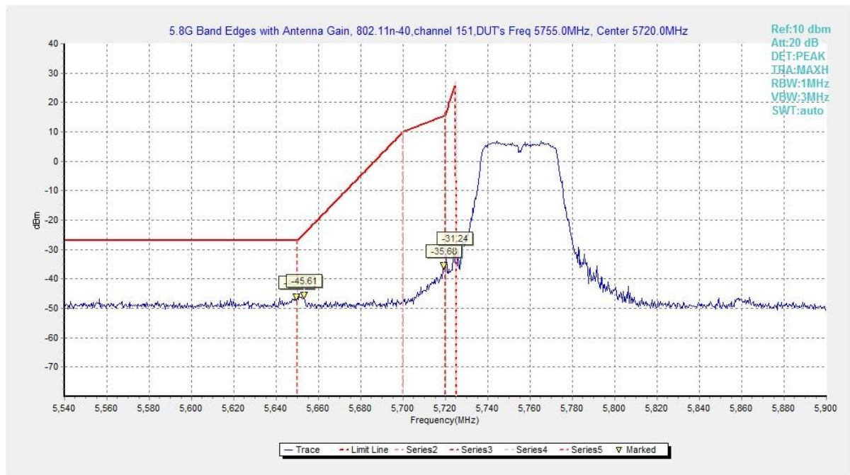
Fig. 45 Band Edges (802.11n40, 5755MHz)
