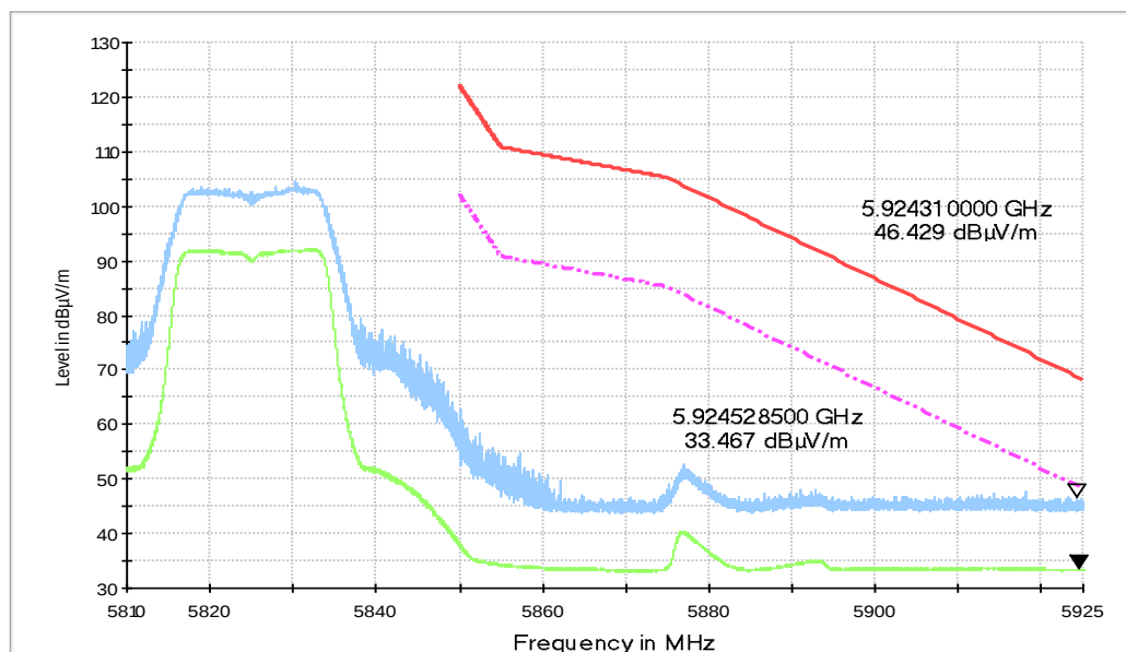
Fig. 50 Band Edges (802.11n-HT20, 5825MHz)
