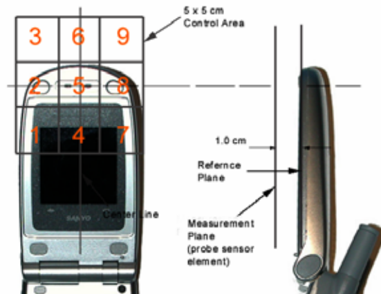
Figure 13 E/H-Field Emissions Test Setup Diagram
