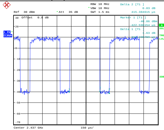
Duty Cycle
