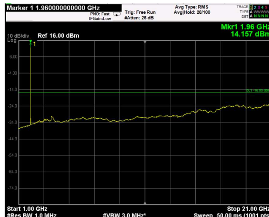
Channel: MIDDLE, Modulation: 256QAM, BW=10MHz, Range: Upper
