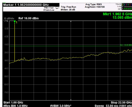
Channel: MIDDLE, Modulation: QPSK, BW=5MHz, Range: Upper
