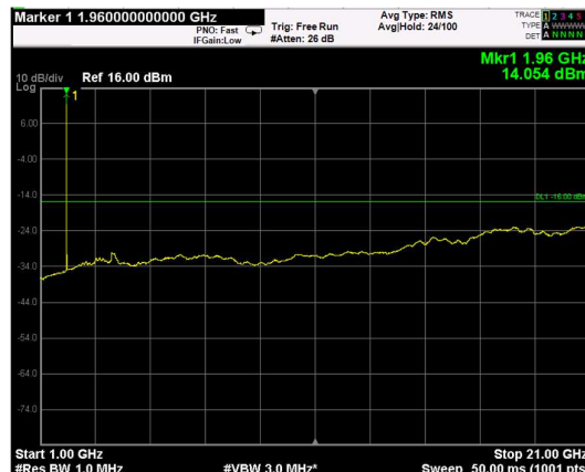
Channel: MIDDLE, Modulation: 64QAM, BW=10MHz, Range: Upper
