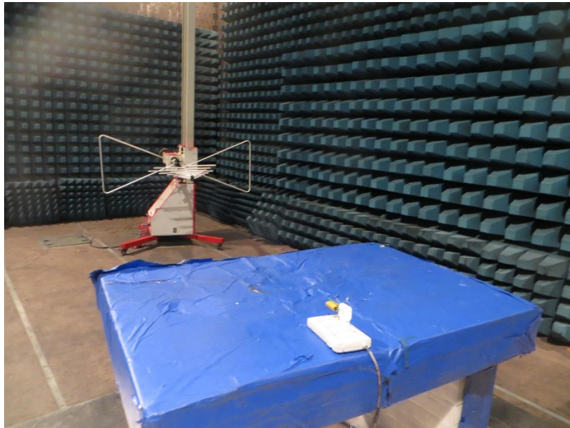
Radiated emission
