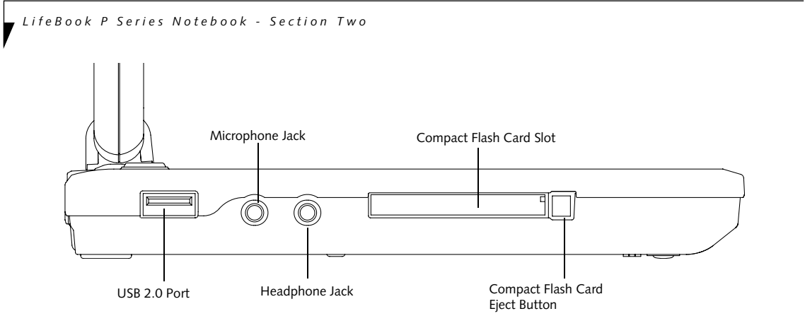
Figure 2-5. LifeBook P Series notebook left-side panel
