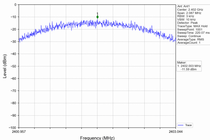
2M_LCH_2402MHz_DataRate= Ant1_NTNV
