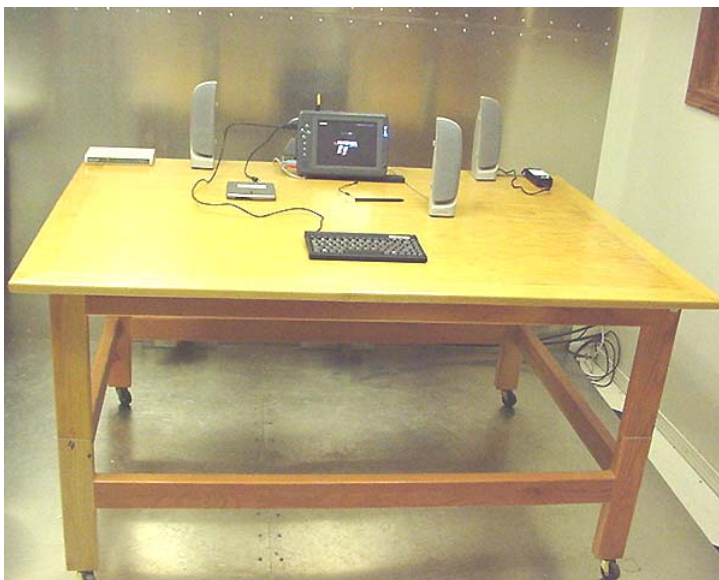
Photograph B.6-2 - AC Powerline Conducted Emission Cable Placement
