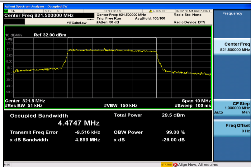
Band26-5MHz-16QAM-26765-25RB#0-4.4747
