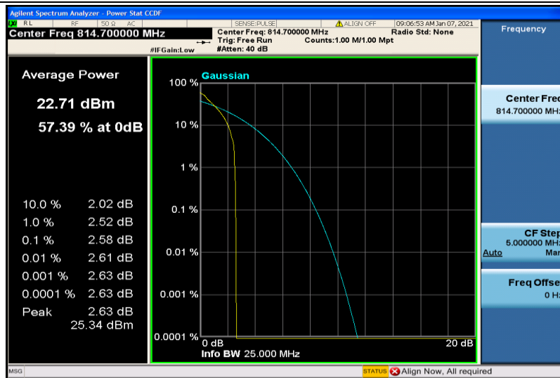
Band26-1.4MHz-QPSK-26697-1RB#0
