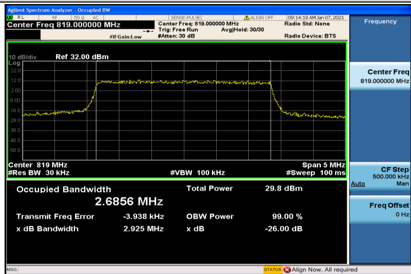
Band26-3MHz-QPSK-26740-15RB#0-2.6856
