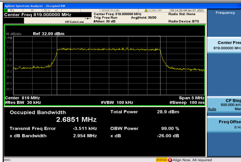
Band26-3MHz-16QAM-26740-15RB#0-2.6851
