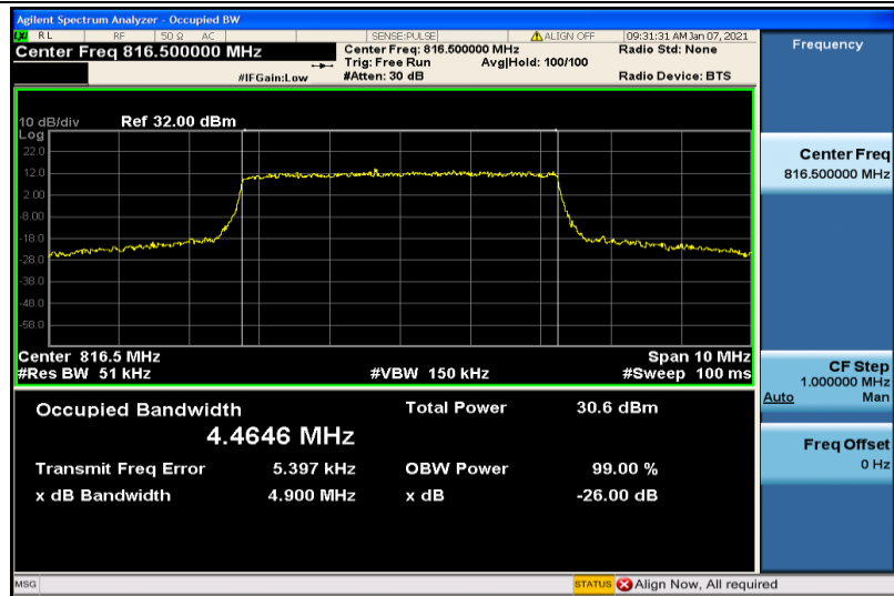
Band26-5MHz-QPSK-26715-25RB#0-4.4646
