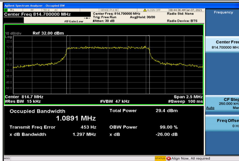
Band26-1.4MHz-QPSK-26697-6RB#0-1.0891
