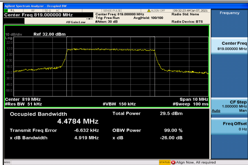
Band26-5MHz-16QAM-26740-25RB#0-4.4784
