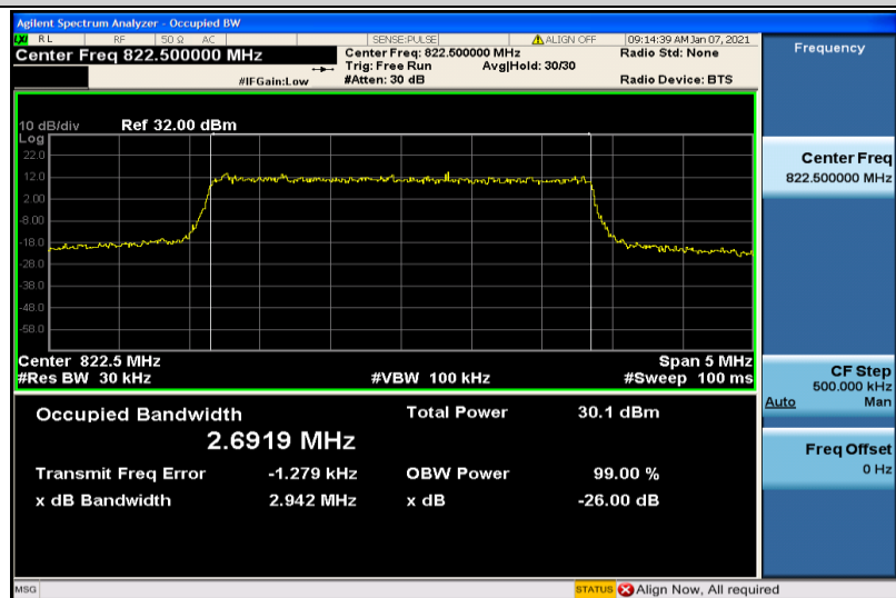
Band26-3MHz-QPSK-26775-15RB#0-2.6919
