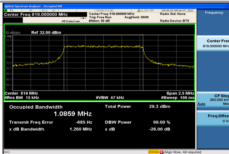
Band26-1.4MHz-QPSK-26740-6RB#0-1.0859
