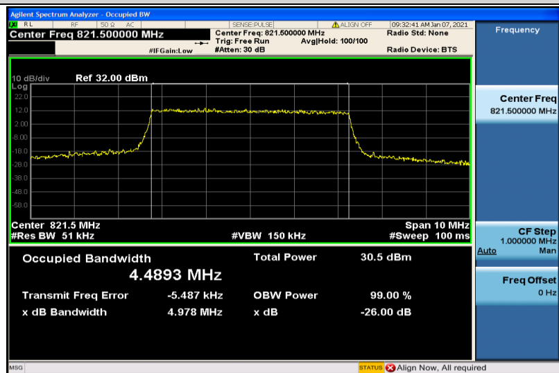
Band26-5MHz-QPSK-26765-25RB#0-4.4893
