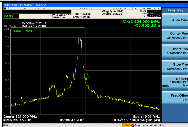
Band26-1.4MHz-QPSK-26783-1RB#5
