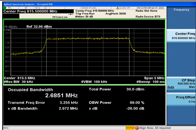
Band26-3MHz-QPSK-26705-15RB#0-2.6851
