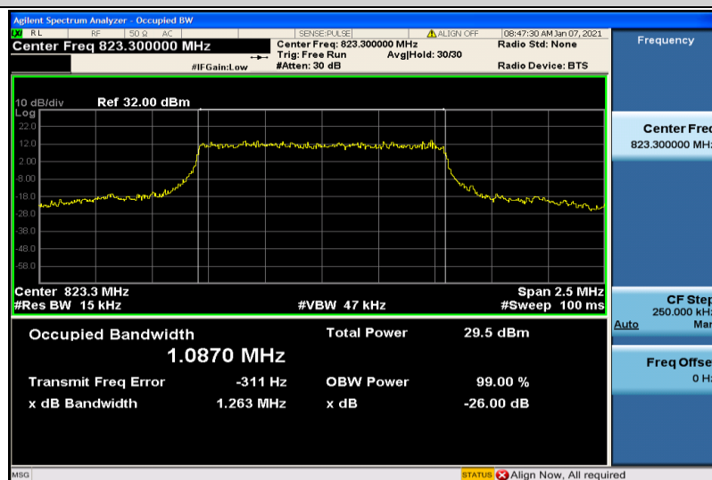
Band26-1.4MHz-QPSK-26783-6RB#0-1.0870
