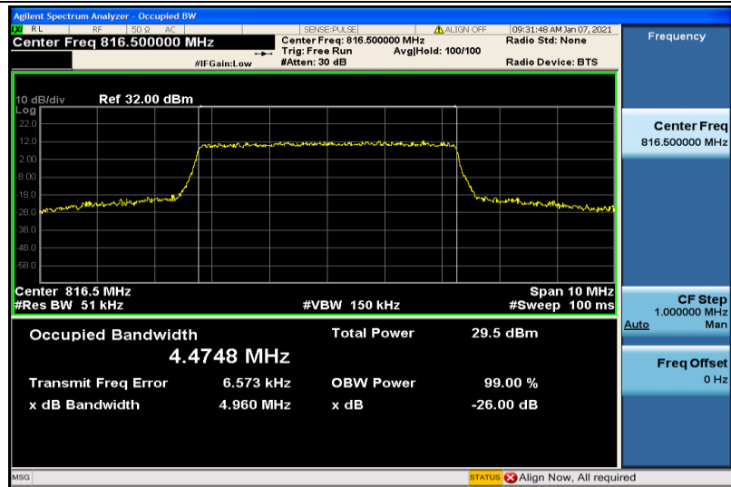
Band26-5MHz-16QAM-26715-25RB#0-4.4748
