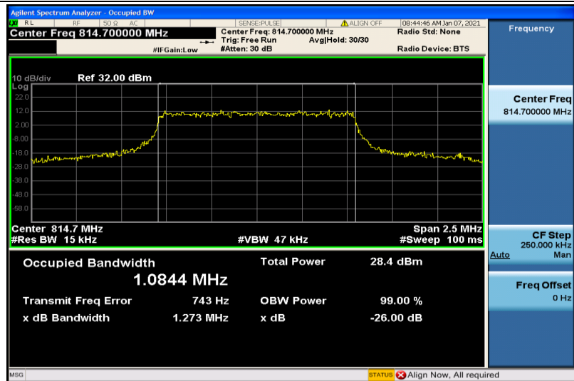
Band26-1.4MHz-16QAM-26697-6RB#0-1.0844
