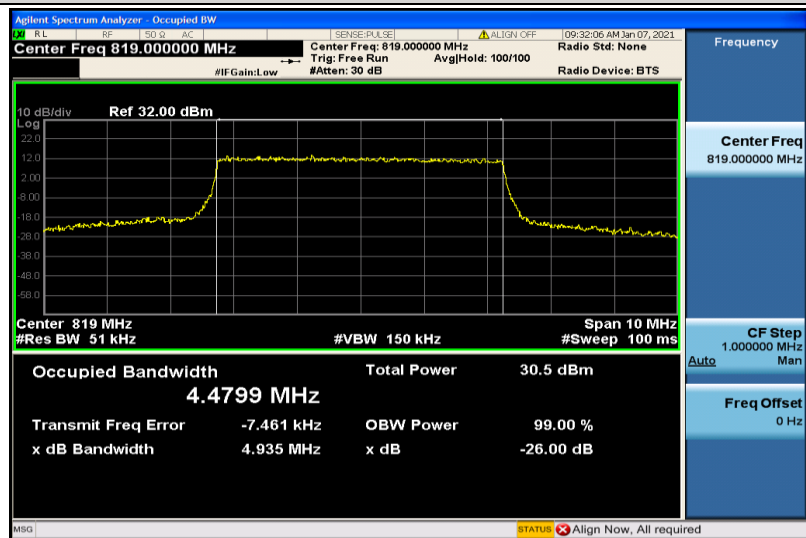
Band26-5MHz-QPSK-26740-25RB#0-4.4799
