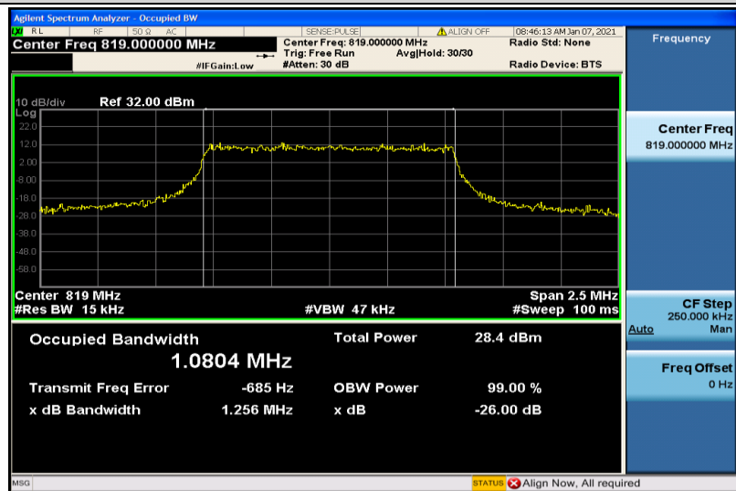
Band26-1.4MHz-16QAM-26740-6RB#0-1.0804
