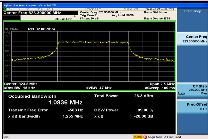
Band26-1.4MHz-16QAM-26783-6RB#0-1.0836
