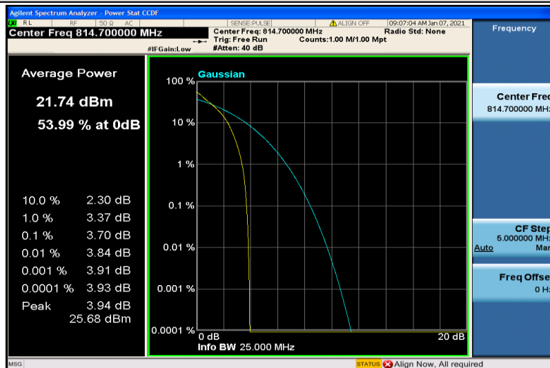
Band26-1.4MHz-QPSK-26697-6RB#0
