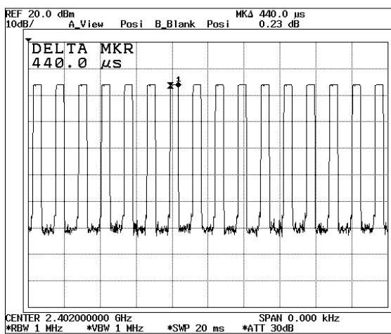
CH 00 2402MHz
