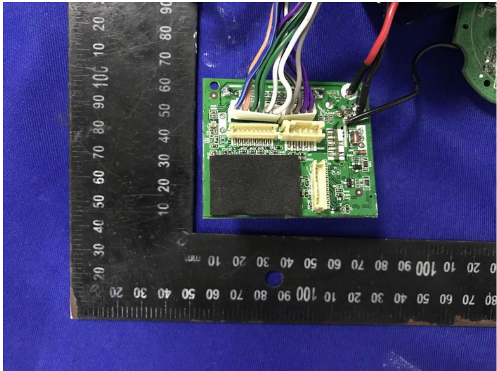
Internal Photos M/N: KD-MR1BTS
