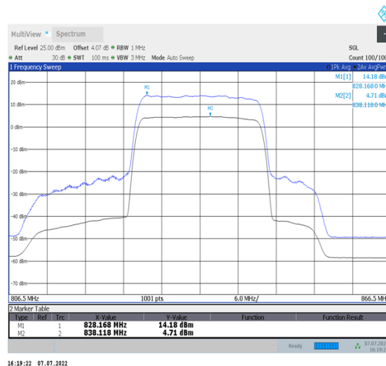
1-N26-824-849--15-20-L-2-CP-256QAM-Outer_Full-106@0-Ant1-9.81-100%-0.00-9.81-PASS-≤13
