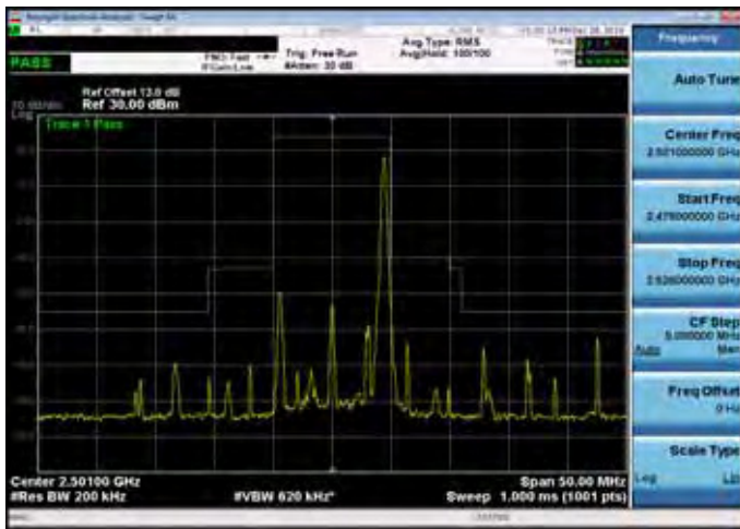
Emission Mask_Band 41_10M_QPSK_MID_RB1,49
