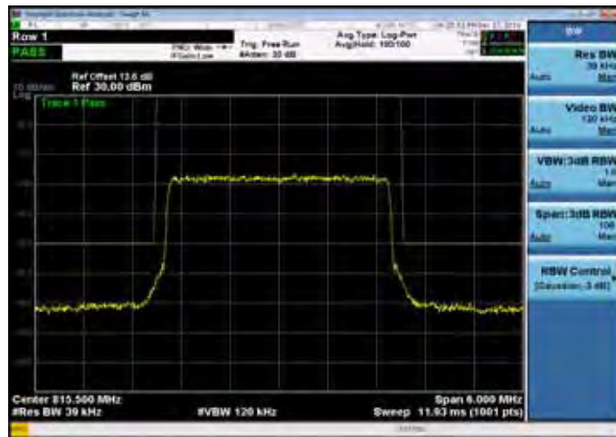
Emission Mask_Band26 for Part 90S_3M_QPSK_MID_RB15,0
