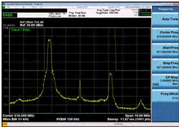
Emission Mask_Band26 for Part 90S_5M_QPSK_MID_RB1,0
