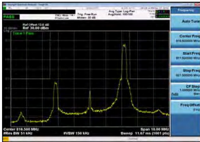
Emission Mask_Band26 for Part 90S_5M_QPSK_MID_RB1,24
