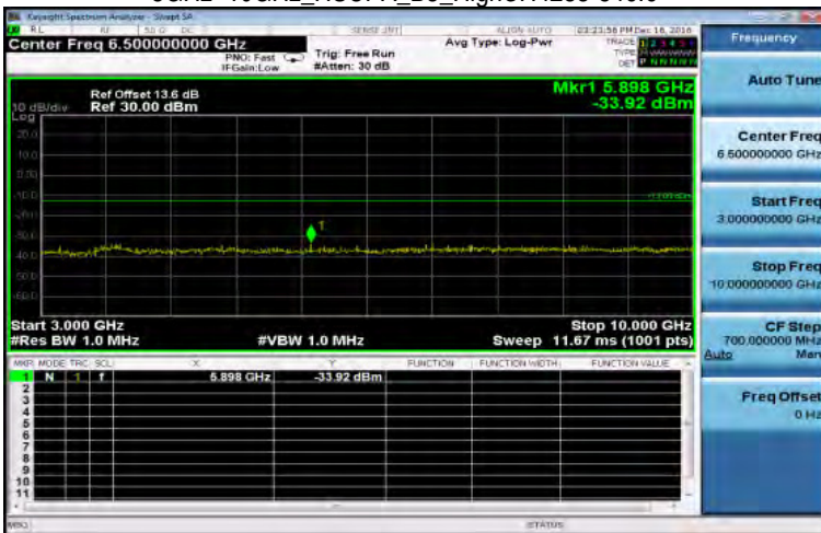
3GHz~10GHz_HSUPA_B5_HighCH4233-846.6
