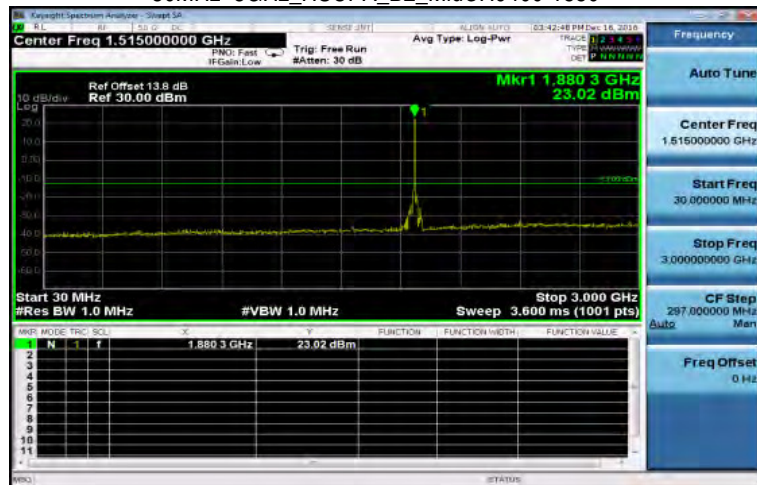
30MHz~3GHz_HSUPA_B2_MidCH9400-1880
