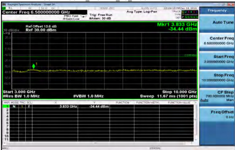
3GHz~10GHz_WCDMA_B5_MidCH4183-836.6
