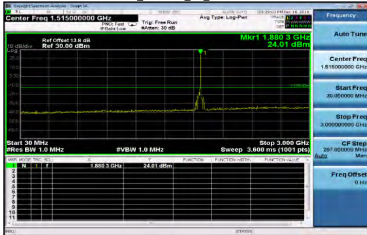
30MHz~3GHz_WCDMA_B2_MidCH9400-1880
