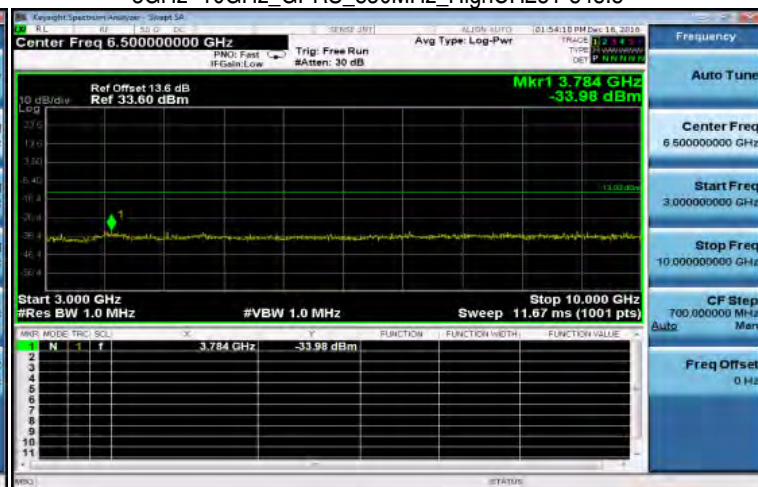
3GHz~10GHz_GPRS_850MHz_HighCH251-848.8
