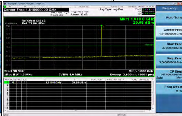
30MHz~3GHz_GSM_1900MHz_HighCH810-1909.8
