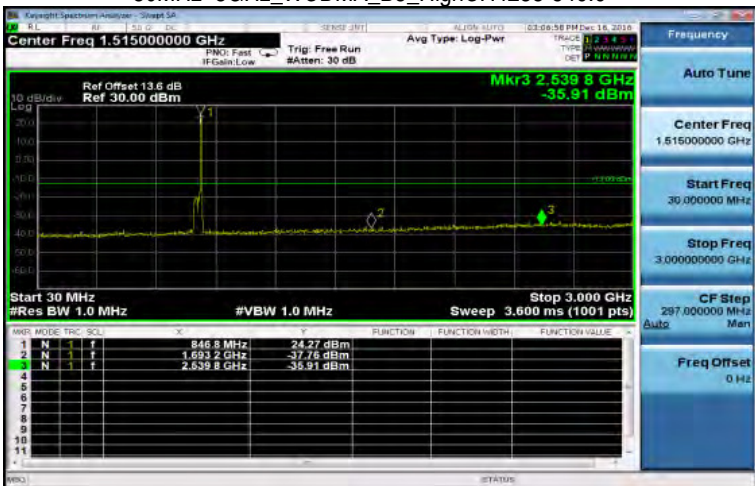
30MHz~3GHz_WCDMA_B5_HighCH4233-846.6
