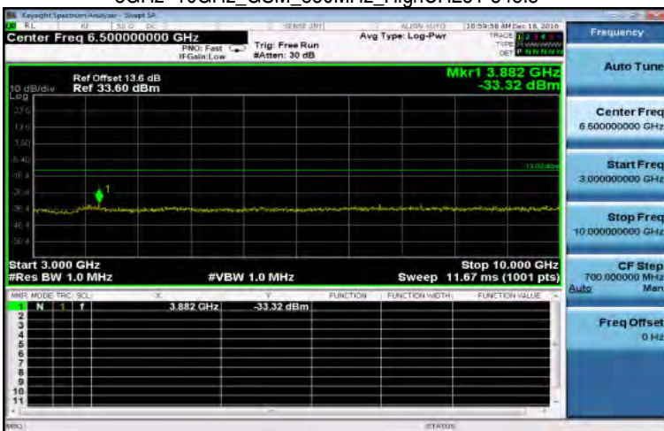
3GHz~10GHz_GSM_850MHz_HighCH251-848.8
