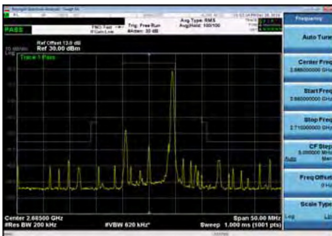
Emission Mask_Band 41_10M_QPSK_HIGH_RB1,49
