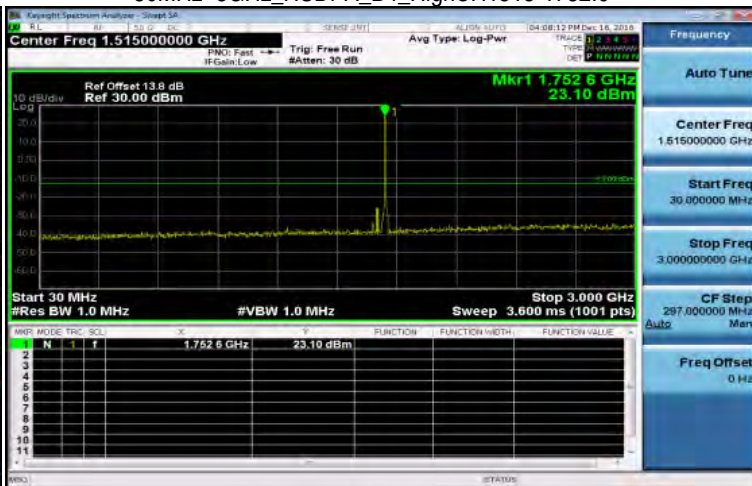
30MHz~3GHz_HSDPA_B4_HighCH1513-1752.6
