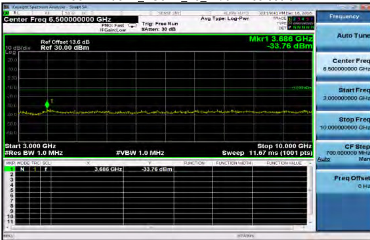
3GHz~10GHz_HSUPA_B5_MidCH4183-836.6
