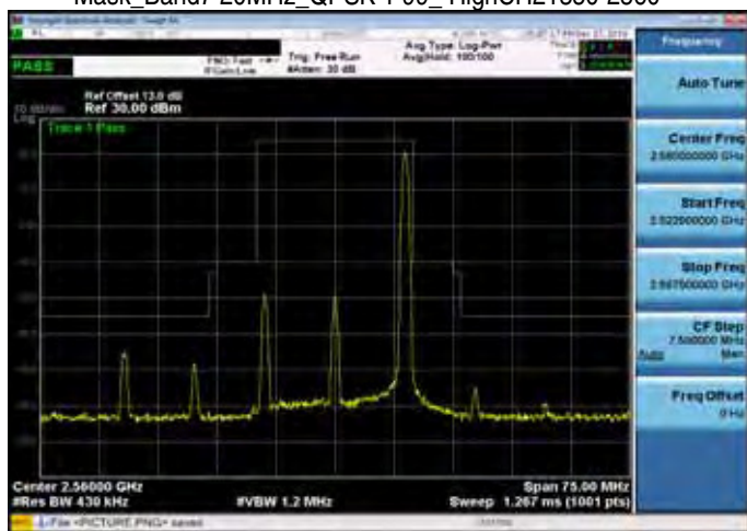
Mask_Band7 20MHz_QPSK 1 99_ HighCH21350-2560
