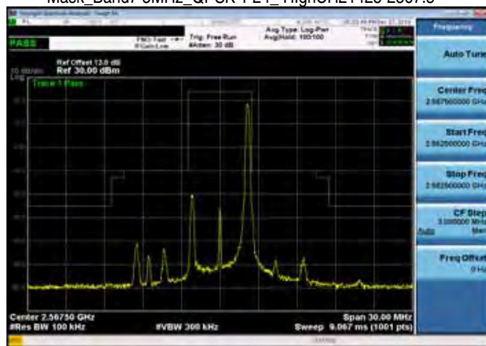
Mask_Band7 5MHz_QPSK 1 24_HighCH21425-2567.5
