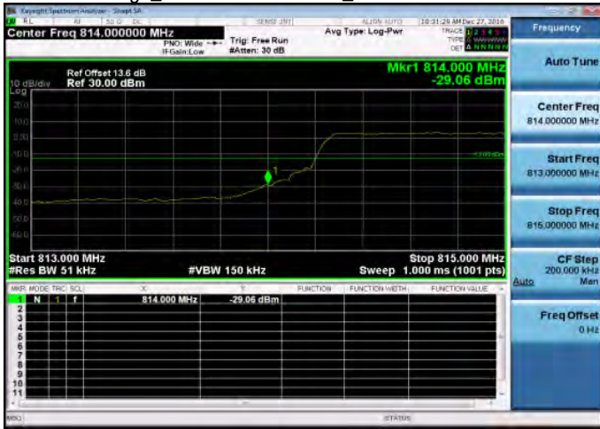
Band Edge_Band 26 for Part 90S_5M-QPSK-25 0-LOW
