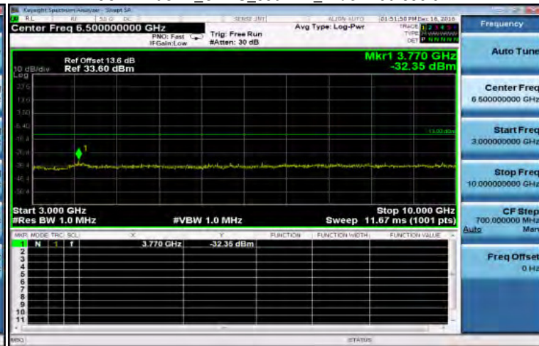
3GHz~10GHz_GPRS_850MHz_MidCH190-836.6
