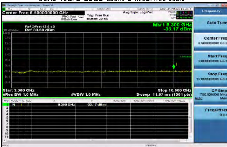
3GHz~10GHz_EDGE_850MHz_MidCH190-836.6
