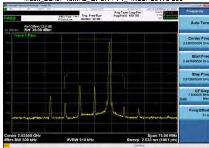
Mask_Band7 15MHz_QPSK 1 74_MidCH20175-253
