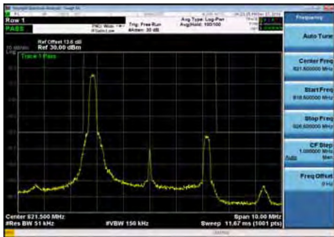
Emission Mask_Band26 for Part 90S_5M_QPSK_HIGH_RB1,0
