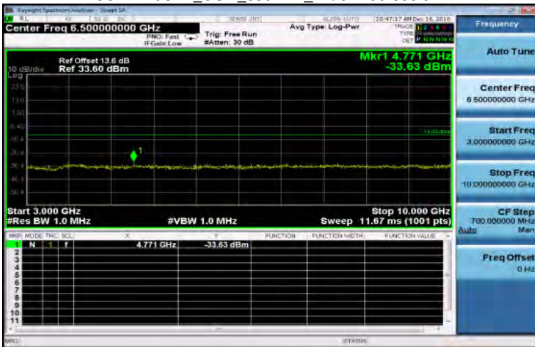
3GHz~10GHz_GSM_850MHz_MidCH190-836.6
