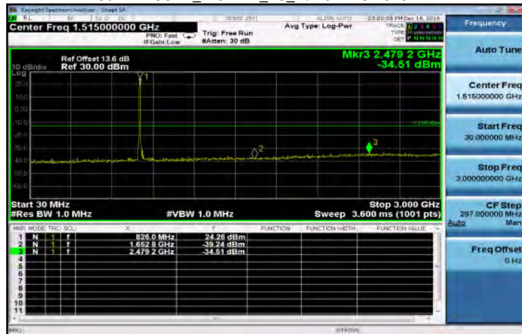
30MHz~3GHz_WCDMA_B5_LowCH4132-826.4
