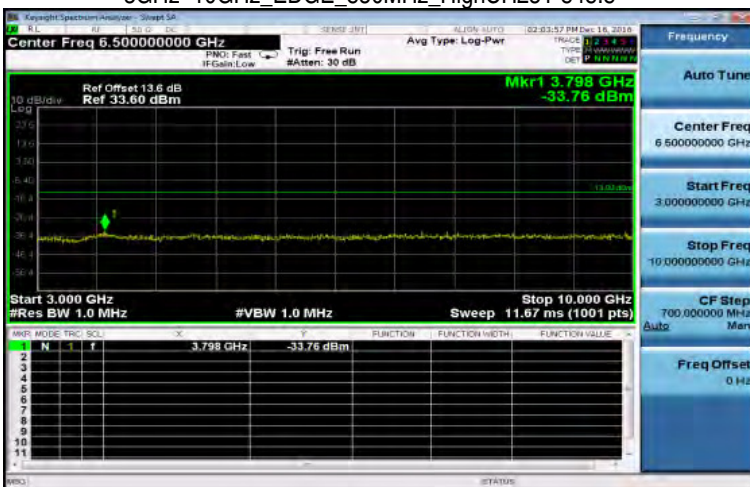
3GHz~10GHz_EDGE_850MHz_HighCH251-848.8
