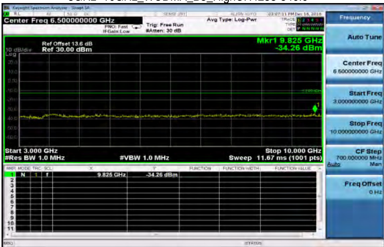
3GHz~10GHz_WCDMA_B5_HighCH4233-846.6
