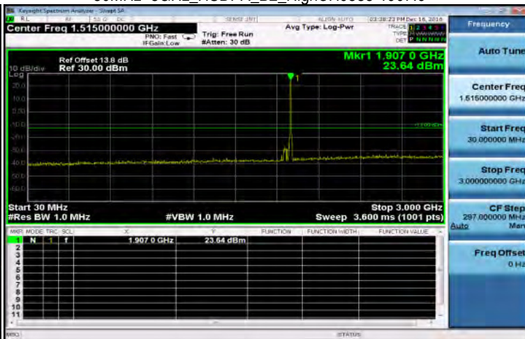
30MHz~3GHz_HSDPA_B2_HighCH9538-1907.6
