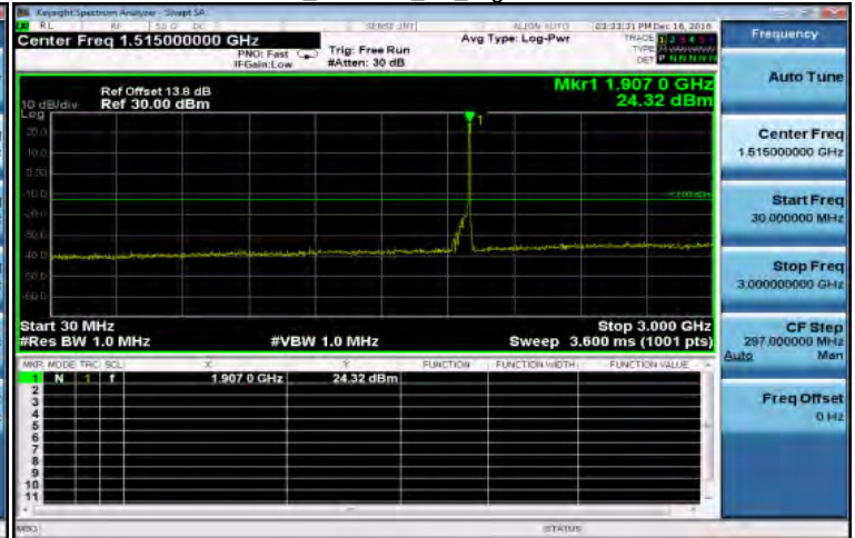
30MHz~3GHz_WCDMA_B2_HighCH9538-1907.6
