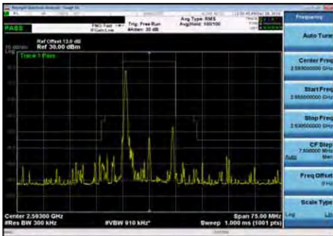
Emission Mask_Band 41_15M_QPSK_HIGH_RB1,0
