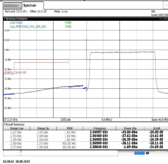
Band38-20MHz-16QAM-38150-100RB#0
