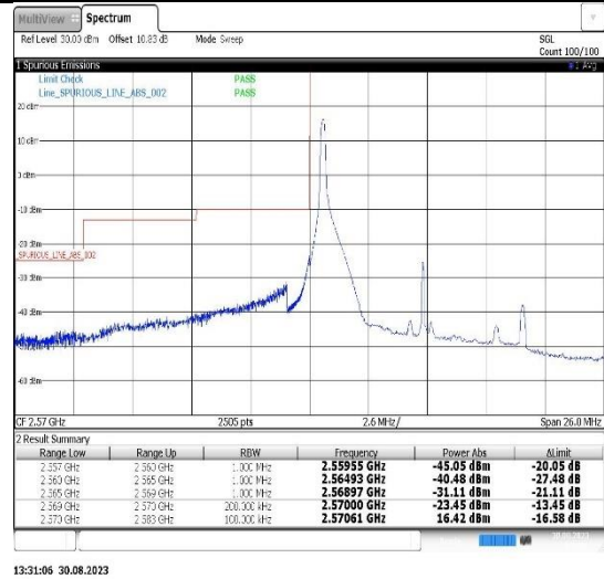
Band38-10MHz-QPSK-38200-1RB#49
