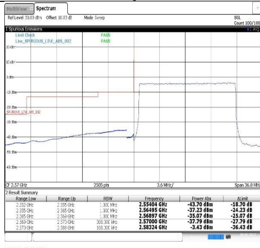
Band38-15MHz-16QAM-38175-75RB#0
