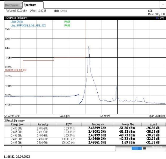
Band41-10MHz-16QAM-41540-1RB#49
