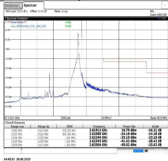
Band38-15MHz-16QAM-37825-1RB#0
