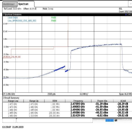
Band41-20MHz-16QAM-41490-100RB#0
