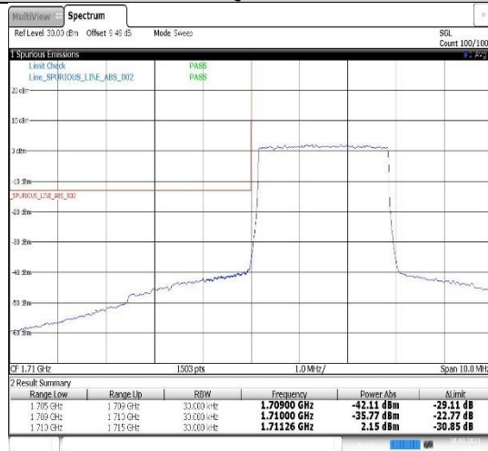
Band66-3MHz-16QAM-131987-15RB#0
