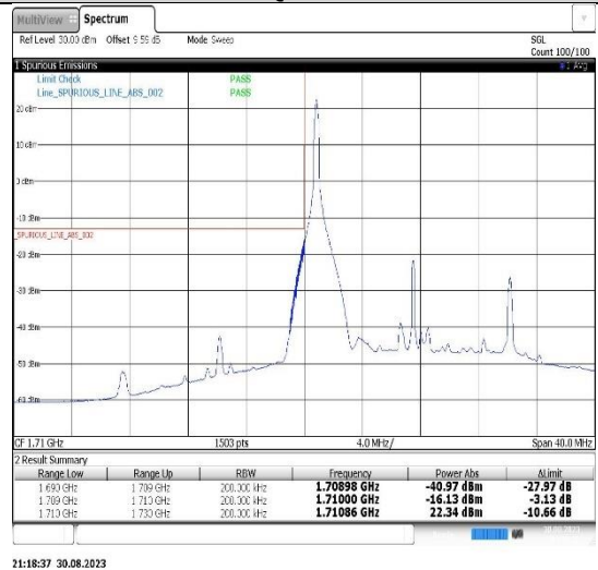
Band66-15MHz-QPSK-132597-1RB#74
