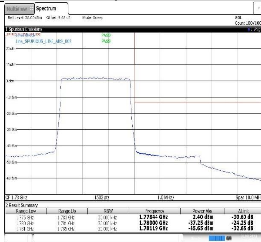
Band66-3MHz-QPSK-132657-15RB#0
