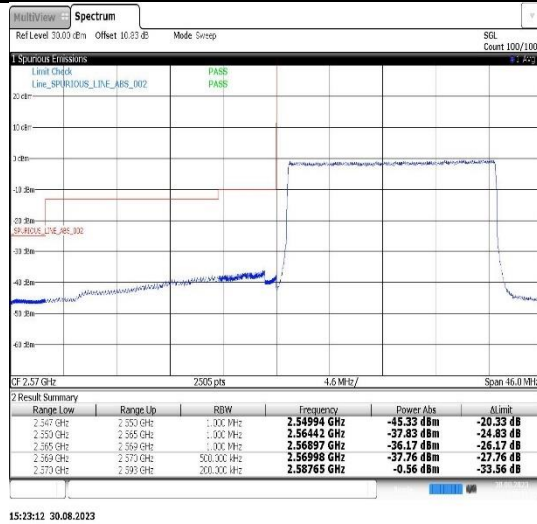
Band38-20MHz-QPSK-38150-100RB#0
