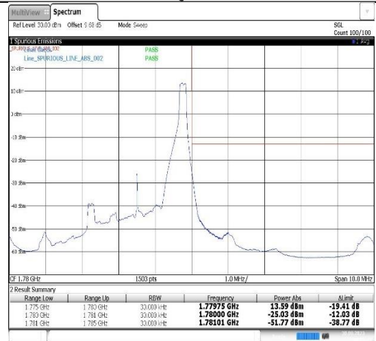
Band66-3MHz-16QAM-132657-1RB#14
