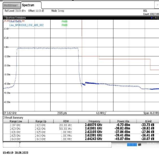
Band38-20MHz-16QAM-37850-100RB#0
