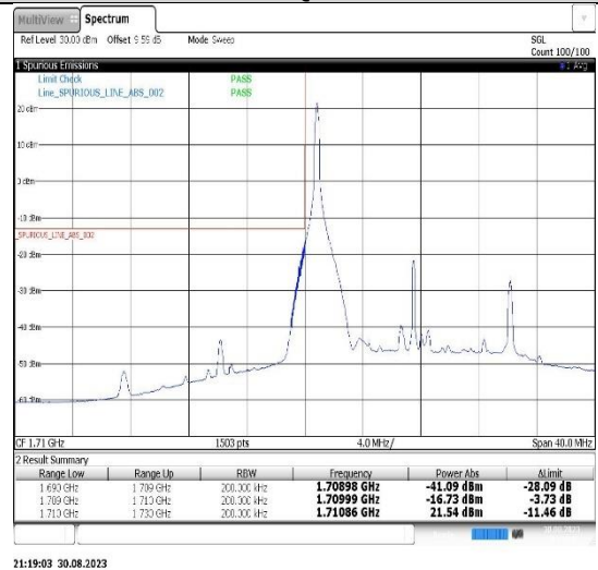
Band66-15MHz-16QAM-132047-1RB#74
