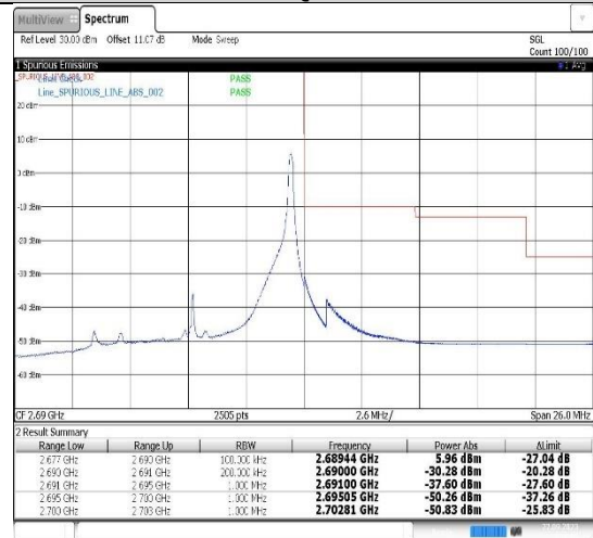
Band41-10MHz-16QAM-41540-1RB#49
