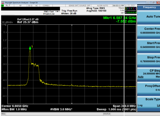
Plot 7-525. LPI Power Spectral Density Plot Antenna WF2a (160MHz) 802.11ax RU26 (UNII Band 7) - Ch. 143)
