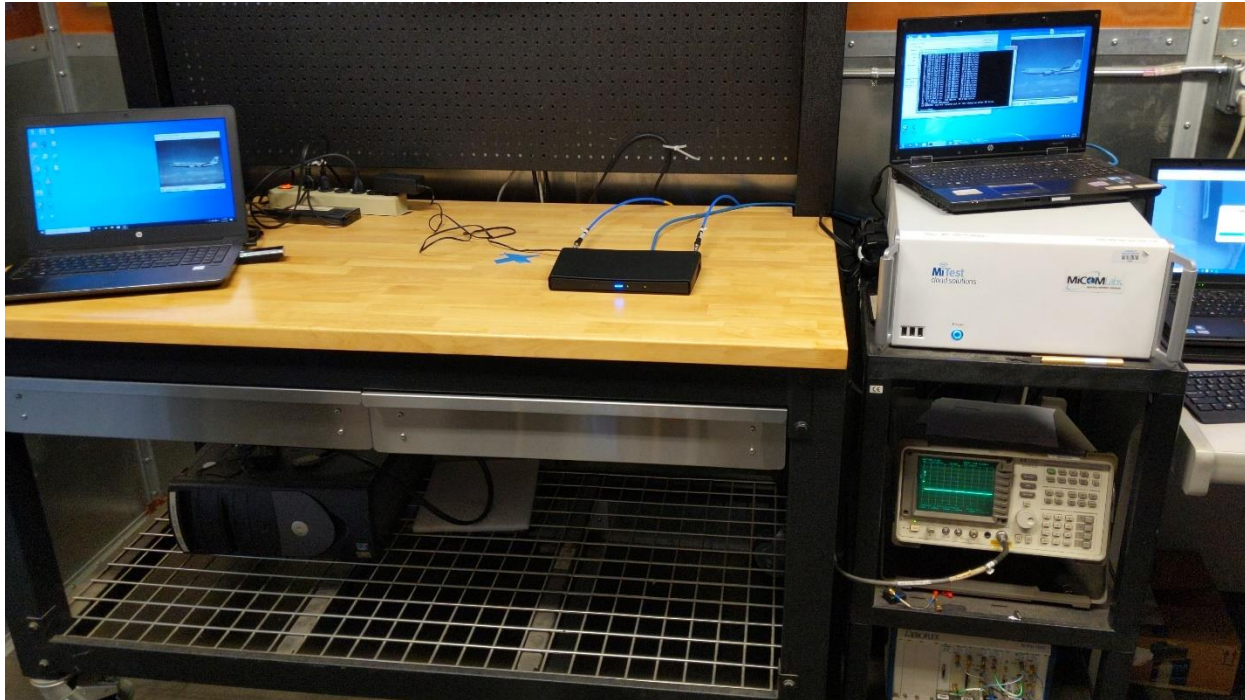
Conducted DFS Setup
