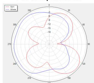
Phi=0 freq=2450MHz
