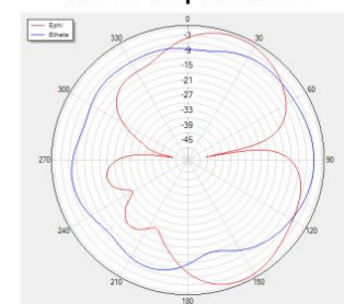
Phi=90 freq=2500MHz
