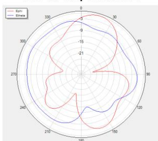
Phi=90 freq=2400MHz
