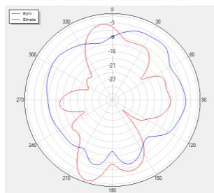
Phi=90 freq=5650MHz
