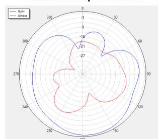
Theta=90 freq=2450MHz
