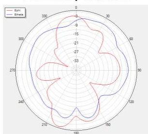
Phi=90 freq=5700MHz
