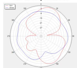
Phi=90 freq=2450MHz
