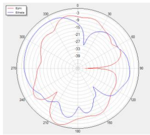
Phi=90 freq=5100MHz
