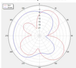
Phi=0 freq=2400MHz
