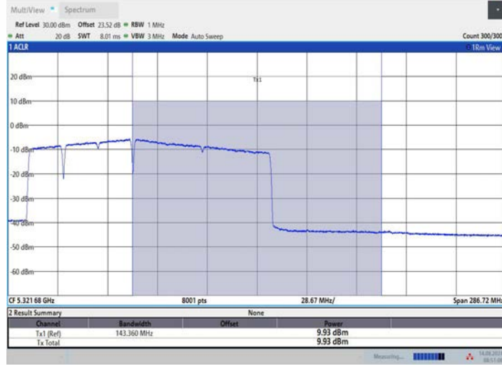
11BE160MIMO Ant1 5250 UNII-2A 996+484+242 OFDMA 1
