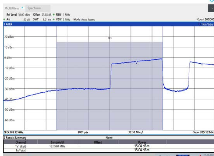
11BE160MIMO Ant3 5250 UNII-1 996+484 OFDMA 4
