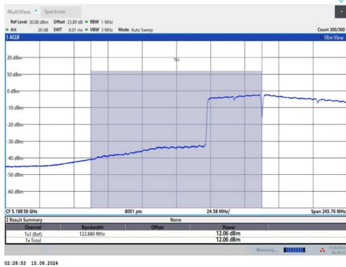
11BE160MIMO_Ant2_5250_UNII-1_996+484_OFDMA_2
