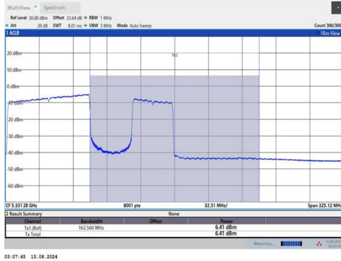
11BE160MIMO_Ant2_5250_UNII-2A_996+484_OFDMA_3
