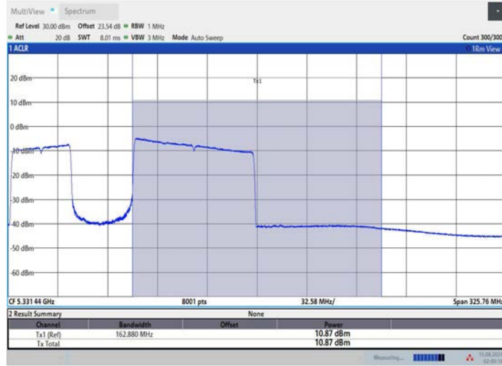
11BE160MIMO Ant3 5250 UNII-2A 996+484 OFDMA_2
