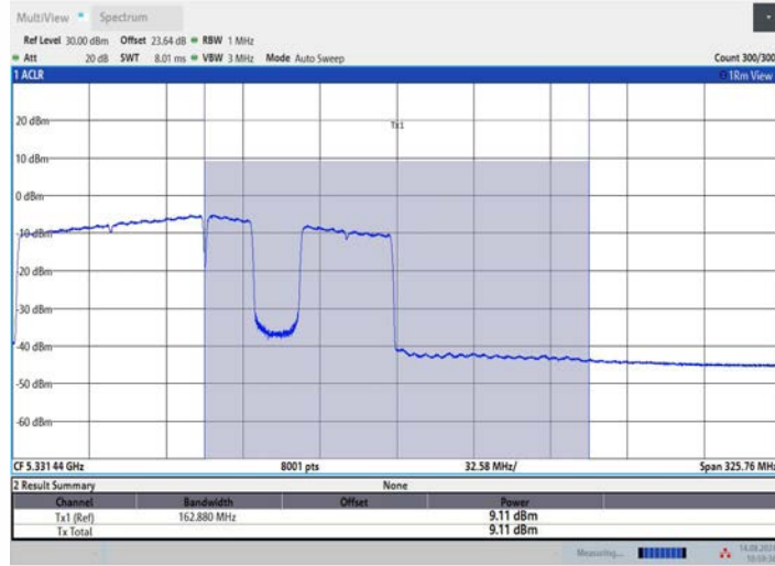
11BE160MIMO Ant2 5250 UNII-2A 996+484+242 OFDMA 6
