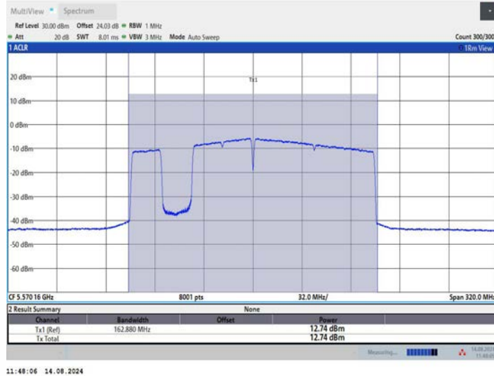
11BE160MIMO Ant1 5570 996+484+242 OFDMA 2
