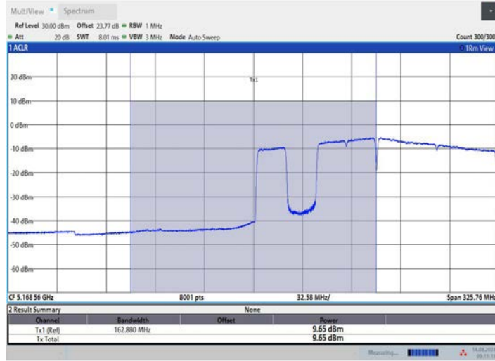
11BE160MIMO_Ant1_5250_UNII-1_996+484+242_OFDMA_2
