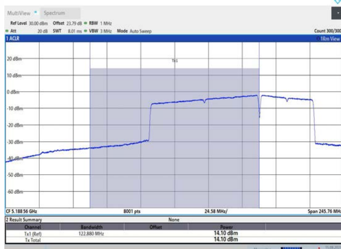
11BE160MIMO_Ant3_5250_UNII-1_996+484+242_OFDMA_1
