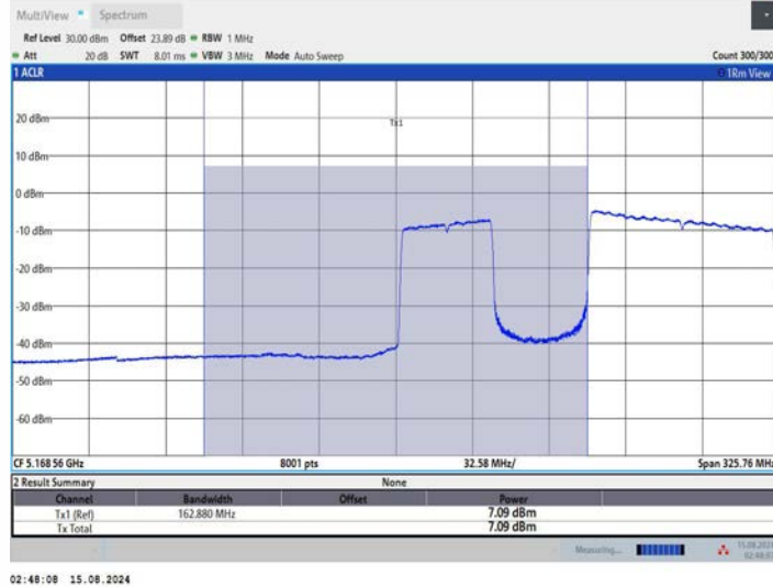
11BE160MIMO_Ant2_5250_UNII-1_996+484_OFDMA_2
