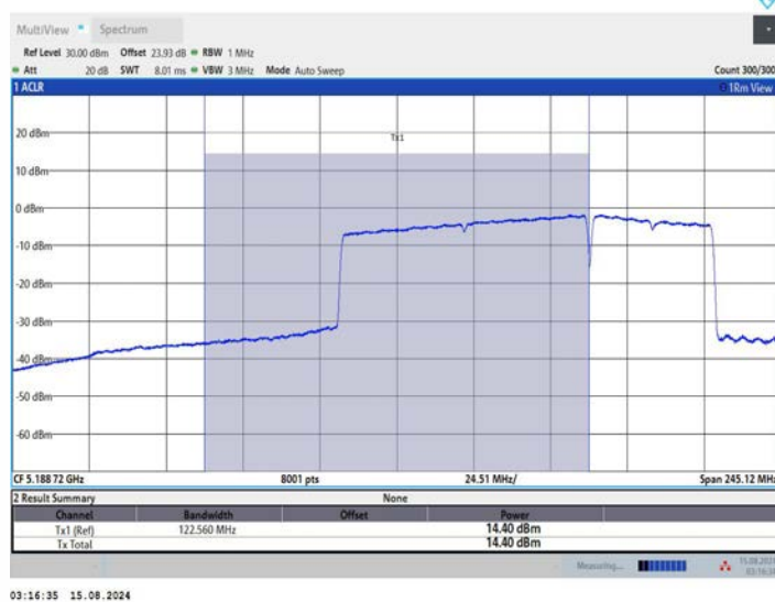
11BE160MIMO_Ant2_5250_UNII-1_996+484+242_OFDMA_1
