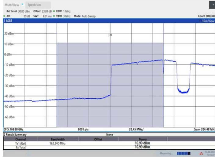
11BE160MIMO_Ant1_5250_UNII-1_996+484+242_OFDMA_6
