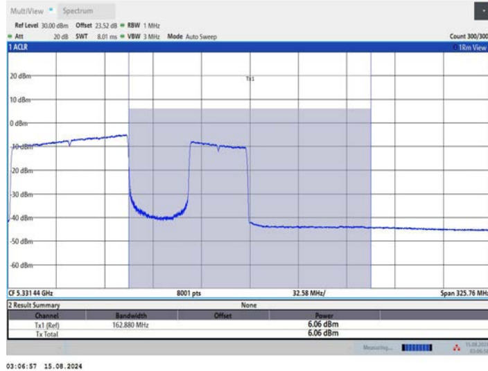
11BE160MIMO_Ant1_5250_UNII-2A_996+484_OFDMA_3
