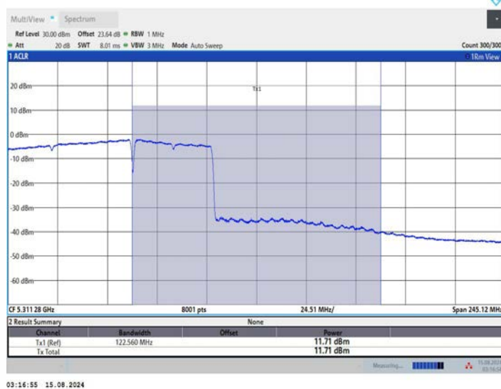
11BE160MIMO Ant2 5250 UNII-2A 996+484+242 OFDMA 1
