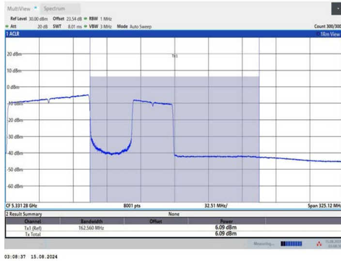
11BE160MIMO_Ant3_5250_UNII-2A_996+484_OFDMA_3
