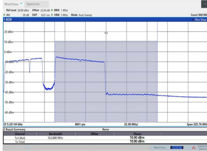
11BE160MIMO Ant2 5250 UNII-2A 996+484+242 OFDMA 4
