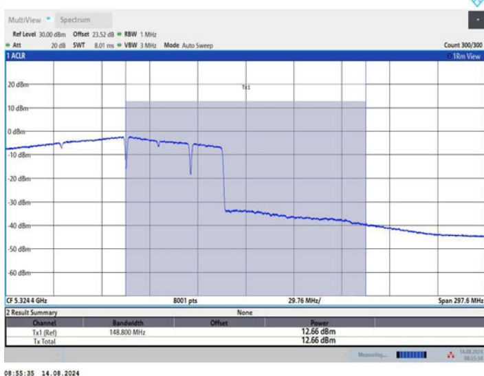
11BE160MIMO Ant2 5250 UNII-2A 996+484 OFDMA 1
