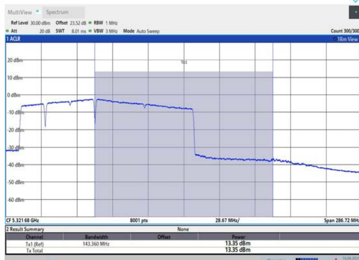
11BE160MIMO Ant1 5250 UNII-2A 996+484+242 OFDMA 2
