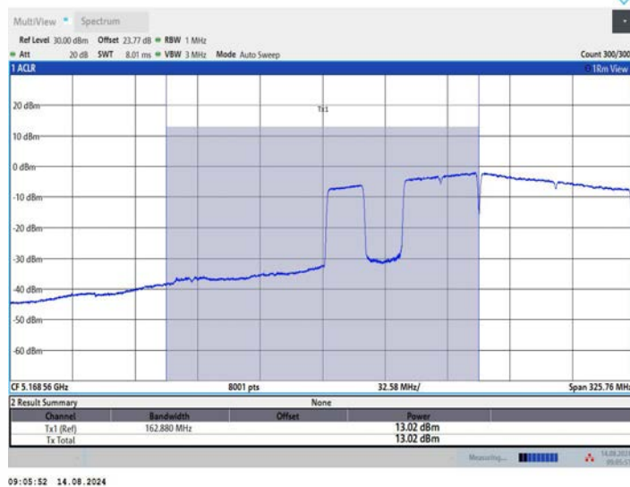
11BE160MIMO_Ant1_5250_UNII-1_996+484+242_OFDMA_3
