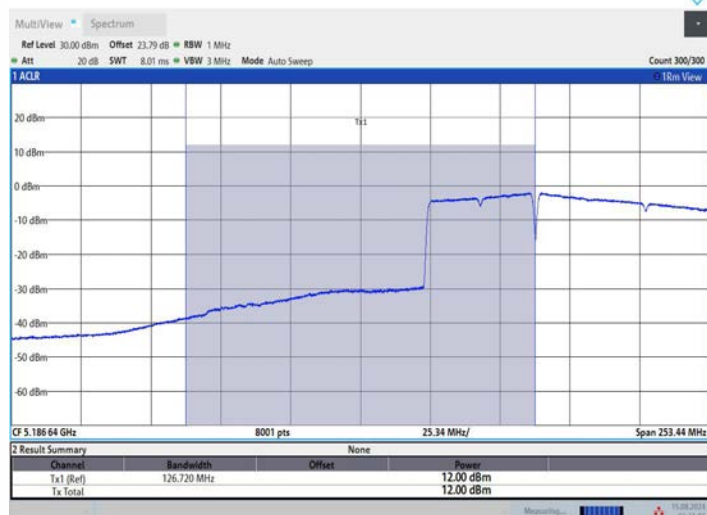
11BE160MIMO Ant3 5250 UNII-1 996+484 OFDMA 2
