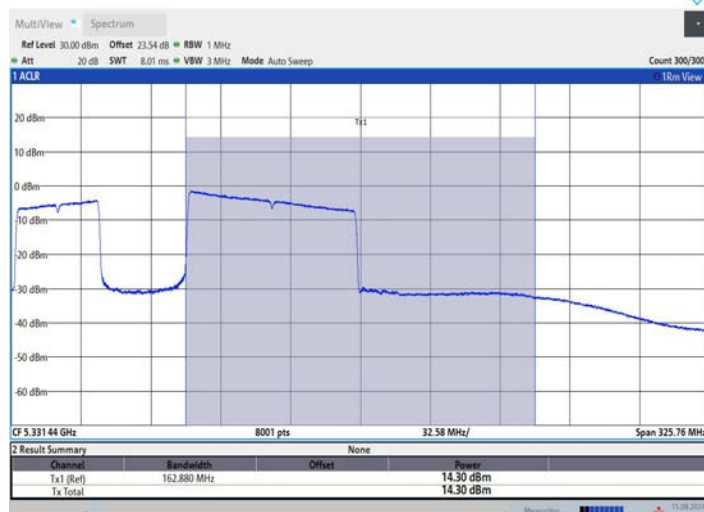
11BE160MIMO Ant3 5250 UNII-2A 996+484 OFDMA_3
