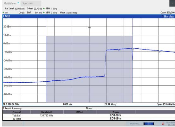
11BE160MIMO Ant3 5250 UNII-1 996+484 OFDMA 1
