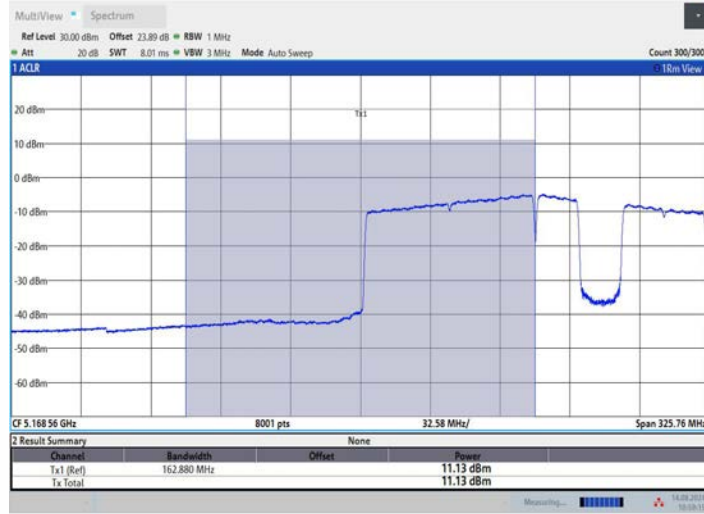
11BE160MIMO_Ant2_5250_UNII-1_996+484+242_OFDMA_6
