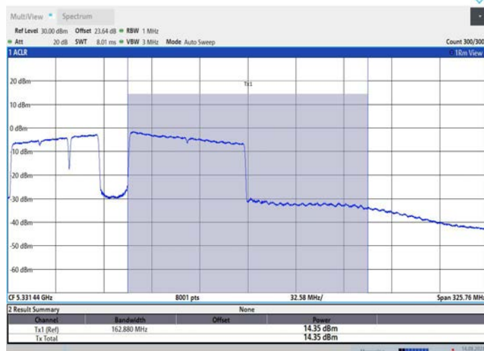
11BE160MIMO Ant2 5250 UNII-2A 996+484+242 OFDMA 5
