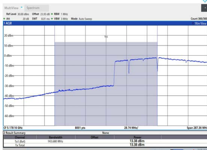
11BE160MIMO_Ant2_5250_UNII-1_996+484+242_OFDMA_2
