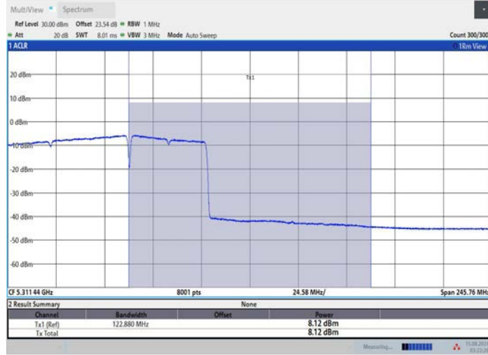
11BE160MIMO Ant3 5250 UNII-2A 996+484 OFDMA_4
