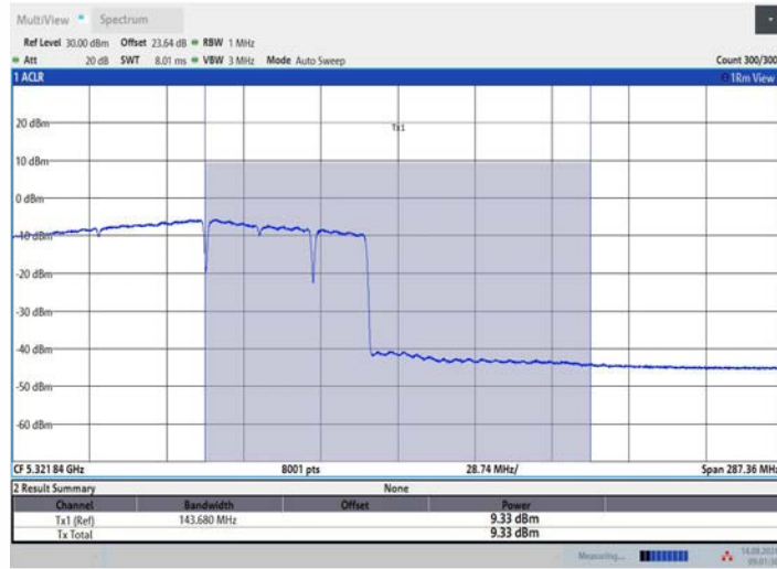
11BE160MIMO Ant2_5250_UNII-2A_996+484+242_OFDMA 8
