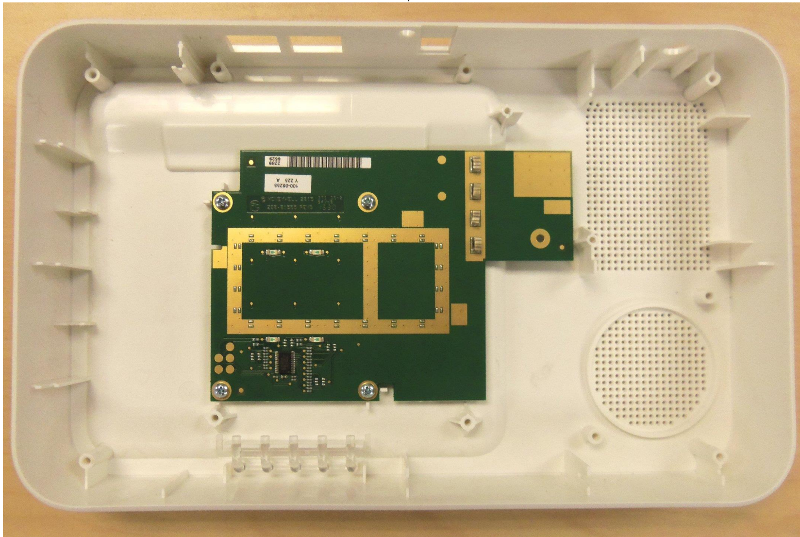
Keypad board showing from back.
