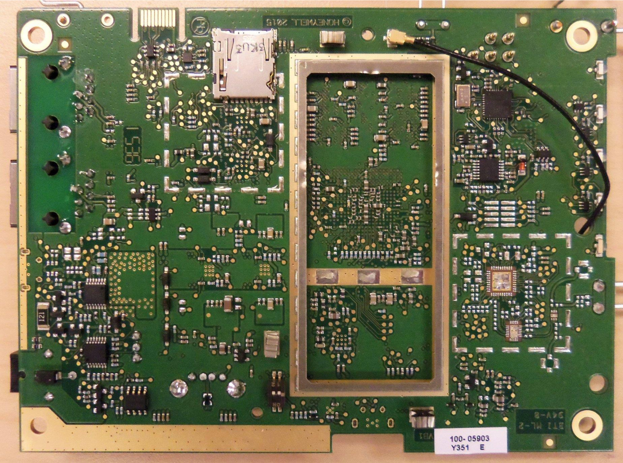
INTERNAL PHOTOS CONT. MAIN BOARD BOTTOM
