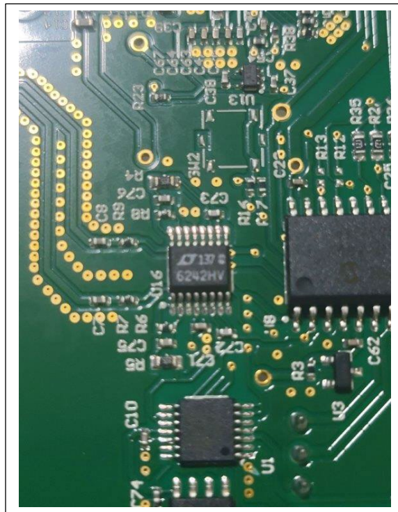
PCB 3
