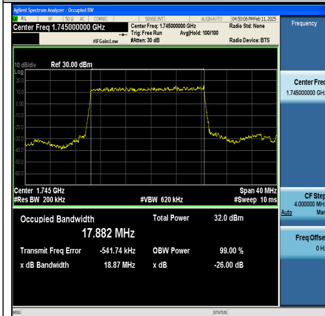
NTNV-n66-PC3-15-20-M-DFT-BPSK-Outer_Full-Ant1- PASS
