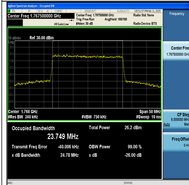
NTNV-n66-PC3-15-25-H-CP-256QAM-Outer_Full-Ant1- PASS
