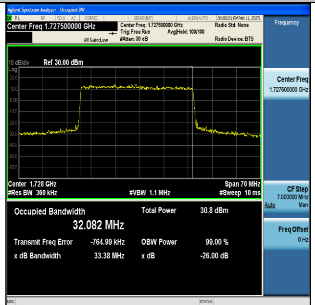
NTNV-n66-PC3-15-35-L-DFT-16QAM-Outer_Full-Ant1- PASS
