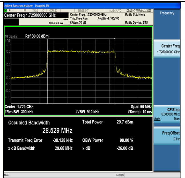
NTNV-n66-PC3-15-30-L-CP-16QAM-Outer_Full-Ant1-PASS
