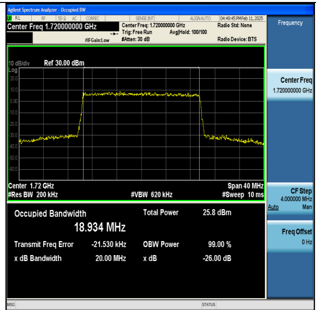
NTNV-n66-PC3-15-20-L-CP-256QAM-Outer_Full-Ant1- PASS
