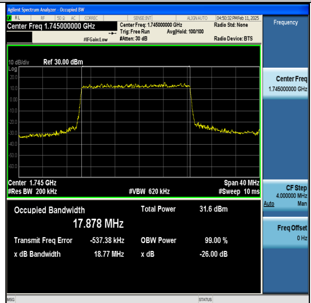
NTNV-n66-PC3-15-20-M-DFT-QPSK-Outer_Full-Ant1- PASS
