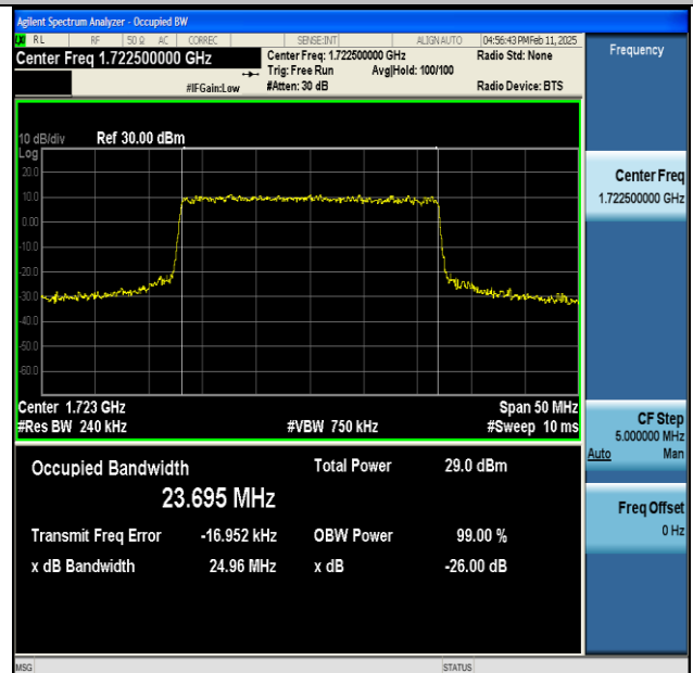
NTNV-n66-PC3-15-25-L-CP-64QAM-Outer_Full-Ant1-PASS
