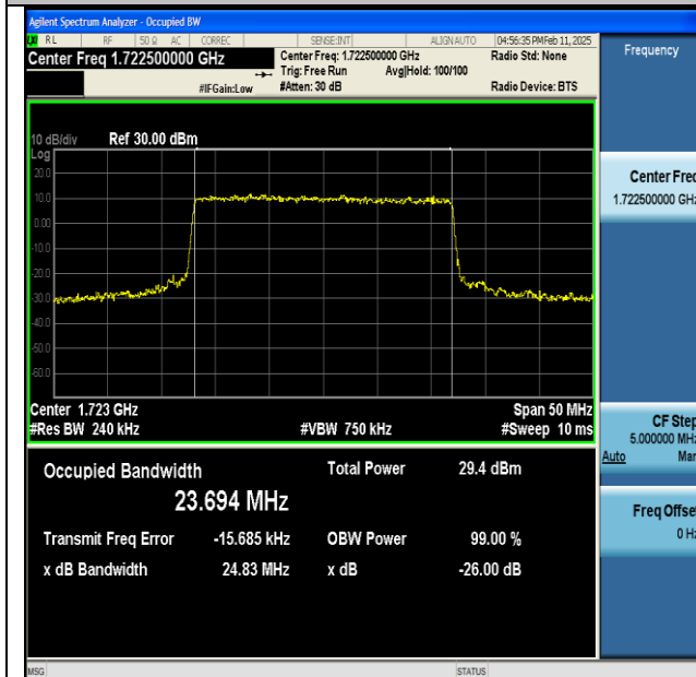
NTNV-n66-PC3-15-25-L-CP-16QAM-Outer_Full-Ant1-PASS
