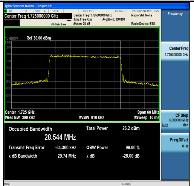
NTNV-n66-PC3-15-30-L-CP-256QAM-Outer_Full-Ant1-PASS
