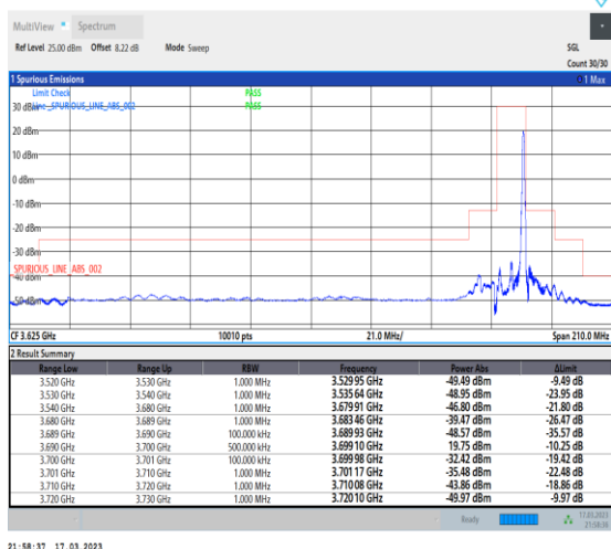
1-N48-PC3-30-10-H-5-CP-QPSK-Edge_1RB_Righ t-1@23-Ant0-1--PASS-see graph
