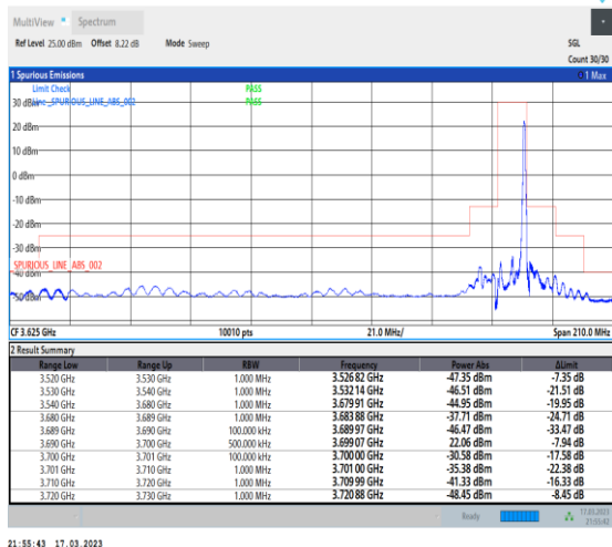
1-N48-PC3-30-10-H-2-DFT-PI2BPSK-Edge_1RB_Righ t-1@23-Ant0-1--PASS-see graph
