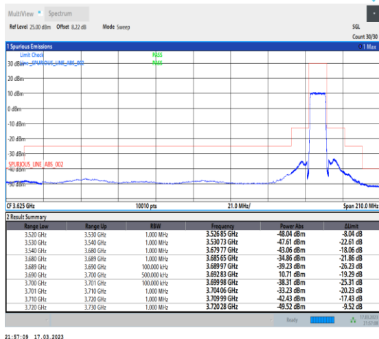
1-N48-PC3-30-10-H-3-DFT-PI2BPSK-Outer_Full-2 4@0-Ant0-1--PASS-see graph
