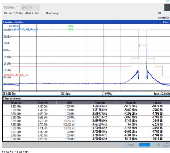
1-N48-PC3-30-10-H-6-CP-QPSK-Outer_Full-24@ 0-Ant0-1--PASS-see graph
