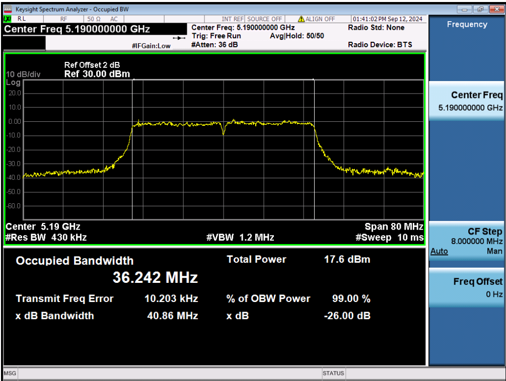
Figure 10: The plots of 26dB Bandwidth and 99% Bandwidth, 802.11n(HT40), 5190MHz
