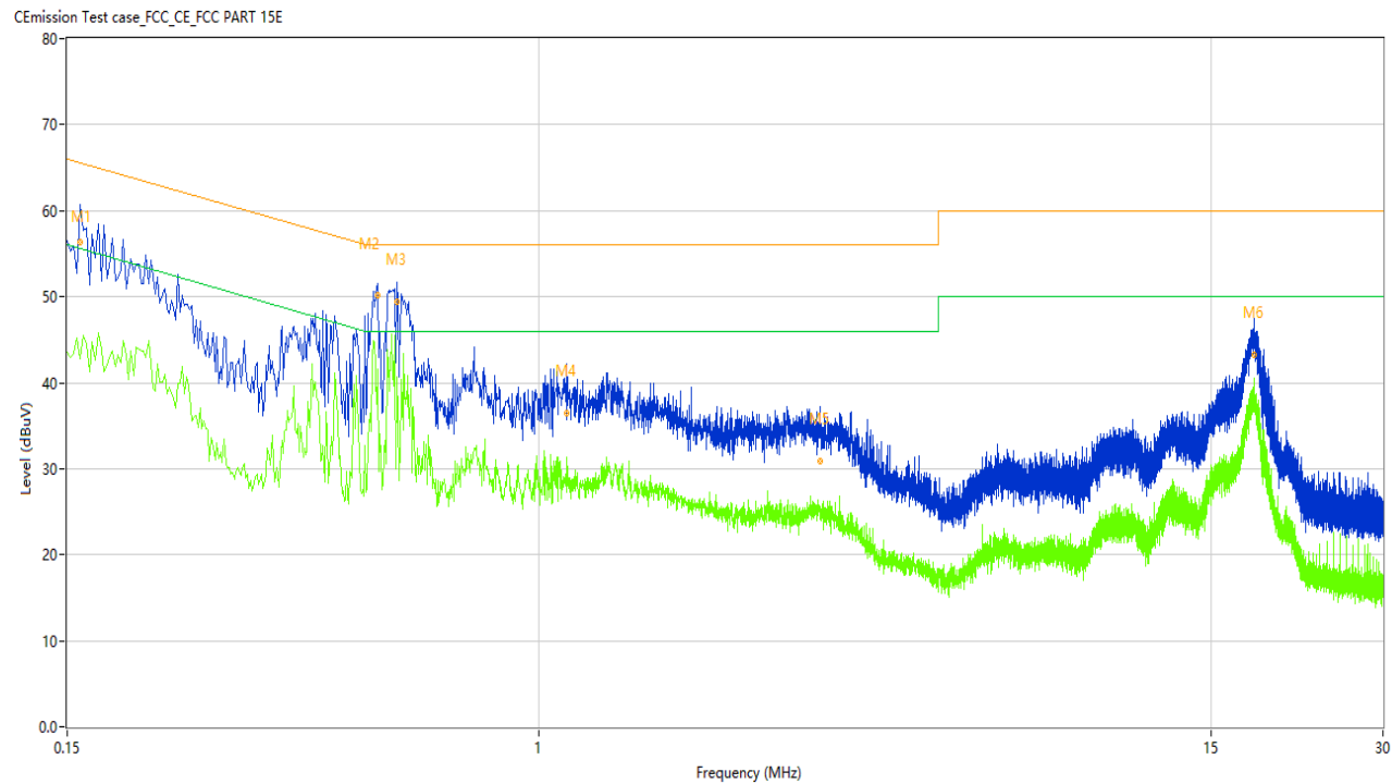
Figure 29: Conducted Emission on AC Mains, L Phase
