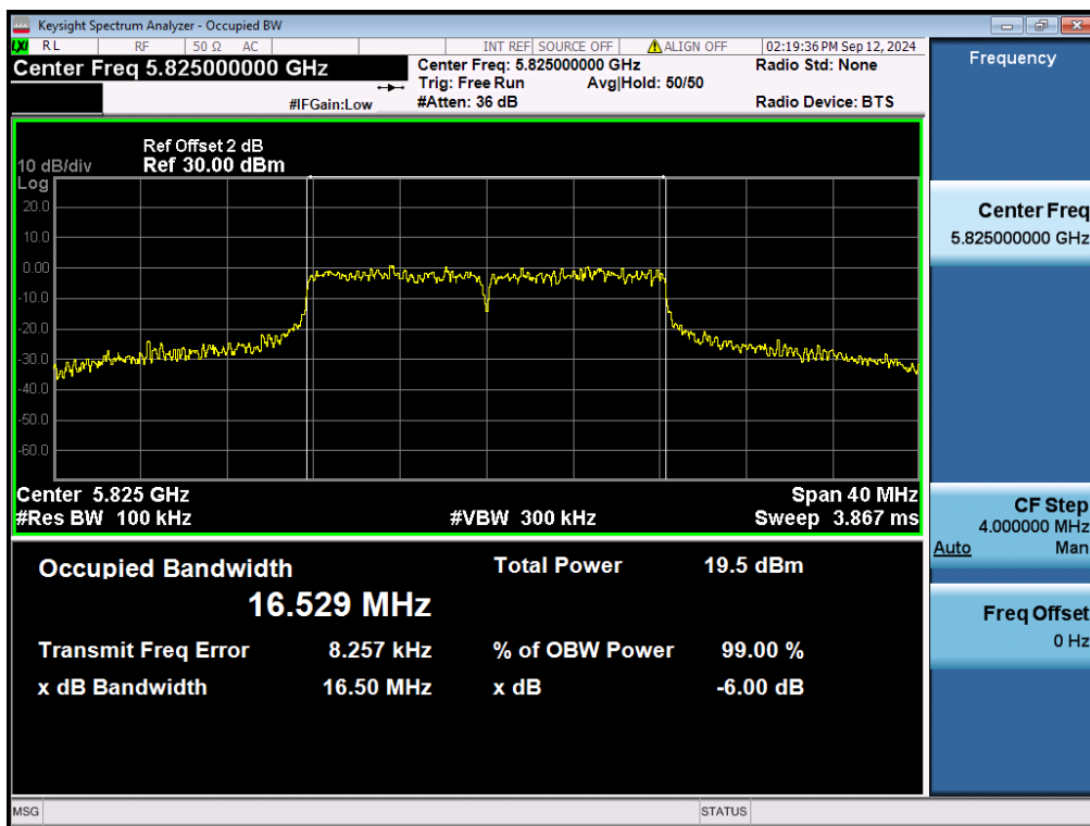
Figure 17: 802.11a, 5825MHz
