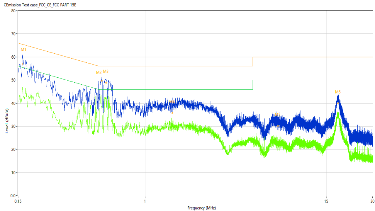
Figure 30: Conducted Emission on AC Mains, N Phase
