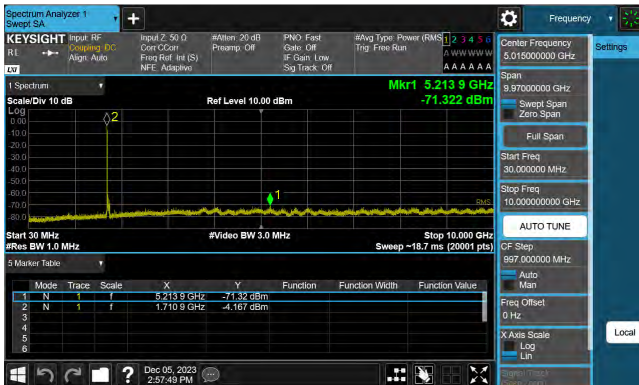
Sub6 n66. Conducted Spurious Plot_1 (346000ch_40 MHz_BPSK_ RB 1_1)
