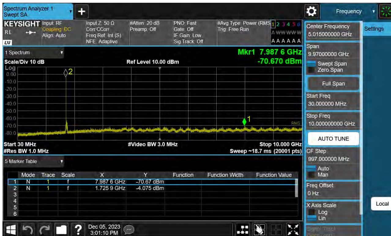
Sub6 n66. Conducted Spurious Plot_1 (349000ch_40 MHz_BPSK_ RB 1_1)
