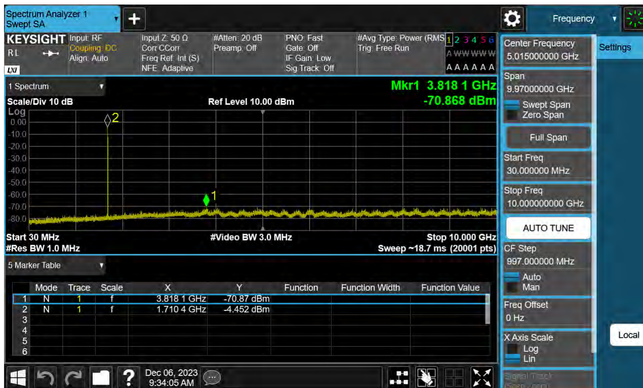
Sub6 n66. Conducted Spurious Plot_1 (342500ch_5 MHz_BPSK_ RB 1_1)
