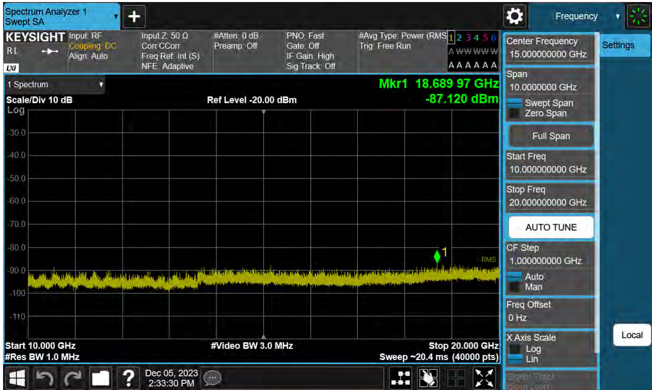
Sub6 n66. Conducted Spurious Plot_2 (354000ch_20 MHz_BPSK_ RB 1_1)
