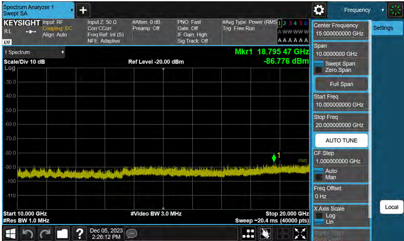
Sub6 n66. Conducted Spurious Plot_2 (354500ch_15 MHz_BPSK_ RB 1_1)
