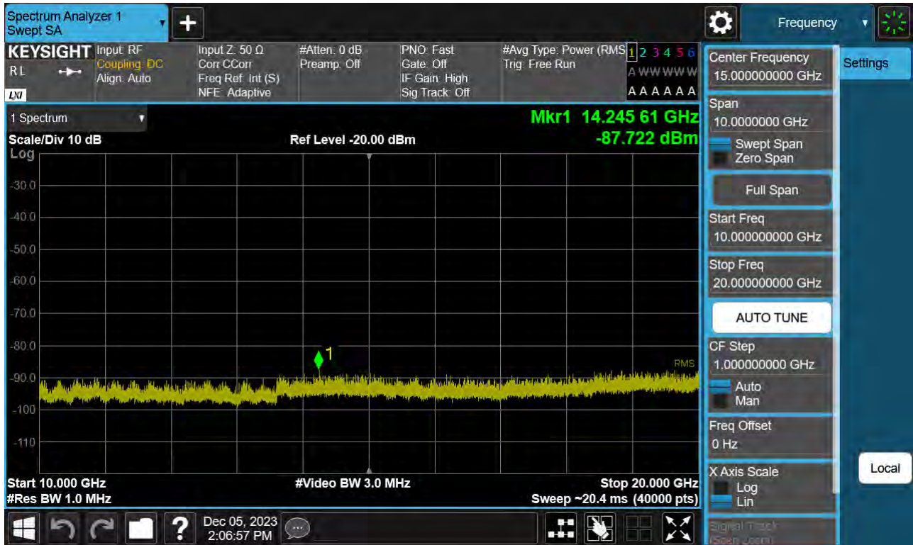
Sub6 n66. Conducted Spurious Plot_2 (355500ch_5 MHz_BPSK_ RB 1_1)
