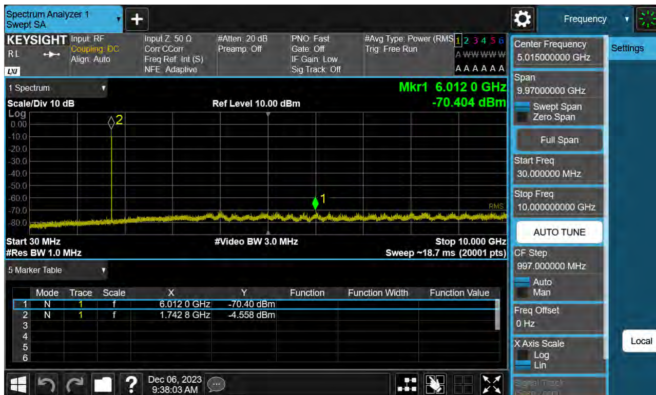
Sub6 n66. Conducted Spurious Plot_1 (349000ch_5 MHz_BPSK_ RB 1_1)
