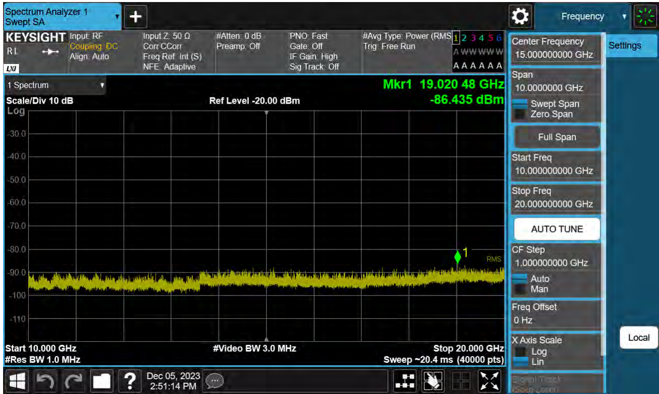
Sub6 n66. Conducted Spurious Plot_2 (349000ch_30 MHz_BPSK_ RB 1_1)
