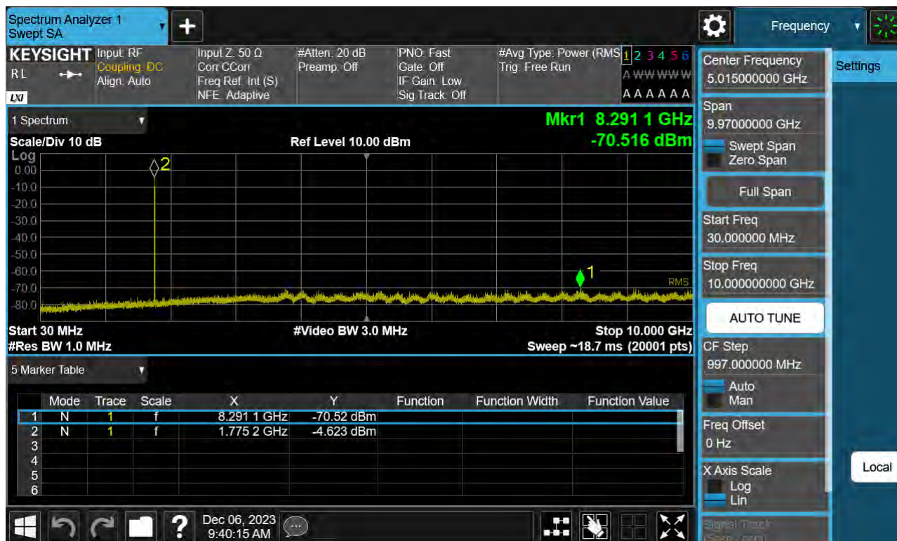
Sub6 n66. Conducted Spurious Plot_1 (355500ch_5 MHz_BPSK_ RB 1_1)
