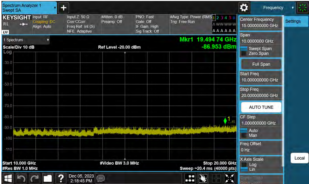
Sub6 n66. Conducted Spurious Plot_2 (355000ch_10 MHz_BPSK_ RB 1_1)
