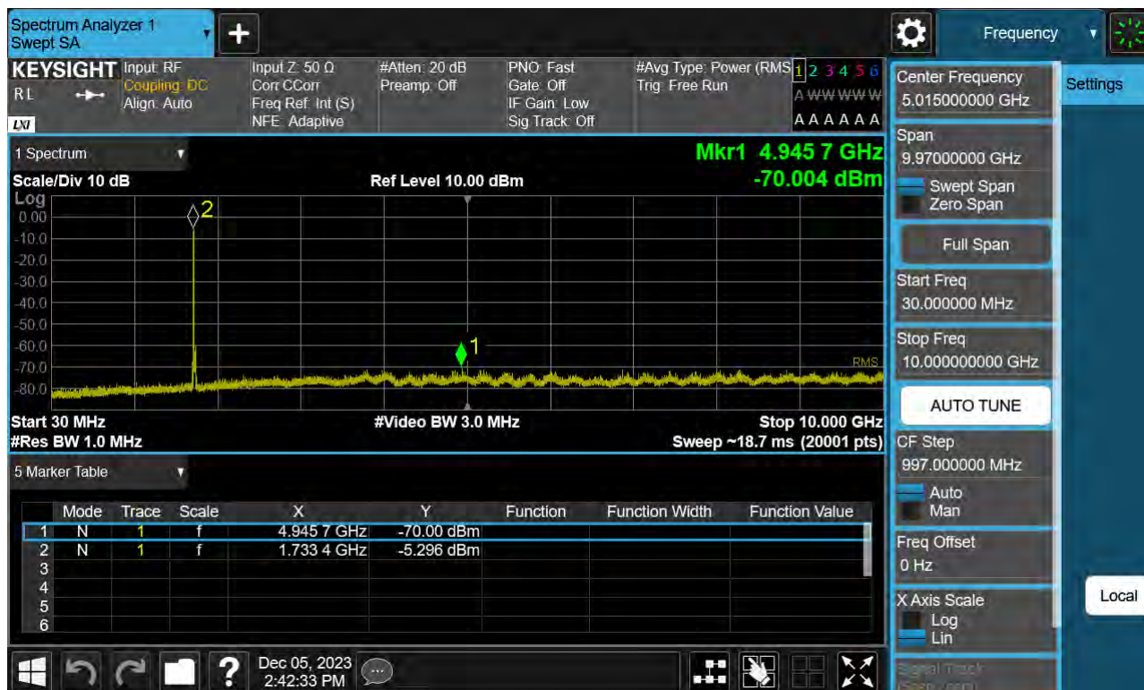
Sub6 n66. Conducted Spurious Plot_1 (349000ch_25 MHz_BPSK_ RB 1_1)
