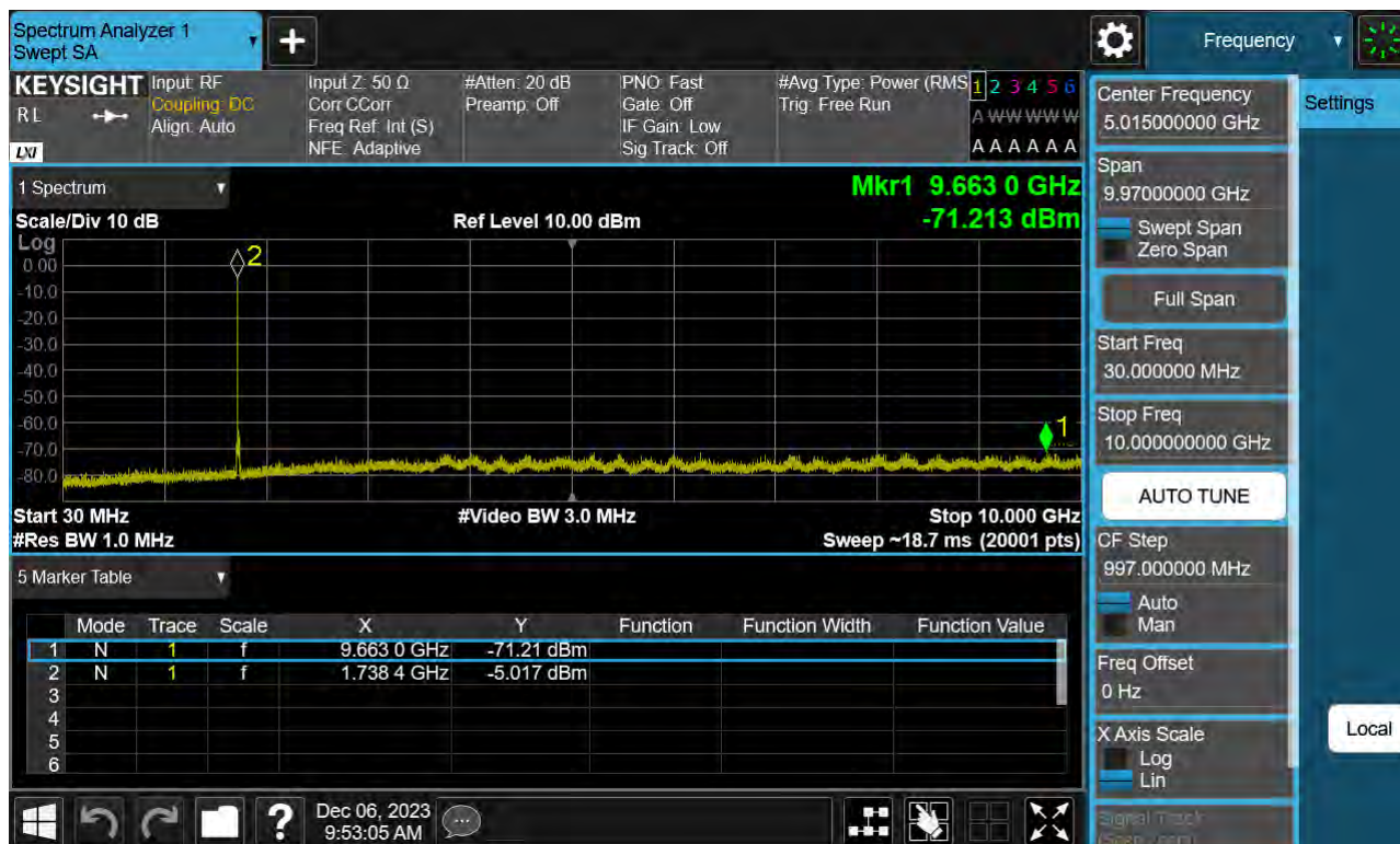
Sub6 n66. Conducted Spurious Plot_1 (349000ch_15 MHz_BPSK_ RB 1_1)
