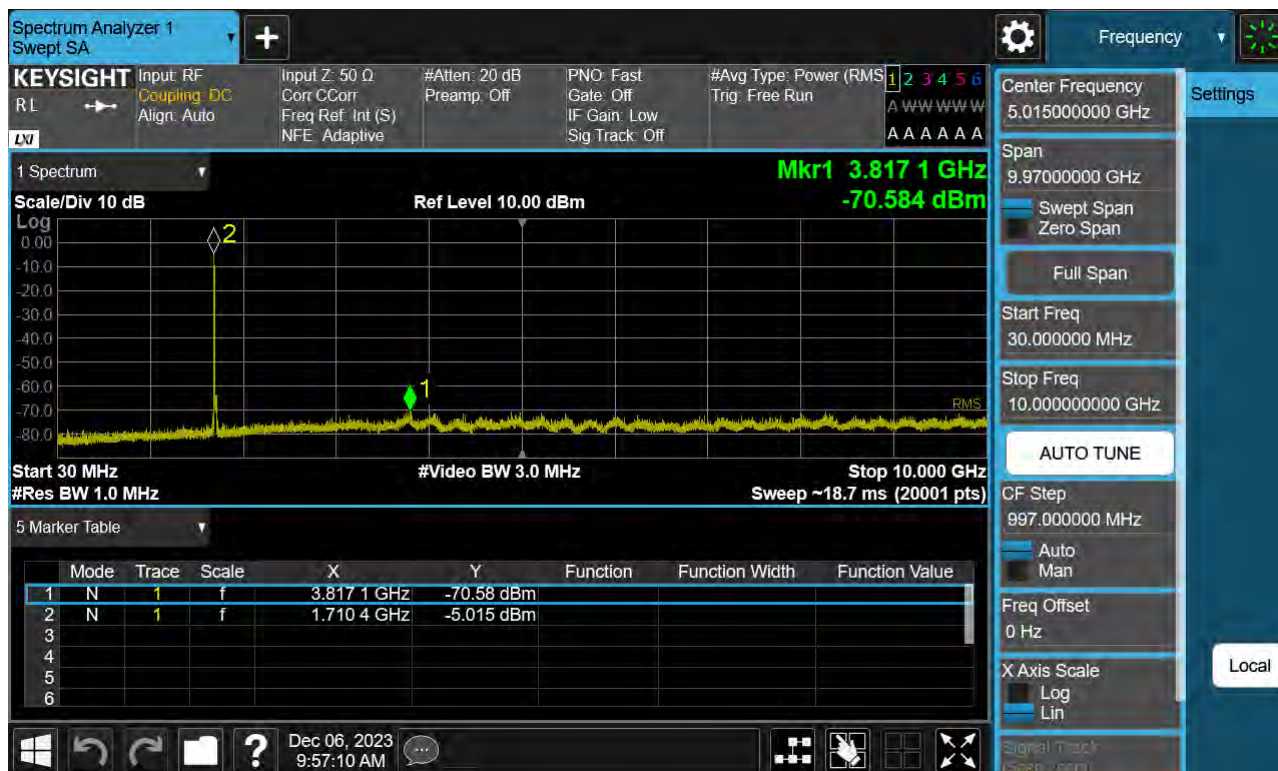
Sub6 n66. Conducted Spurious Plot_1 (344000ch_20 MHz_BPSK_ RB 1_1)
