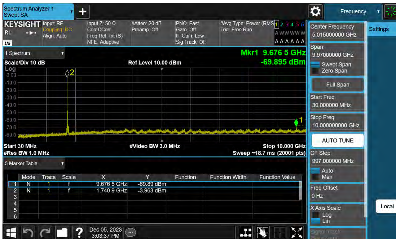
Sub6 n66. Conducted Spurious Plot_1 (352000ch_40 MHz_BPSK_ RB 1_1)
