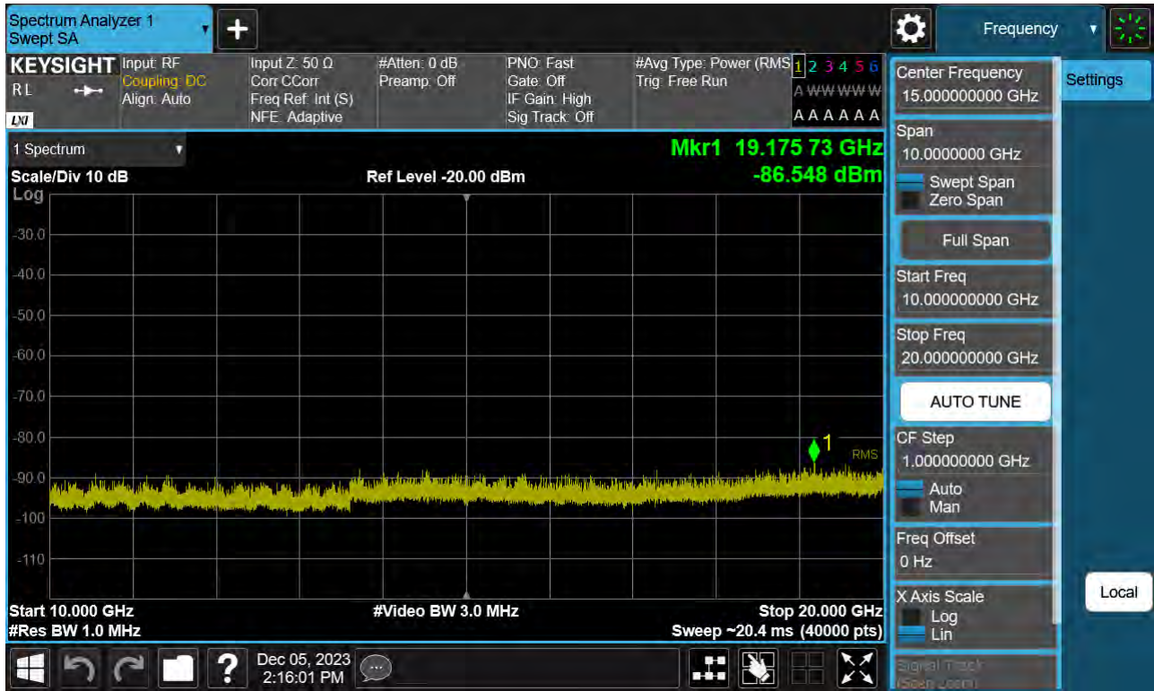
Sub6 n66. Conducted Spurious Plot_2 (349000ch_10 MHz_BPSK_ RB 1_1)
