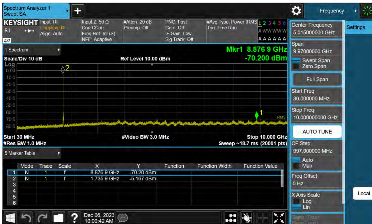
Sub6 n66. Conducted Spurious Plot_1 (349000ch_20 MHz_BPSK_ RB 1_1)
