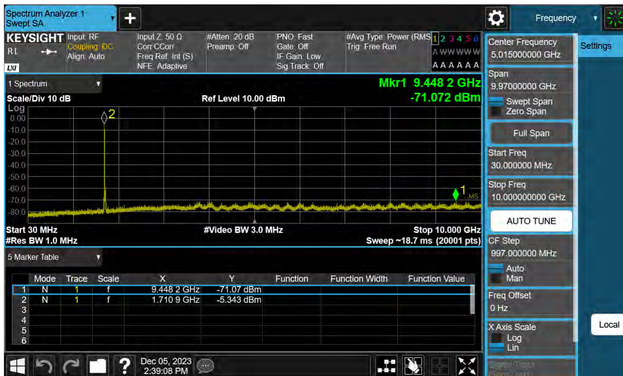
Sub6 n66. Conducted Spurious Plot_1 (344500ch_25 MHz_BPSK_ RB 1_1)
