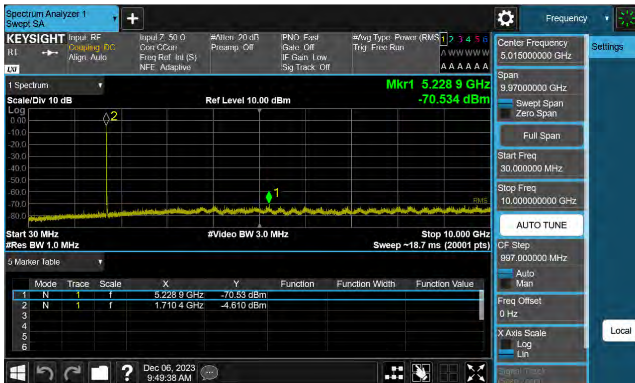
Sub6 n66. Conducted Spurious Plot_1 (343500ch_15 MHz_BPSK_ RB 1_1)
