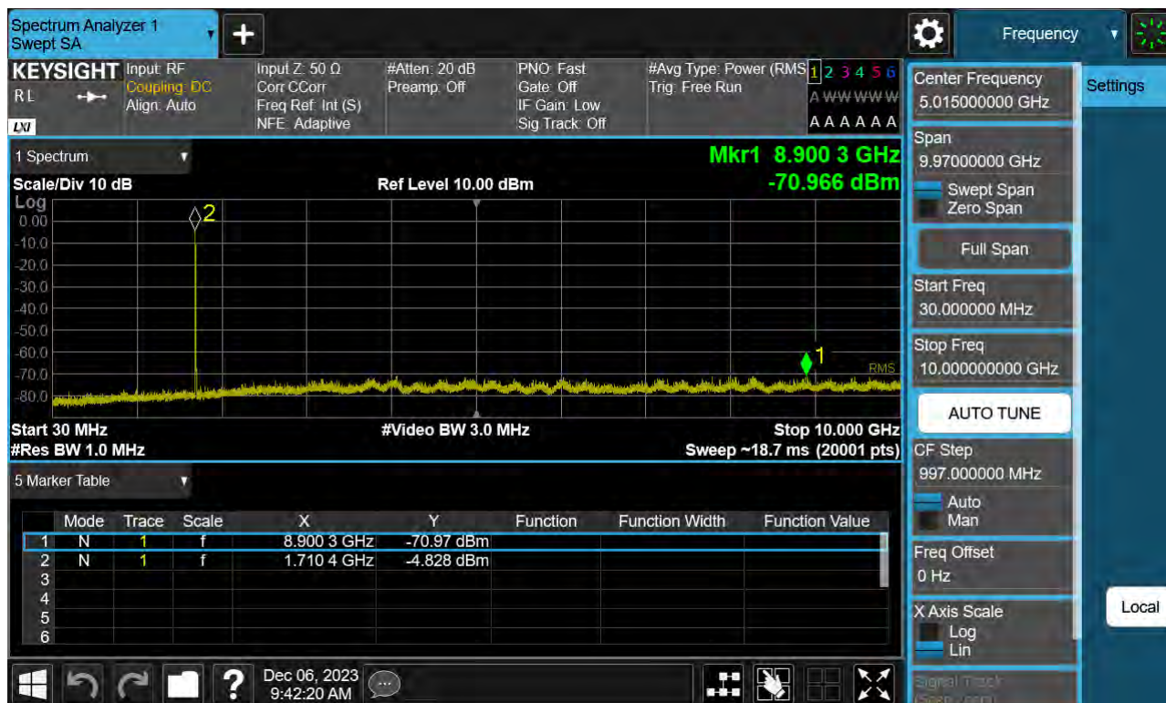
Sub6 n66. Conducted Spurious Plot_1 (343000ch_10 MHz_BPSK_ RB 1_1)
