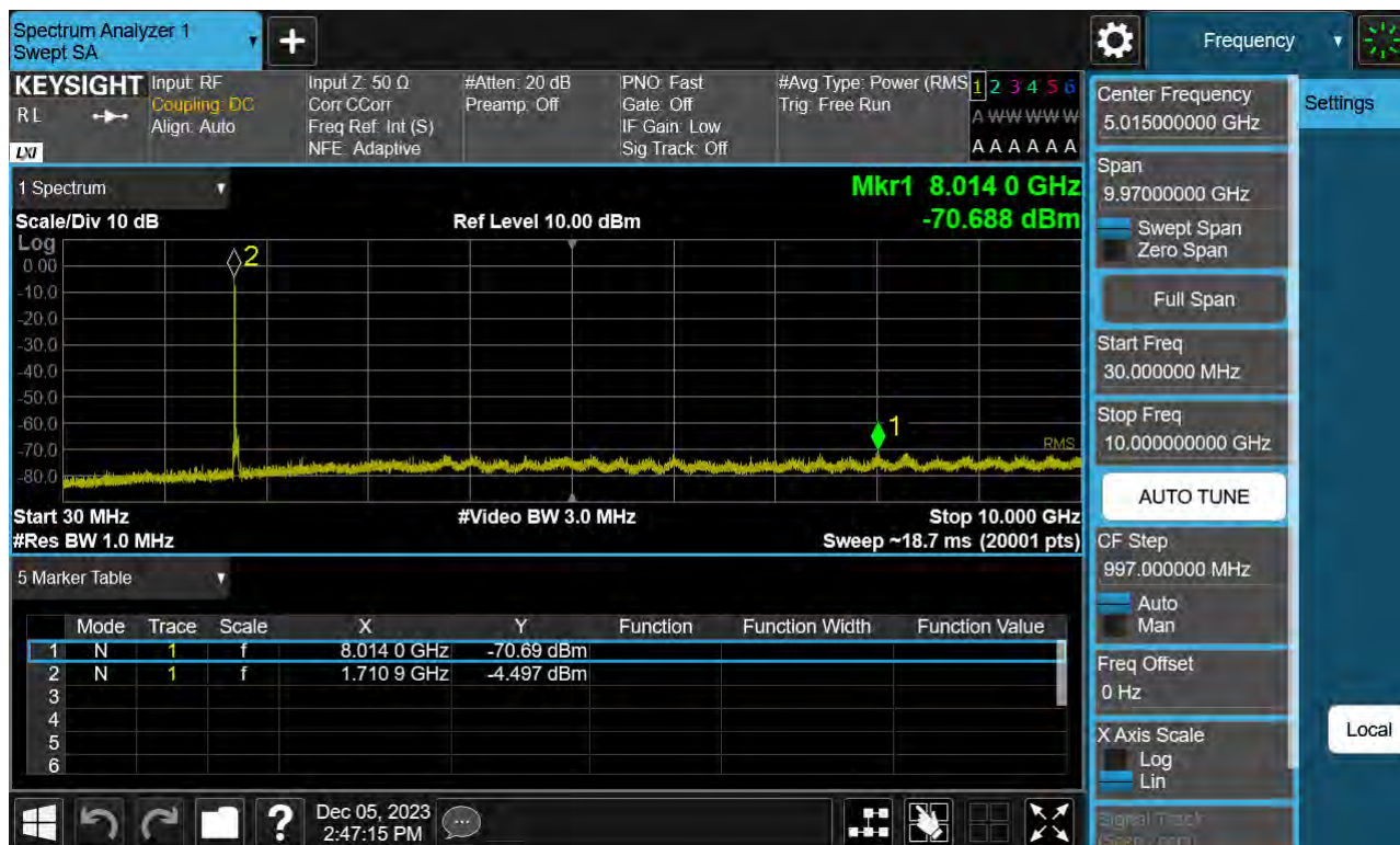
Sub6 n66. Conducted Spurious Plot_1 (345000ch_30 MHz_BPSK_ RB 1_1)
