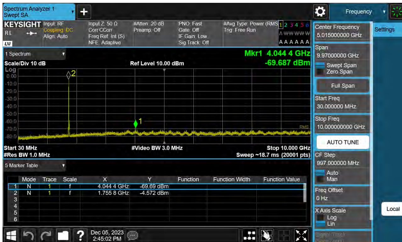
Sub6 n66. Conducted Spurious Plot_1 (353500ch_25 MHz_BPSK_ RB 1_1)
