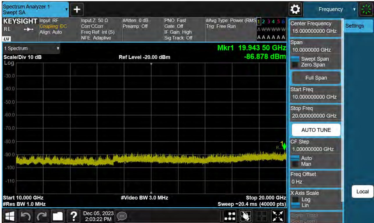
Sub6 n66. Conducted Spurious Plot_2 (349000ch_5 MHz_BPSK_ RB 1_1)
