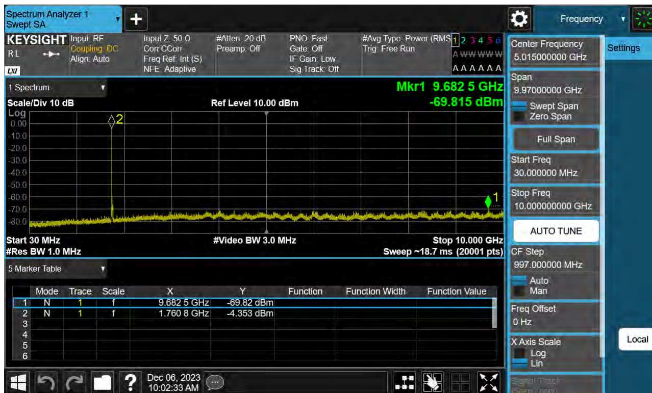
Sub6 n66. Conducted Spurious Plot_1 (354000ch_20 MHz_BPSK_ RB 1_1)
