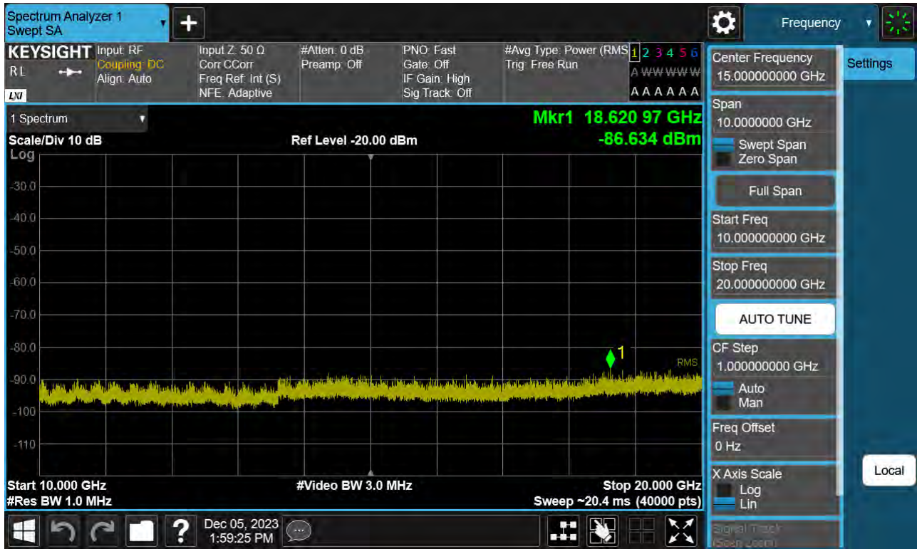
Sub6 n66. Conducted Spurious Plot_2 (342500ch_5 MHz_BPSK_ RB 1_1)
