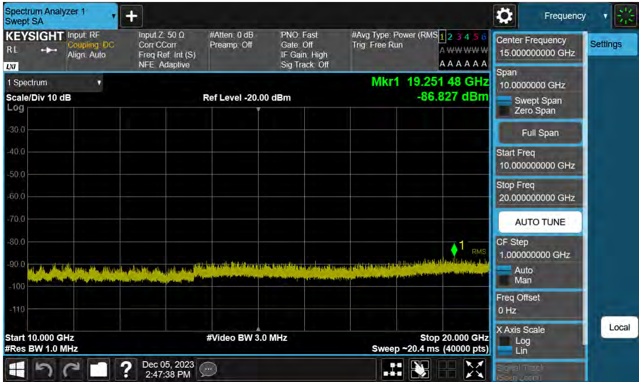
Sub6 n66. Conducted Spurious Plot_2 (345000ch_30 MHz_BPSK_ RB 1_1)
