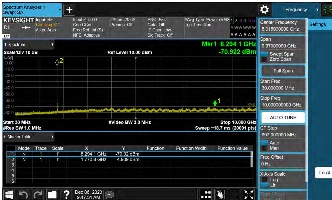
Sub6 n66. Conducted Spurious Plot_1 (355000ch_10 MHz_BPSK_ RB 1_1)
