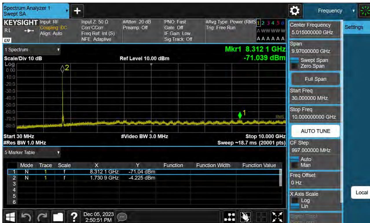
Sub6 n66. Conducted Spurious Plot_1 (349000ch_30 MHz_BPSK_ RB 1_1)
