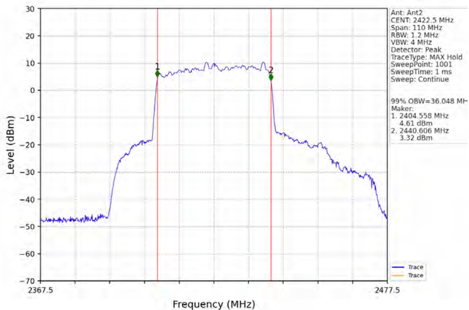
40M_LCH_2422.5MHz_Ant2_NTNV
