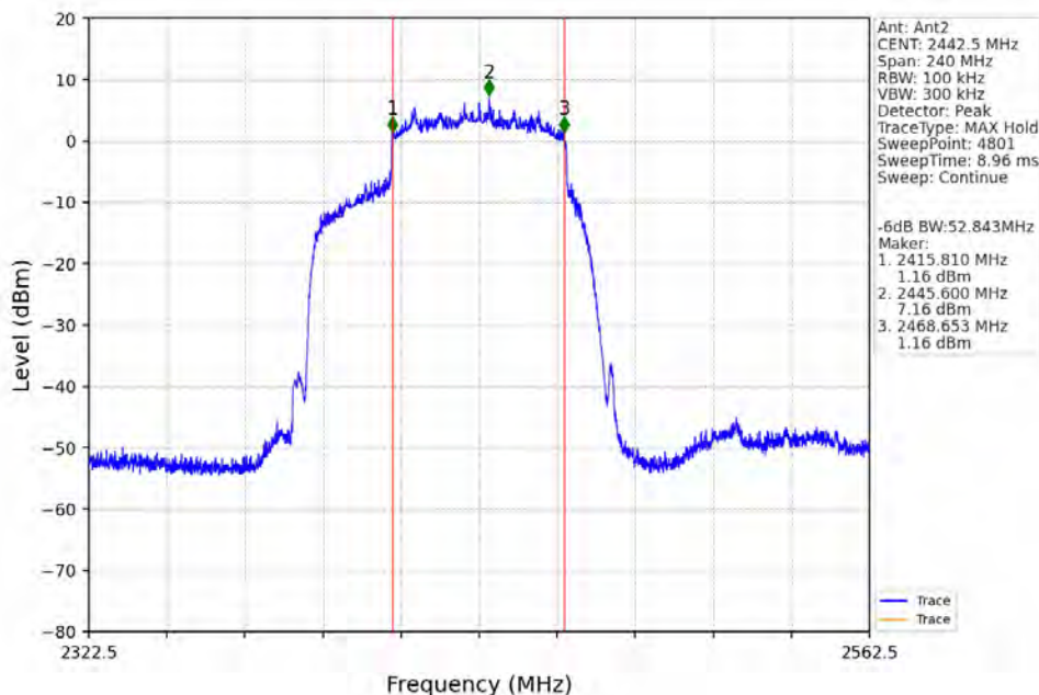
60M_HCH_2442.5MHz_Ant2_NTNV
