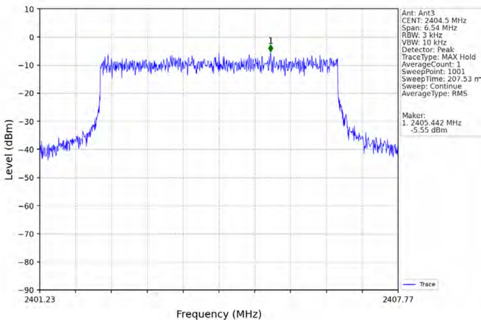
5M_LCH_2404.5MHz_Ant3_NTNV
