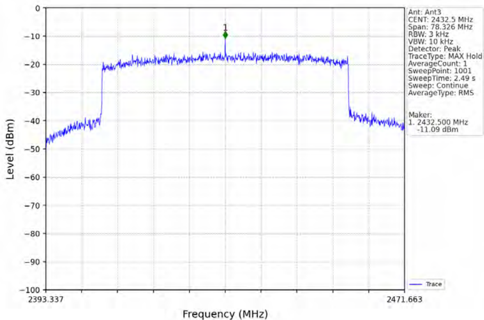
60M_LCH_2432.5MHz_Ant3_NTNV
