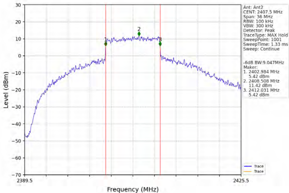
10M_LCH_2407.5MHz_Ant2_NTNV
