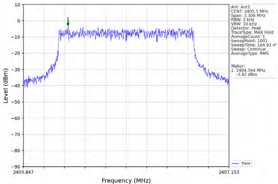
3M_LCH_2405.5MHz_Ant2_NTNV
