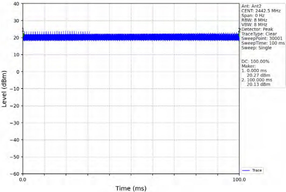
60M_HCH_2442.5MHz_Ant2_NTNV
