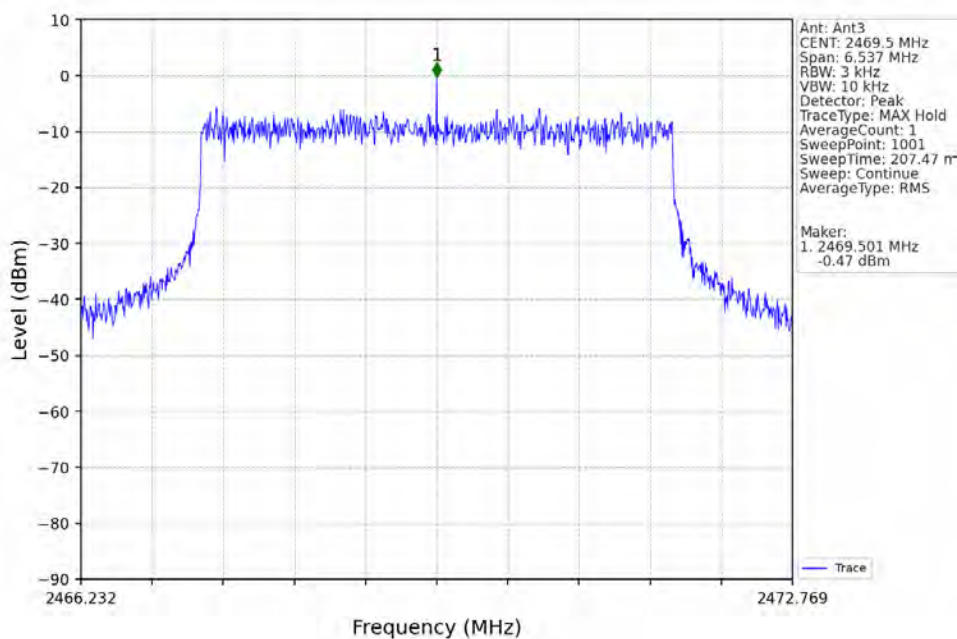
5M_HCH_2469.5MHz_Ant3_NTNV
