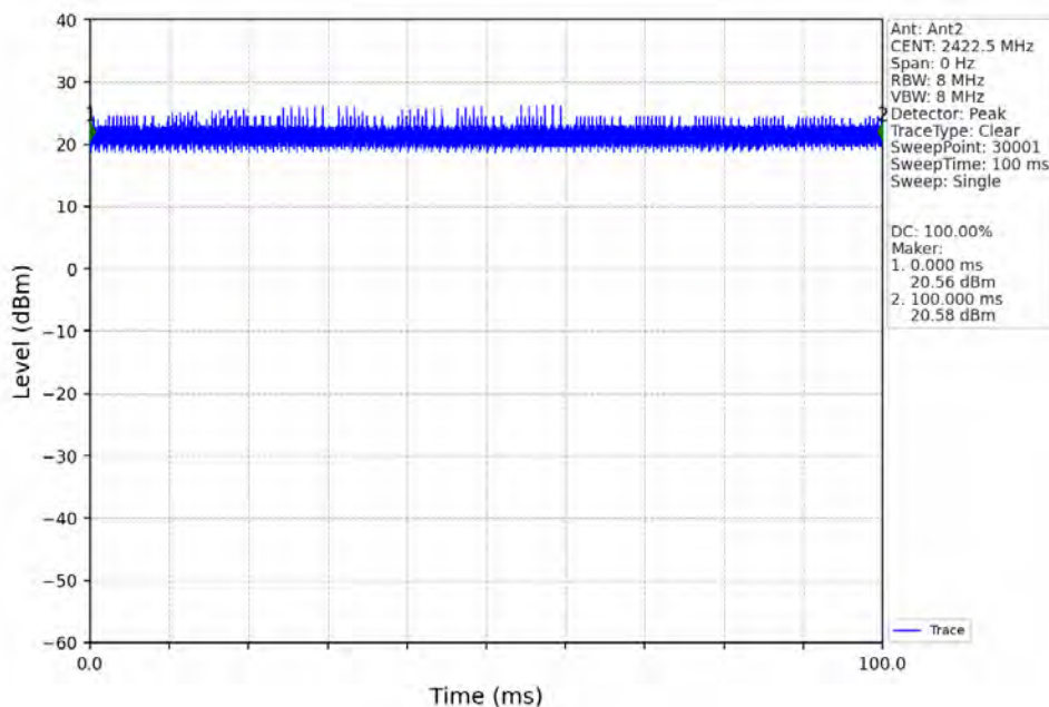
40M_LCH_2422.5MHz_Ant2_NTNV
