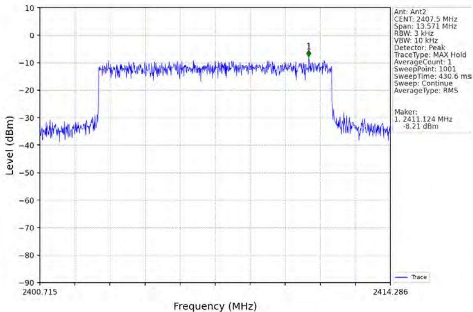
10M_LCH_2407.5MHz_Ant2_NTNV
