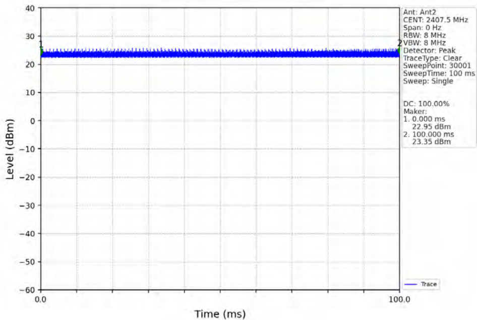
10M_LCH_2407.5MHz_Ant2_NTNV
