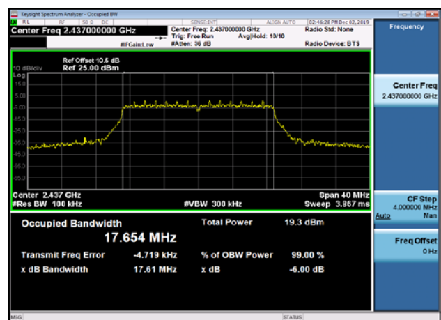
6dB Bandwidth-802.11n(HT20),2437MHz
