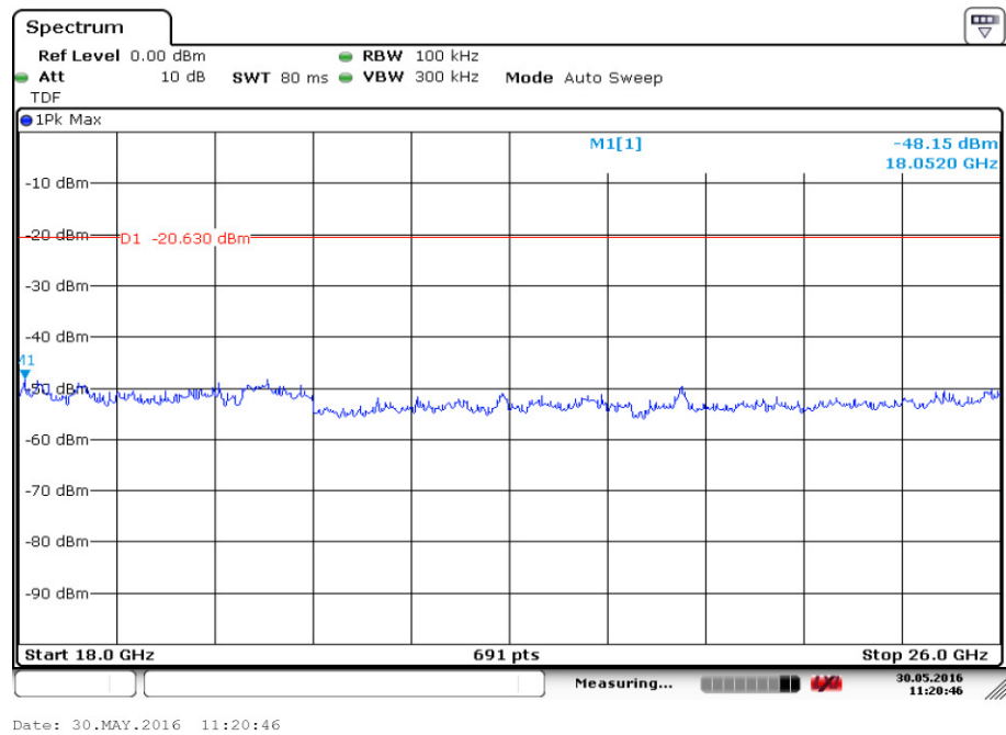
Fig.12. Conducted Spurious Emission (All channels, 18 GHz-26 GHz)
