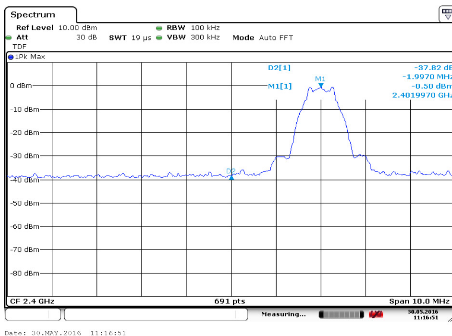
Fig.1. Frequency Band Edges: GFSK, 2402 MHz, Hopping Off
