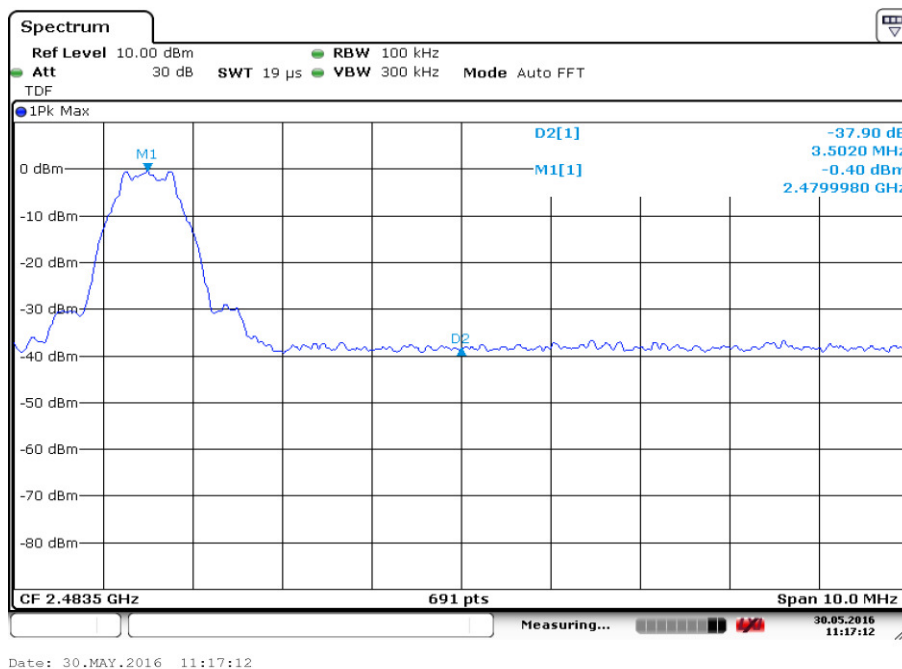
Fig.2. Frequency Band Edges: GFSK, 2480 MHz, Hopping Off
