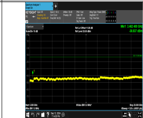
Band4_3MHz_16QAM_20175_1RB#0_3000-20000_3000-20000
