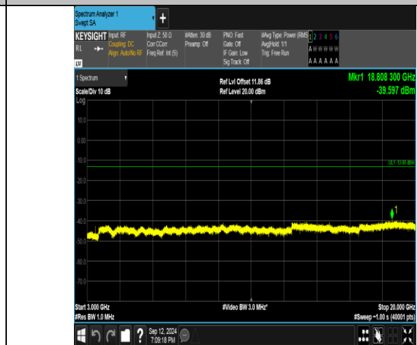
Band4_3MHz_16QAM_19965_1RB#0_3000-20000_3000-20000
