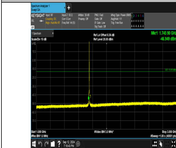
Band4_3MHz_16QAM_20385_1RB#0_1000-3000_1000-3000
