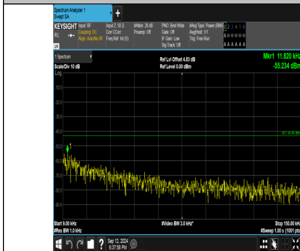
Band4_1.4MHz_QPSK_20393_6RB#0_0.009~0.15_0.009~0.15
