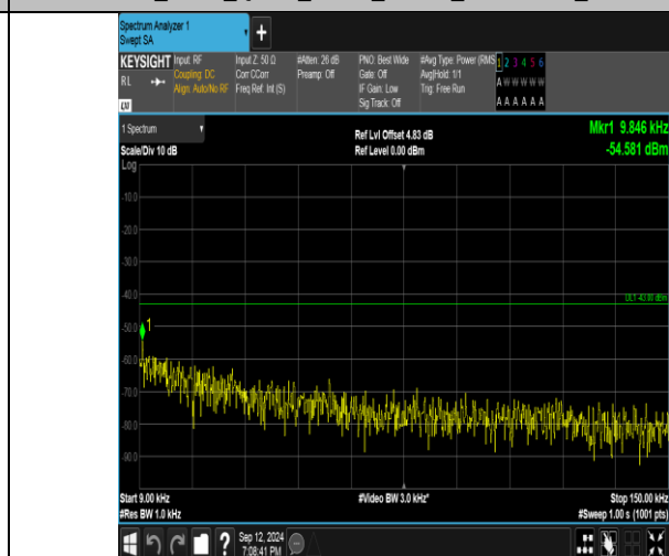
Band4_3MHz_16QAM_19965_1RB#0_0.009~0.15_0.009~0.15
