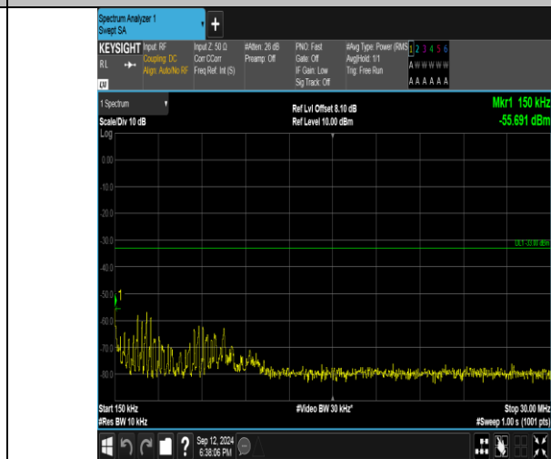
Band4_1.4MHz_QPSK_20393_6RB#0_0.15~30_0.15~30
