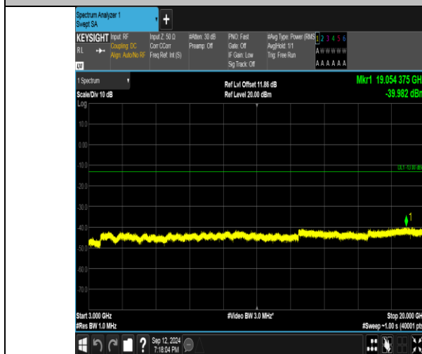
Band4_3MHz_QPSK_20385_1RB#0_3000~20000_3000~20000
