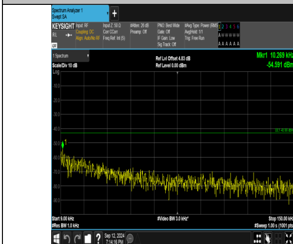
Band4_3MHz_QPSK_20175_1RB#14_0.009-0.15_0.009-0.15
