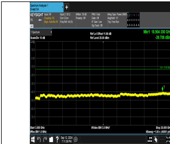
Band4_3MHz_QPSK_19965_15RB#0_3000~20000_3000~20000
