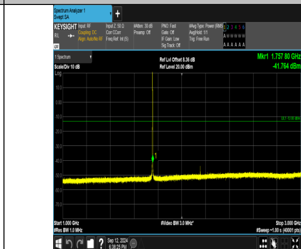
Band4_1.4MHz_QPSK_20393_6RB#0_1000~3000_1000~3000
