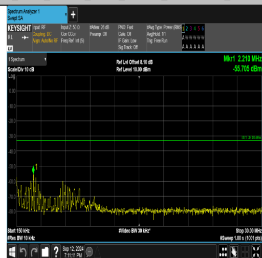
Band4_3MHz_QPSK_19965_15RB#0_0.15~30_0.15~30
