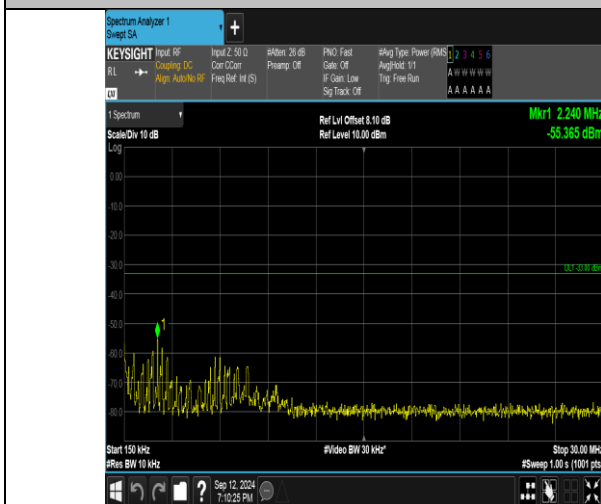
Band4_3MHz_16QAM_19965_1RB#14_0.15~30_0.15~30
