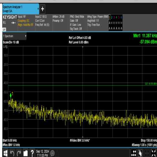
Band4_3MHz_QPSK_19965_15RB#0_0.009~0.15_0.009~0.15
