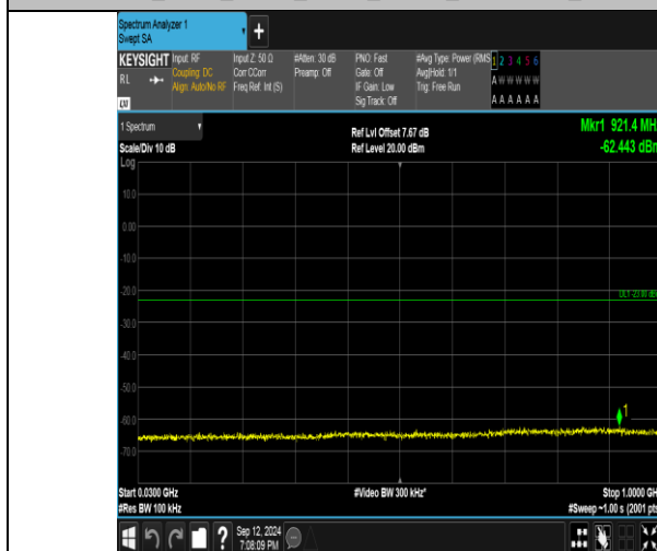
Band4_3MHz_QPSK_19965_1RB#0_30~1000_30~1000
