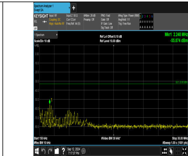
Band4_3MHz_QPSK_20385_1RB#0_0.15~30_0.15~30
