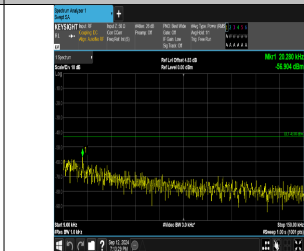
Band4_3MHz_16QAM_20175_1RB#0_0.009~0.15_0.009~0.15
