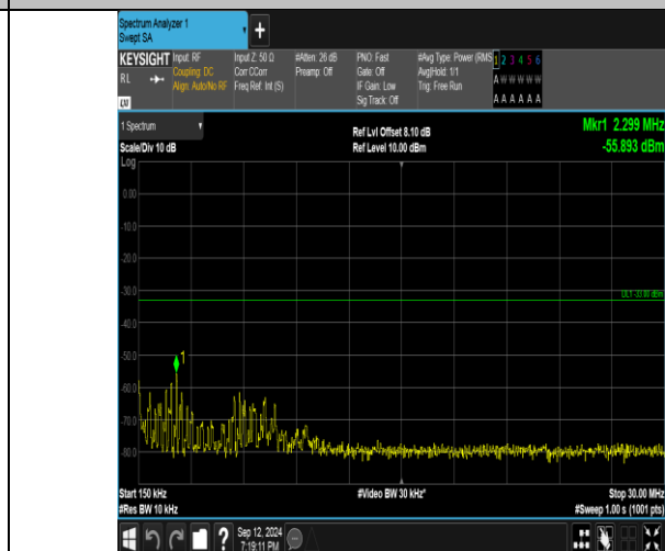
Band4_3MHz_QPSK_20385_1RB#14_0.15-30_0.15-30
