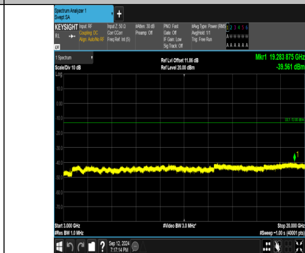
Band4_3MHz_16QAM_20175_15RB#0_3000~20000_3000~20000
