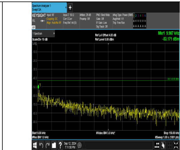
Band4_3MHz_16QAM_19965_15RB#0_0.009~0.15_0.009~0.15
