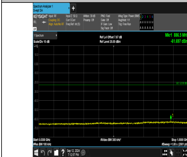
Band4_3MHz_QPSK_20175_1RB#0_30~1000_30~1000
