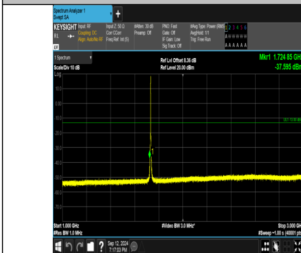
Band4_3MHz_16QAM_20175_15RB#0_1000~3000_1000~3000
