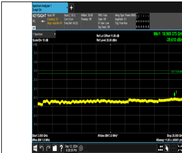
Band4_1.4MHz_QPSK_20393_6RB#0_3000~20000_3000~20000
