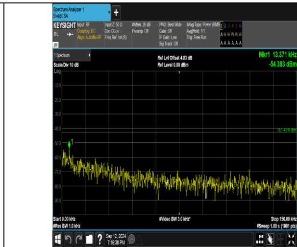
Band4_3MHz_16QAM_20175_15RB#0_0.009~0.15_0.009~0.15
