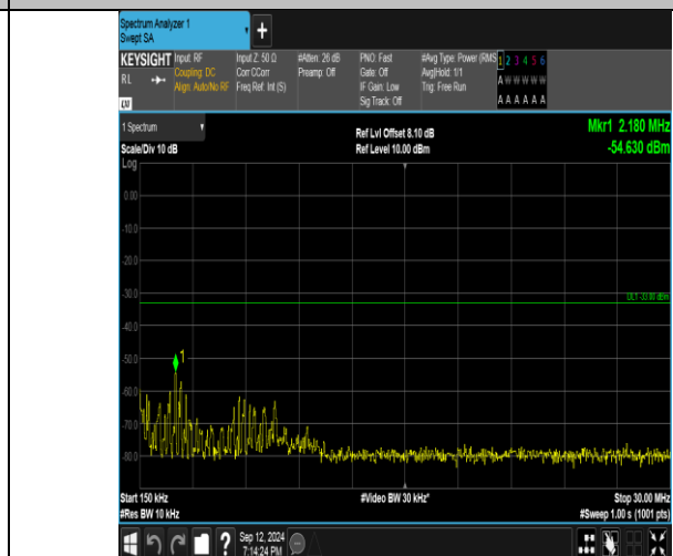
Band4_3MHz_QPSK_20175_1RB#14_0.15-30_0.15-30
