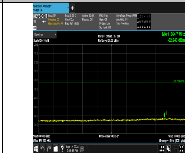
Band4_3MHz_16QAM_20175_15RB#0_30~1000_30~1000
