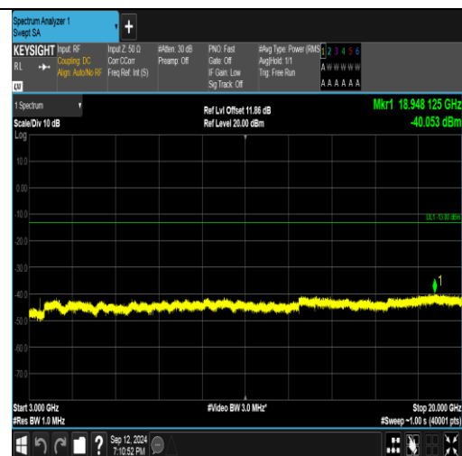
Band4_3MHz_16QAM_19965_1RB#14_3000~20000_3000~20000
