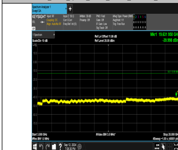
Band4_3MHz_QPSK_19965_1RB#0_3000~20000_3000~20000
