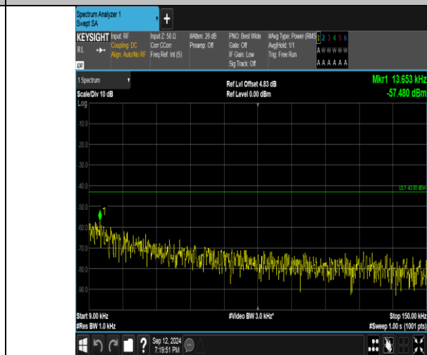
Band4_3MHz_16QAM_20385_1RB#14_0.009~0.15_0.009~0.15
