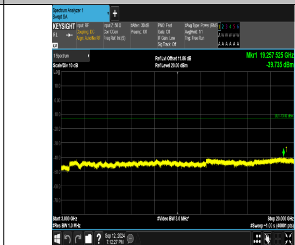
Band4_3MHz_16QAM_19965_15RB#0_3000~20000_3000~20000
