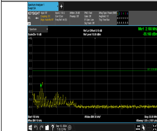
Band4_3MHz_16QAM_20175_1RB#14_0.15~30_0.15~30
