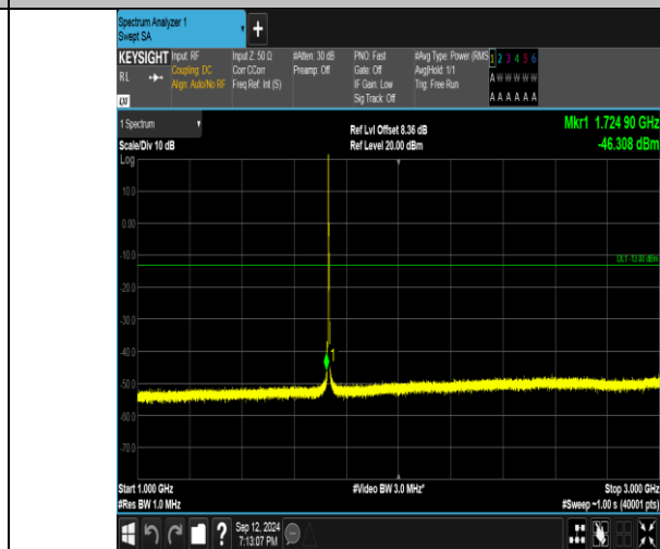
Band4_3MHz_QPSK_20175_1RB#0_1000~3000_1000~3000
