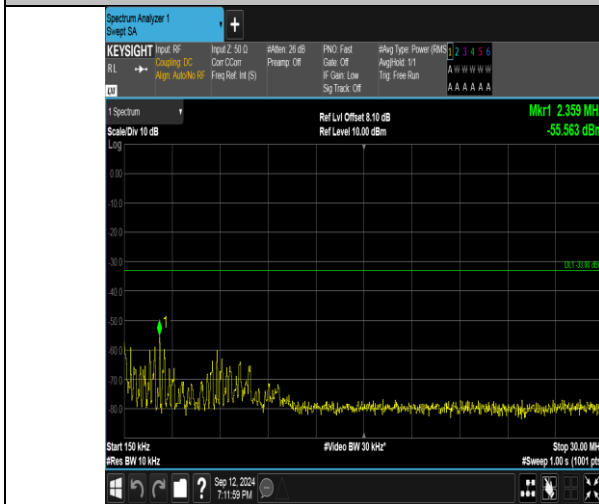
Band4_3MHz_16QAM_19965_15RB#0_0.15~30_0.15~30
