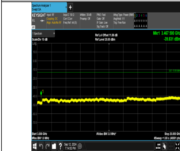
Band4_3MHz_QPSK_20175_1RB#14_3000~20000_3000~20000
