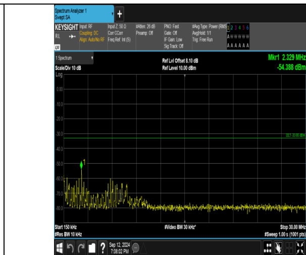
Band4_3MHz_QPSK_19965_1RB#0_0.15~30_0.15~30
