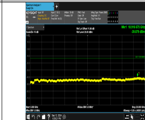
Band4_1.4MHz_16QAM_20393_6RB#0_3000~20000_3000~20000
