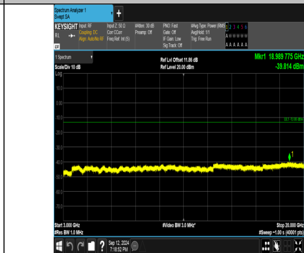
Band4_3MHz_16QAM_20385_1RB#0_3000-20000_3000-20000
