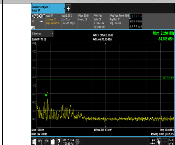
Band4_3MHz_QPSK_19965_1RB#14_0.15-30_0.15-30
