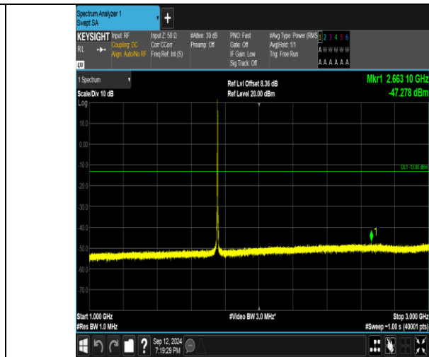
Band4_3MHz_QPSK_20385_1RB#14_1000~3000_1000~3000
