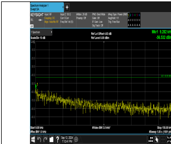
Band4_3MHz_QPSK_20175_1RB#0_0.009~0.15_0.009~0.15
