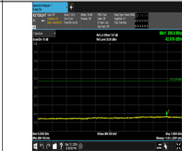
Band4_1.4MHz_16QAM_20393_6RB#0_30~1000_30~1000
