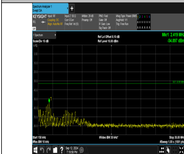
Band4_3MHz_16QAM_20385_1RB#14_0.15~30_0.15~30
