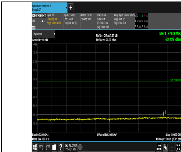
Band4_3MHz_QPSK_20175_1RB#14_30~1000_30~1000
