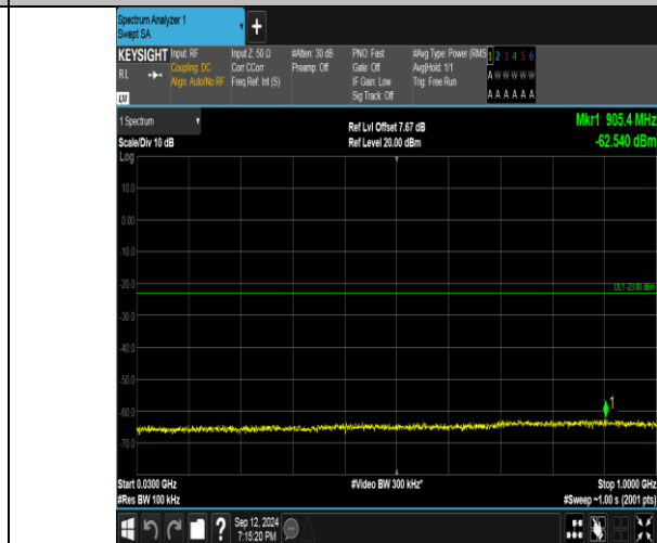
Band4_3MHz_16QAM_20175_1RB#14_30~1000_30~1000
