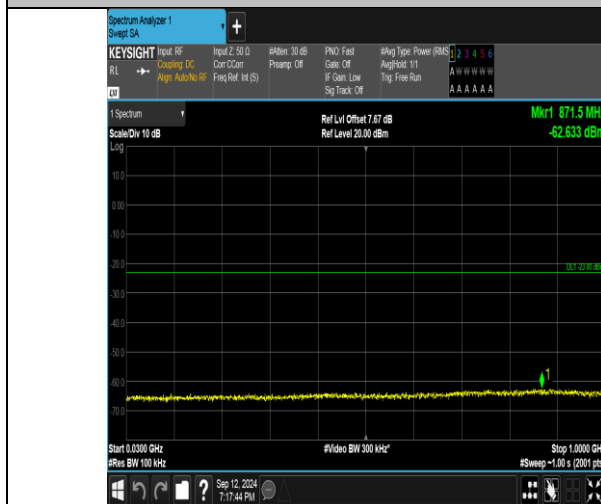
Band4_3MHz_QPSK_20385_1RB#0_30~1000_30~1000
