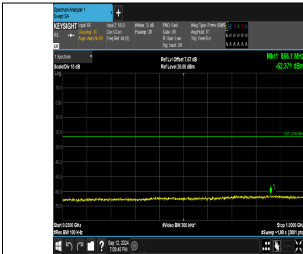
Band4_3MHz_QPSK_19965_1RB#14_30~1000_30~1000
