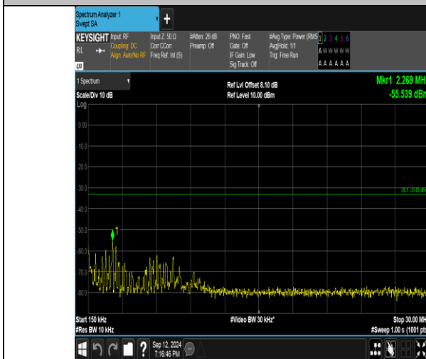
Band4_3MHz_16QAM_20175_15RB#0_0.15~30_0.15~30
