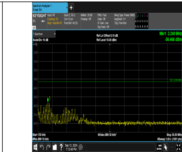
Band4_3MHz_QPSK_20175_1RB#0_0.15~30_0.15~30
