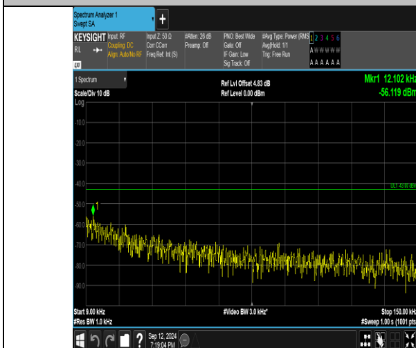
Band4_3MHz_QPSK_20385_1RB#14_0.009-0.15_0.009-0.15
