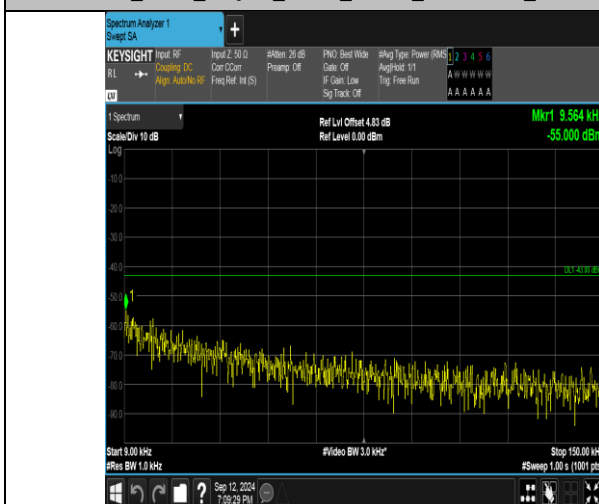
Band4_3MHz_QPSK_19965_1RB#14_0.009-0.15_0.009-0.15
