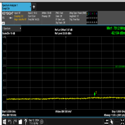
Band4_3MHz_QPSK_19965_15RB#0_30~1000_30~1000
