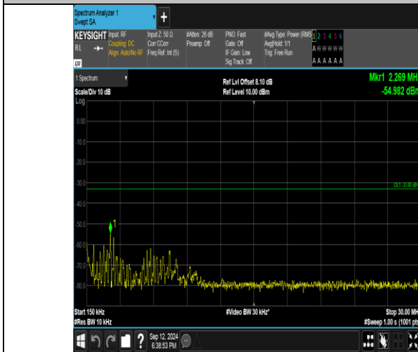
Band4_1.4MHz_16QAM_20393_6RB#0_0.15~30_0.15~30
