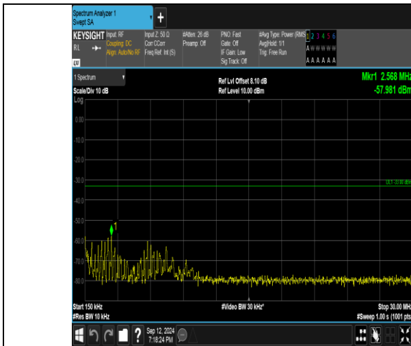
Band4_3MHz_16QAM_20385_1RB#0_0.15-30_0.15-30
