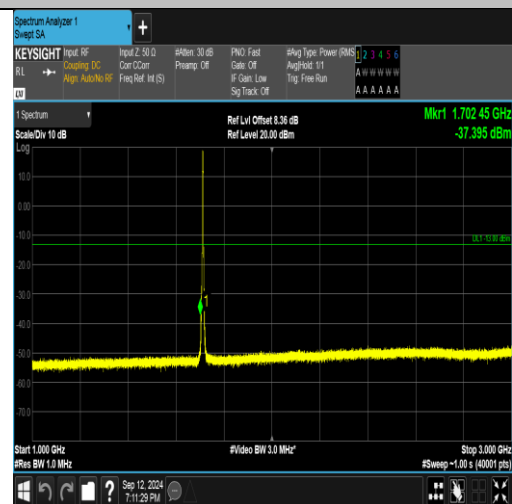
Band4_3MHz_QPSK_19965_15RB#0_1000~3000_1000~3000
