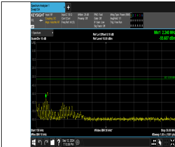
Band4_3MHz_16QAM_20175_1RB#0_0.15-30_0.15-30
