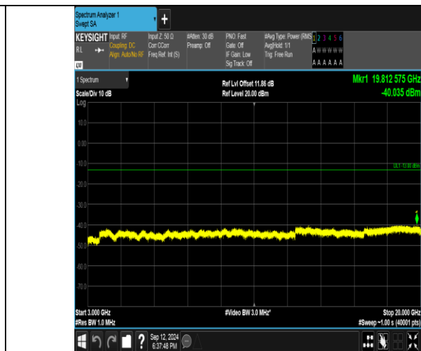
Band4_1.4MHz_16QAM_20393_1RB#5_3000~20000_3000~20000
