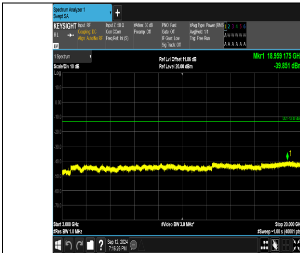
Band4_3MHz_QPSK_20175_15RB#0_3000~20000_3000~20000
