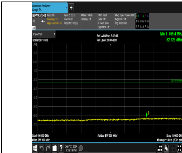
Band4_3MHz_QPSK_20385_1RB#14_30~1000_30~1000
