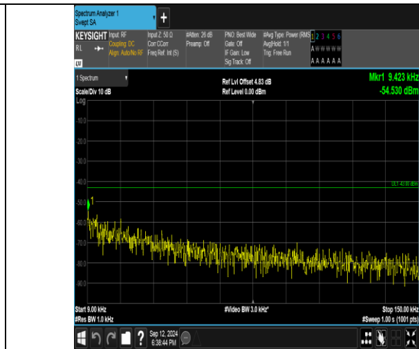
Band4_1.4MHz_16QAM_20393_6RB#0_0.009~0.15_0.009~0.15
