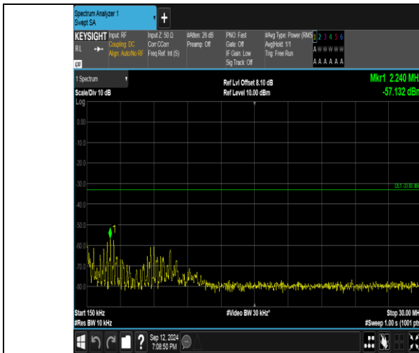
Band4_3MHz_16QAM_19965_1RB#0_0.15-30_0.15-30
