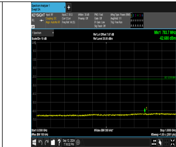
Band4_3MHz_16QAM_20385_1RB#0_30-1000_30-1000
