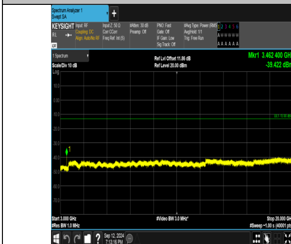
Band4_3MHz_QPSK_20175_1RB#0_3000~20000_3000~20000
