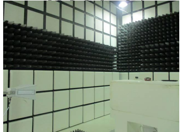
Part_15_249_SRD_2.4G_Radiated_Setup
