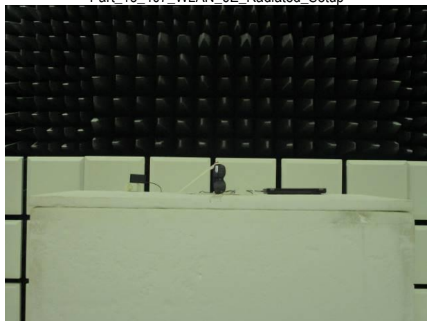
Part_15_407_WLAN_6E_Radiated_Setup
