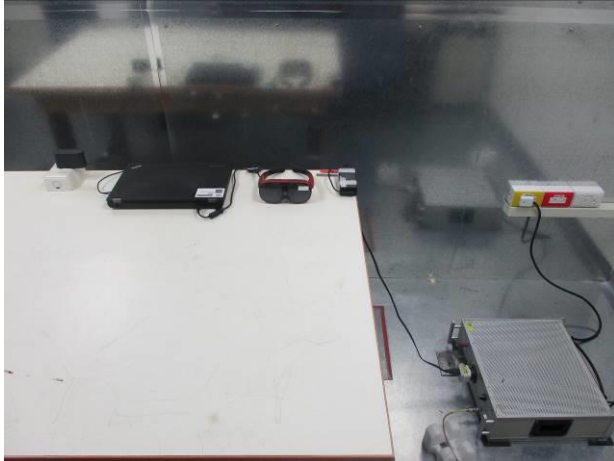
Part_15_247_WLAN_2.4G_Conduction_Setup
