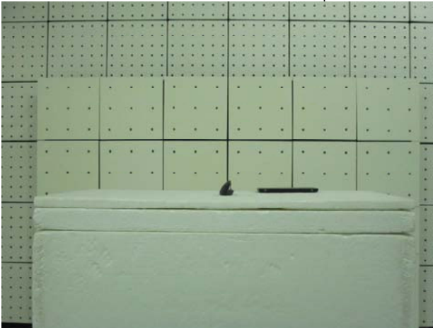
Part_15_249_SRD_Radiated_Setup
