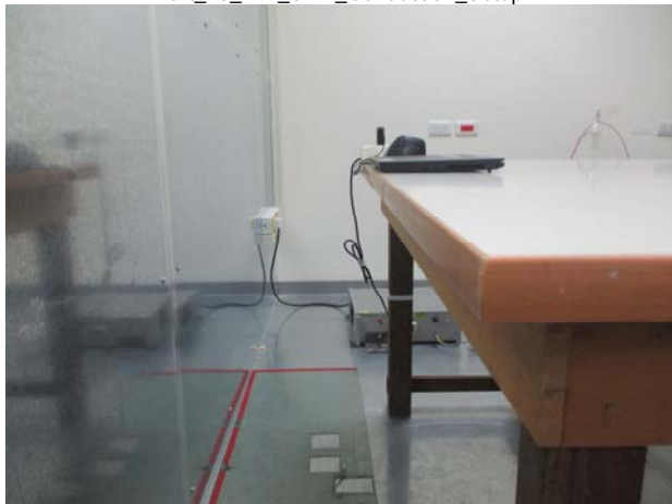
Part_15_249_SRD_Conduction_Setup
