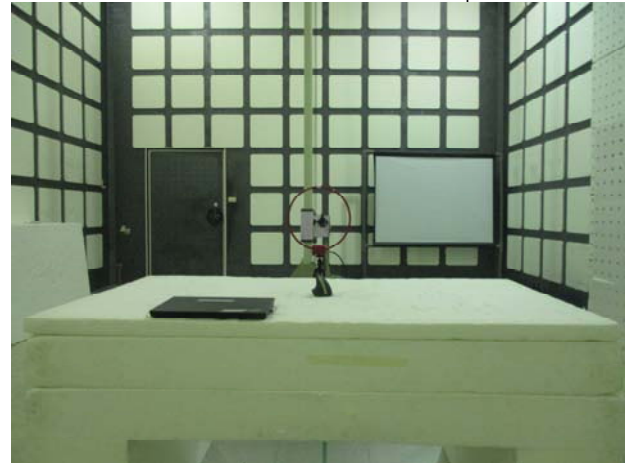
Part_15_249_SRD_Radiated_Setup
