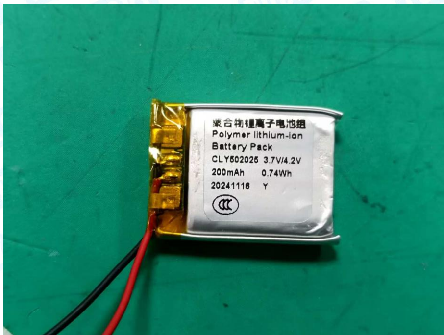
Photo 10 Battery Appearance
