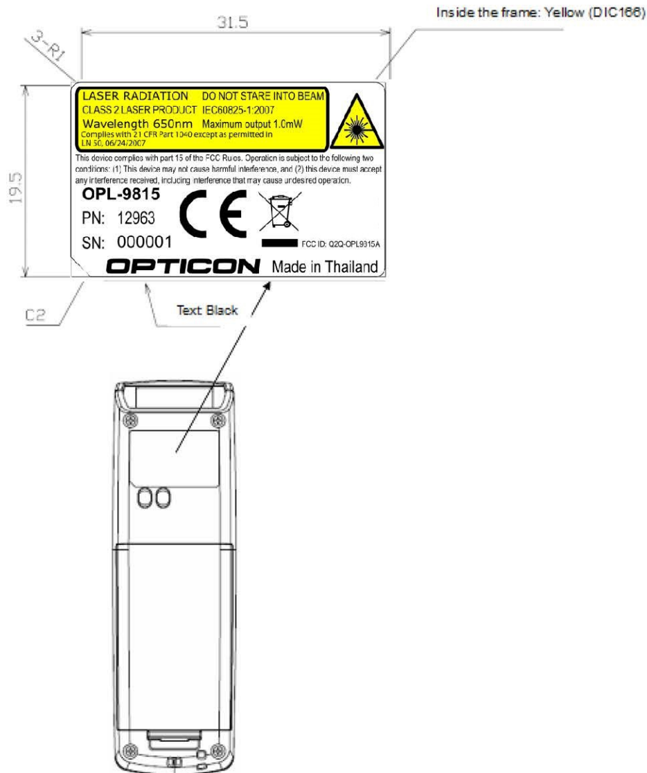
Figure 7: Name plate and serial number
