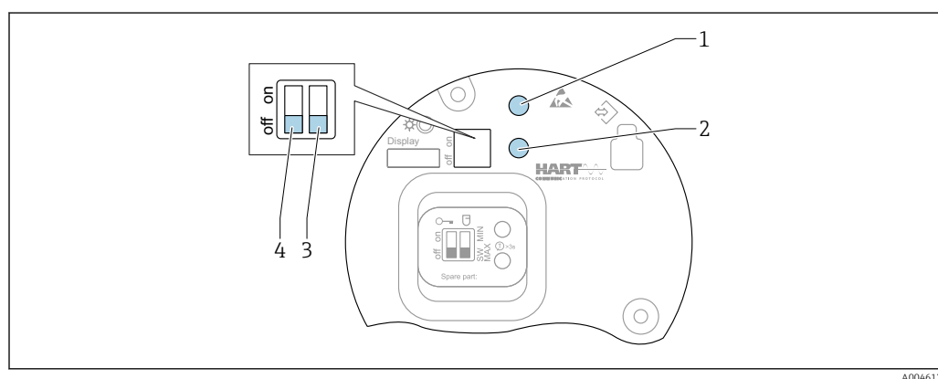
7 Operating keys and DIP switches on the HART electronic insert
