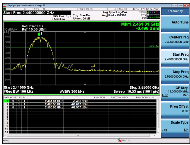
Right bandedge
