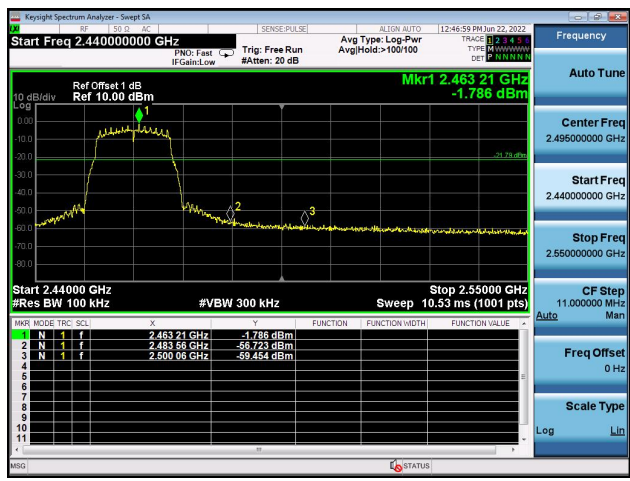
Right bandedge
