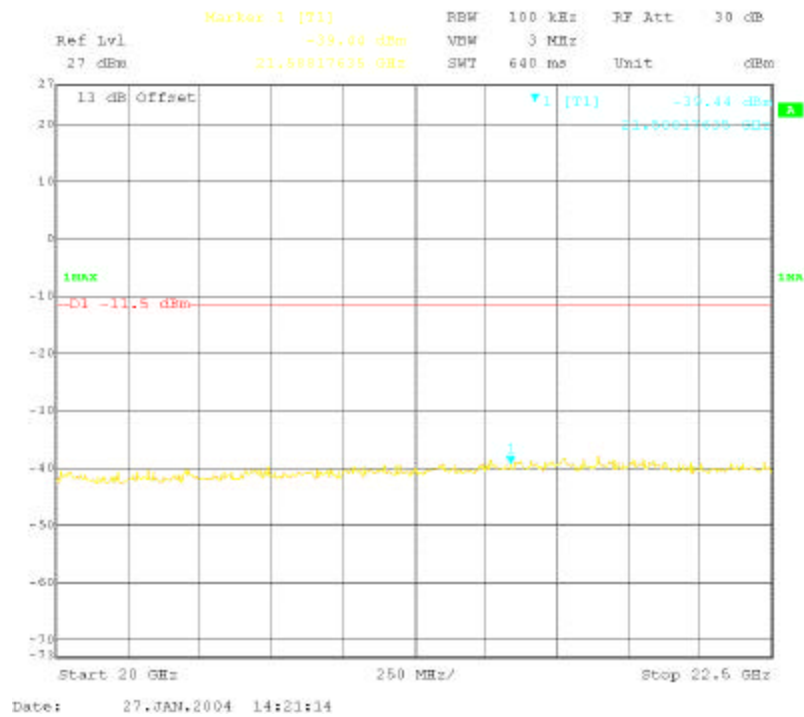
Conducted Spurious, 20 GHz – 22.5 GHz
