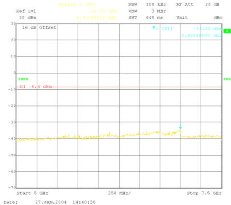
Conducted Spurious, 5 GHz – 7.5 GHz
