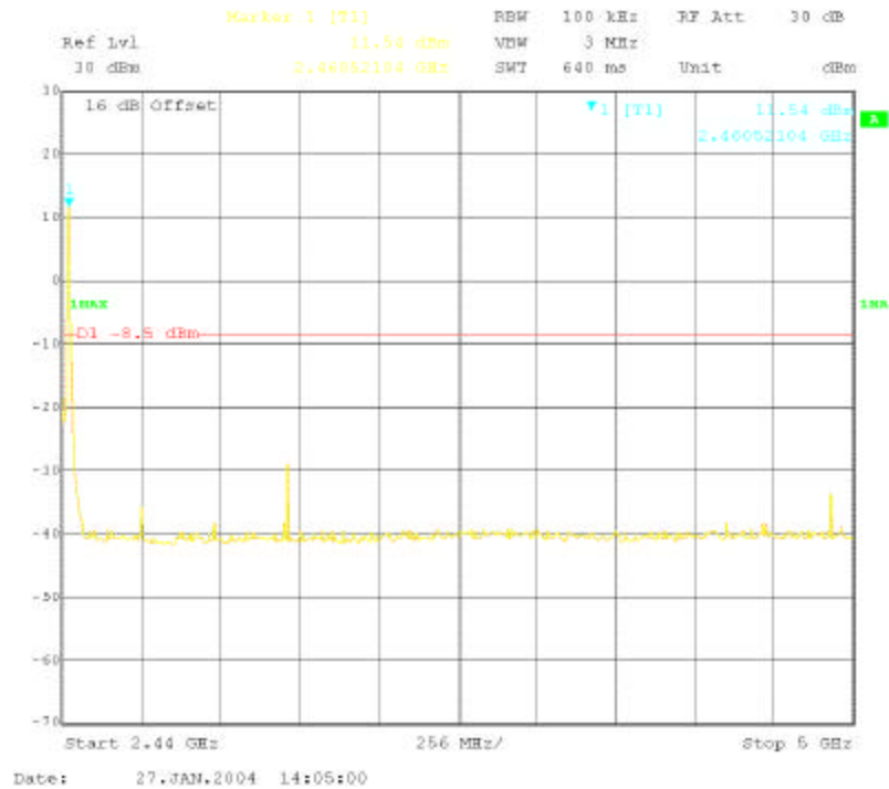
Conducted Spurious, 2.44 GHz – 5 GHz
