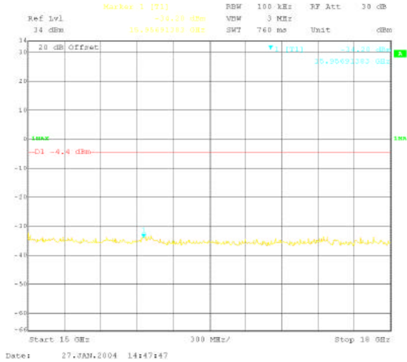
Conducted Spurious, 15 GHz – 18 GHz
