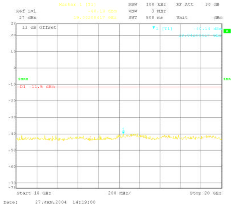
Conducted Spurious, 18 GHz – 20 GHz
