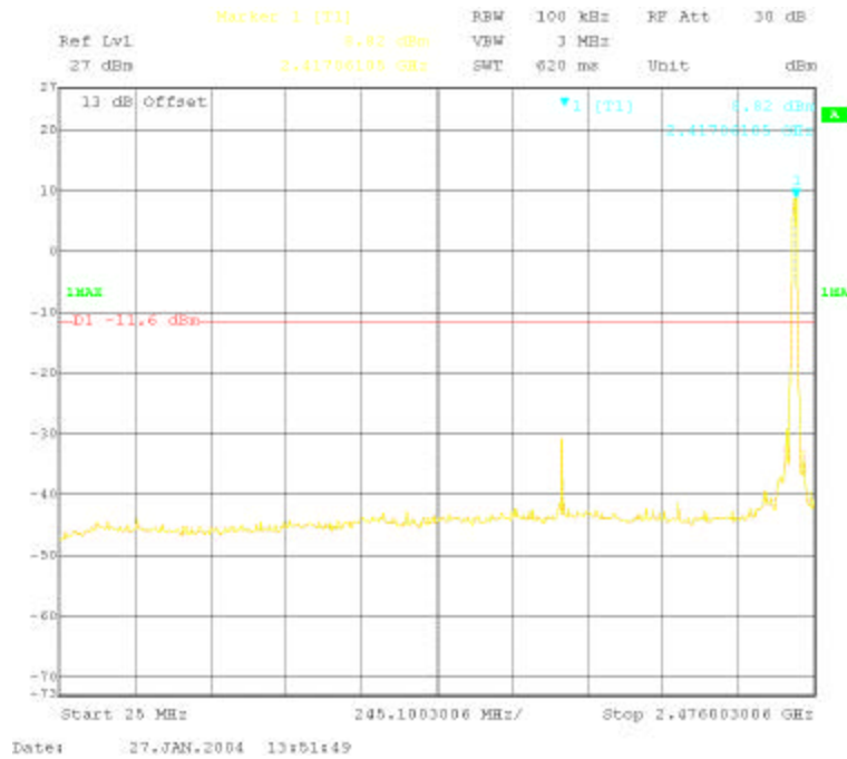
Conducted Spurious, 25 MHz – 2.47 GHz
