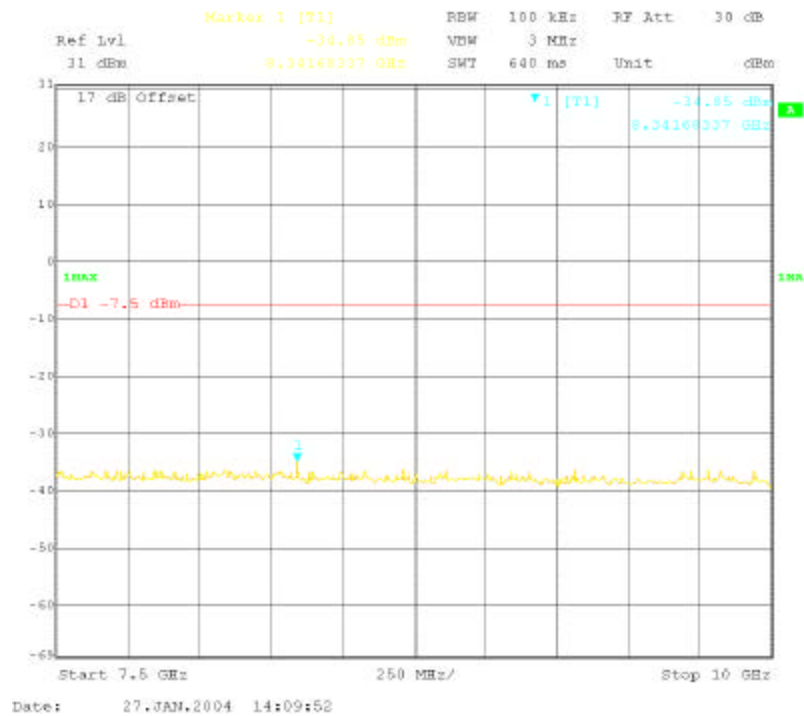
Conducted Spurious, 7.5 GHz – 10 GHz
