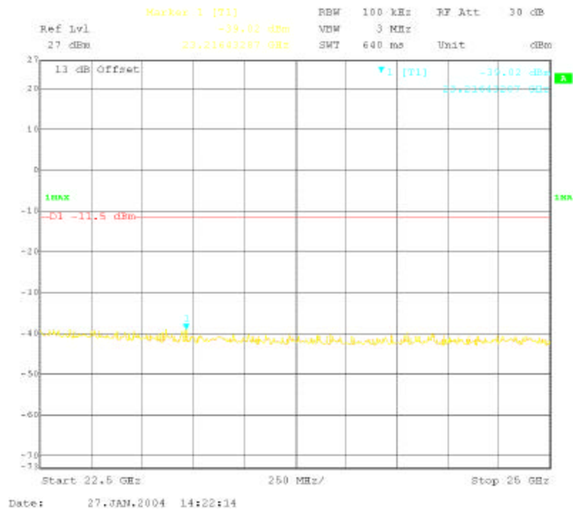
Conducted Spurious, 22.5 GHz – 25 GHz
