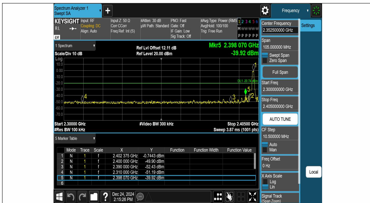
2.4GHz SRD 1M-Ant1-2402-PASS
