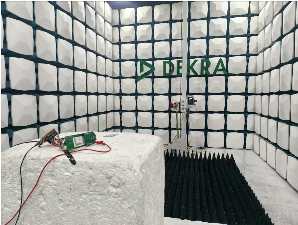
Description: Radiated emission(18-40GHz)
