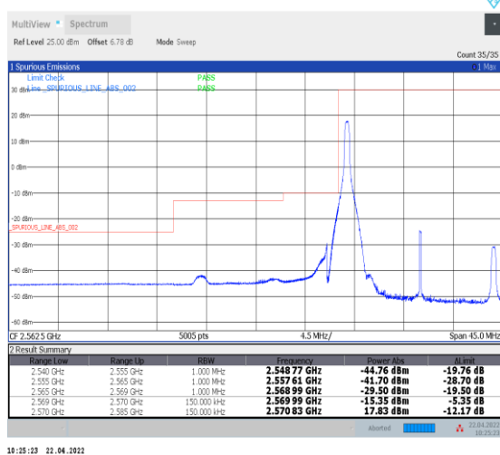
1-N38--30-15-L-4-CP-QPSK-Edge_1RB_Left-1@0-Ant0-PASS-see graph
