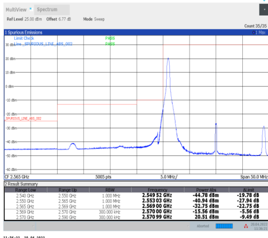
1-N38--30-20-L-4-CP-QPSK-Edge_1RB_Left-1@0-Ant0-PASS-see graph
