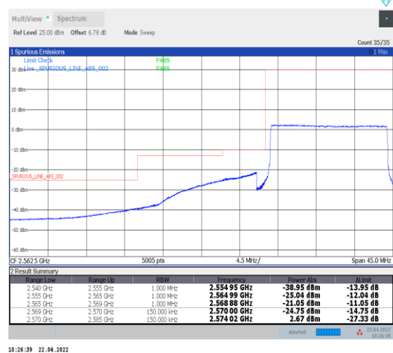
1-N38--30-15-L-6-CP-QPSK-Outer_Full-38@0-Ant0-PASS-see graph
