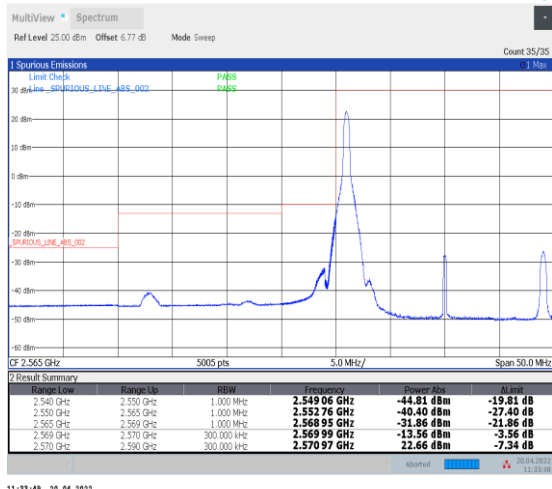
1-N38--30-20-L-1-DFT-PI2BPSK-Edge_1RB_Left-1@0-Ant0-PASS-see graph
