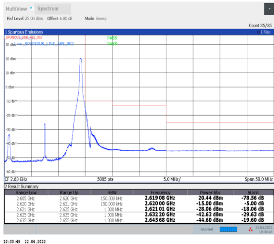
1-N38--30-15-H-2-DFT-PI2BPSK-Edge_1RB_Right-1@37-Ant0-PASS-see graph
