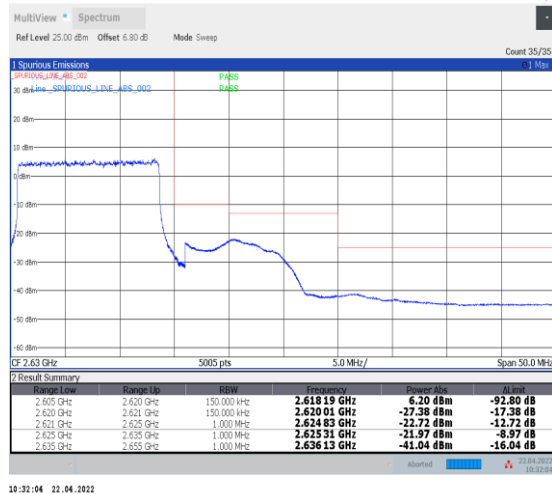
1-N38--30-15-H-3-DFT-PI2BPSK-Outer_Full-36@0-Ant0-PASS-see graph
