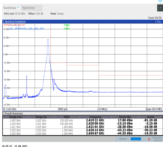
1-N38--30-15-H-5-CP-QPSK-Edge_1RB_Right-1@37-Ant0-PASS-see graph
