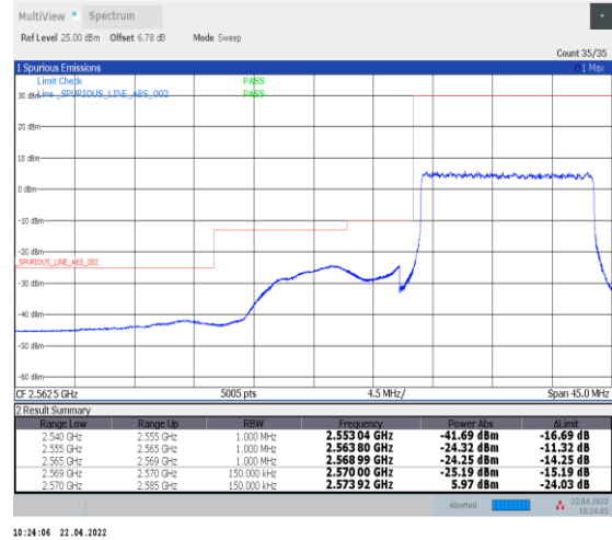
1-N38--30-15-L-3-DFT-PI2BPSK-Outer_Full-36@0-Ant0-PASS-see graph
