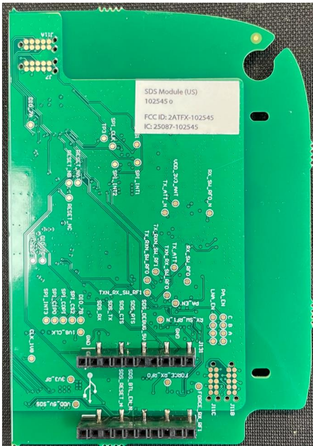
Figure 3: Picture of bottom side of part 102545 - SDS Module (US).
