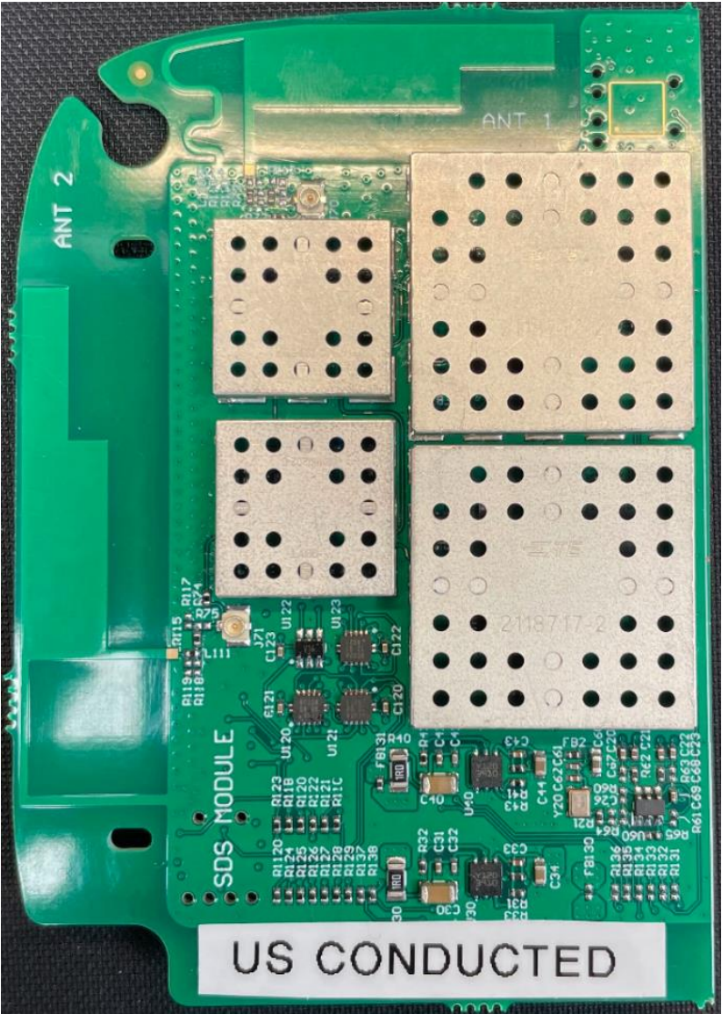
Figure 1: Picture of component side of part 102545 - SDS Module (US)
