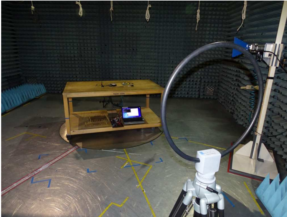
Photo 1: Test setup for radiated measurements (below 30 MHz)
