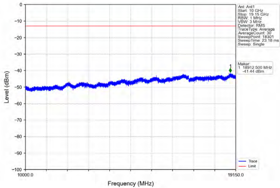
Band25 15MHz 16QAM HCH 1907.5MHz RB 1 0 NTV
